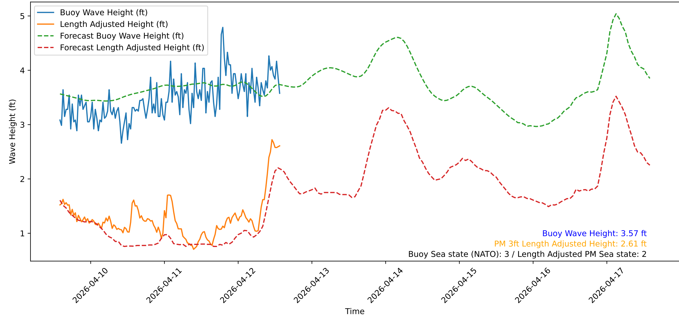
Wave Heights over Time for Oceanside Harbor at 2026-04-12 14:10:31
