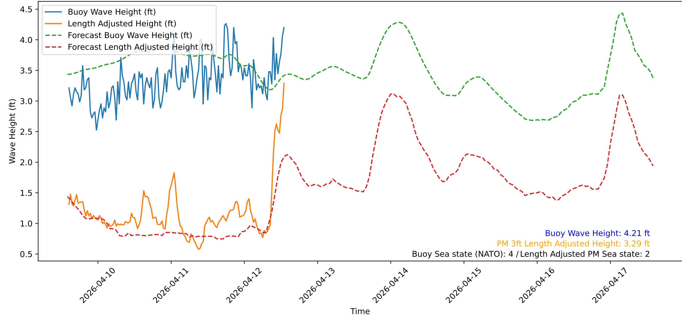
Wave Heights over Time for Red Beach at 2026-04-12 14:10:50
