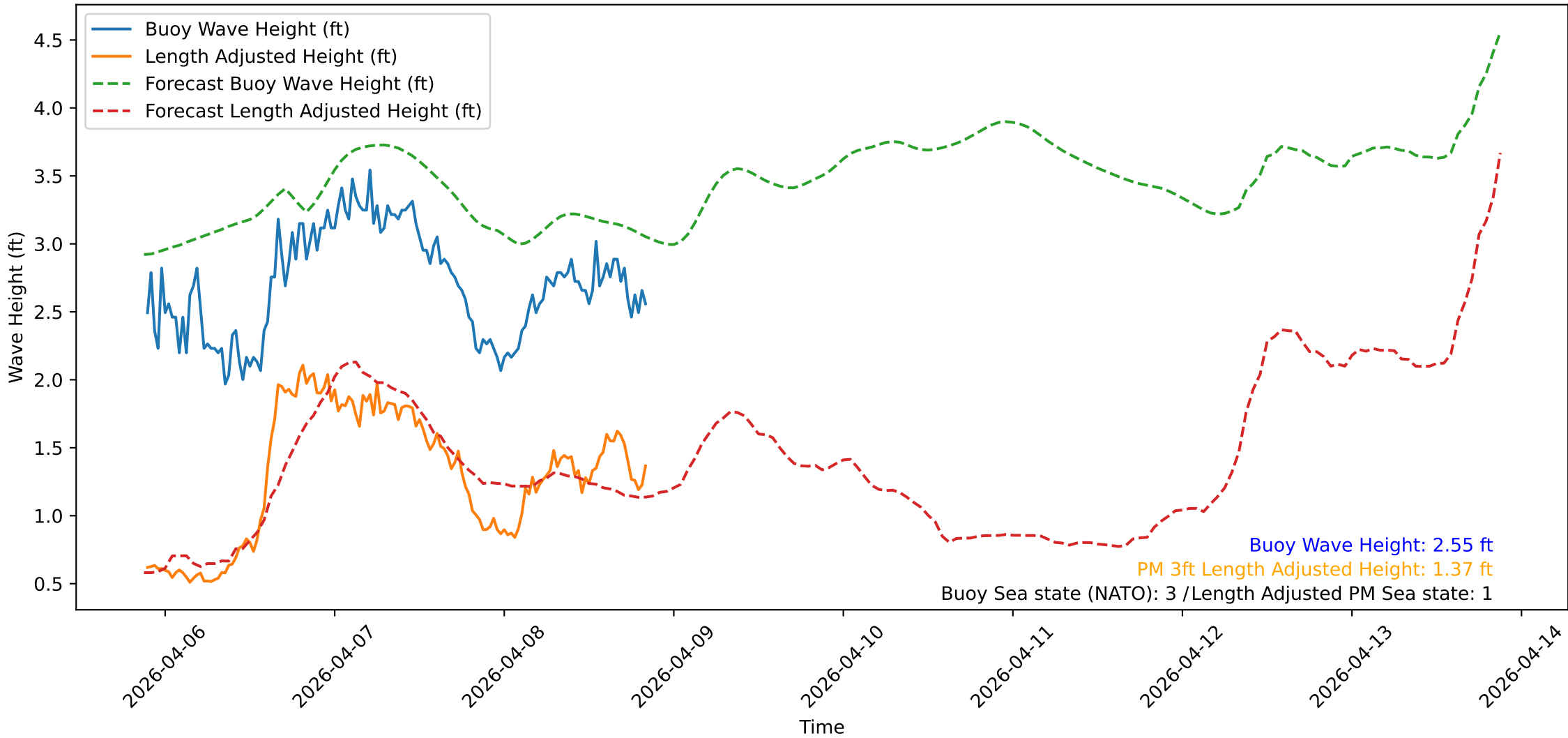
Wave Heights over Time for Red Beach at 2026-04-08 21:00:48
