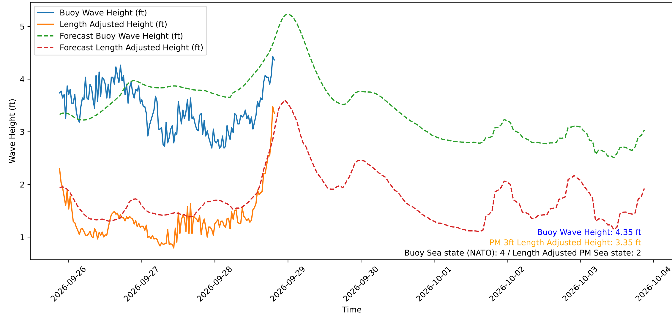
Wave Heights over Time for Green Beach at 2026-09-28 20:31:14
