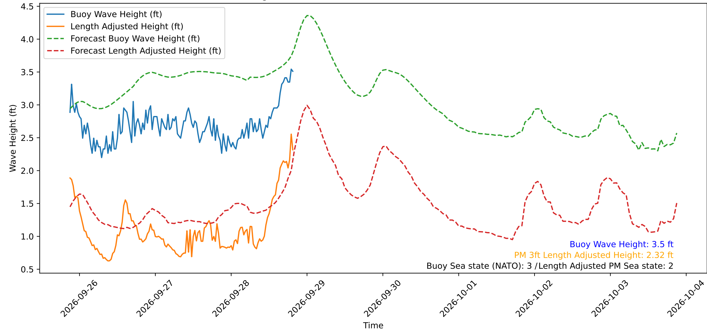
Wave Heights over Time for Red Beach at 2026-09-28 20:30:50
