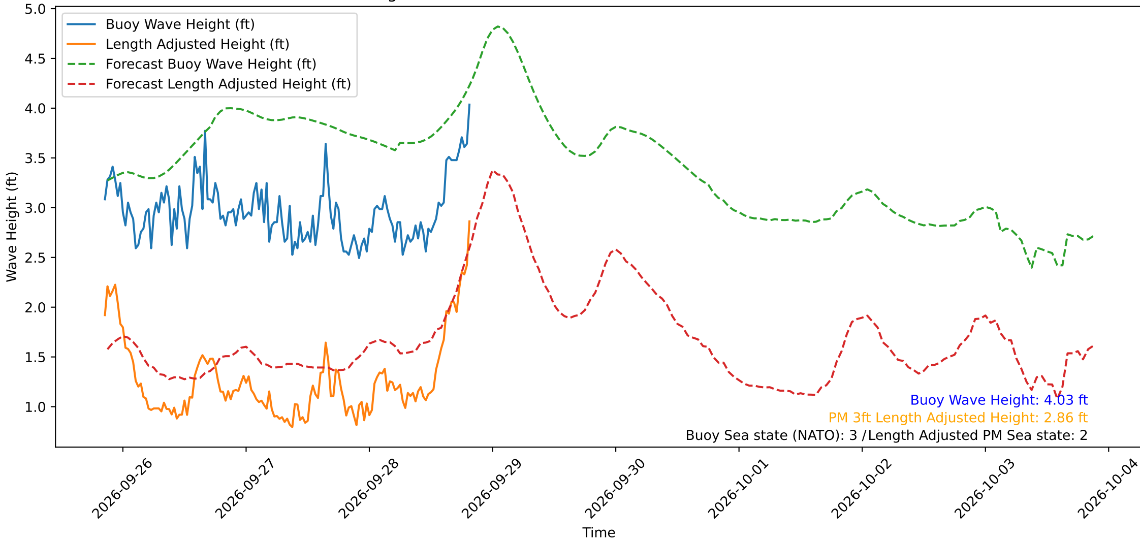
Wave Heights over Time for Oceanside Harbor at 2026-09-28 20:30:29
