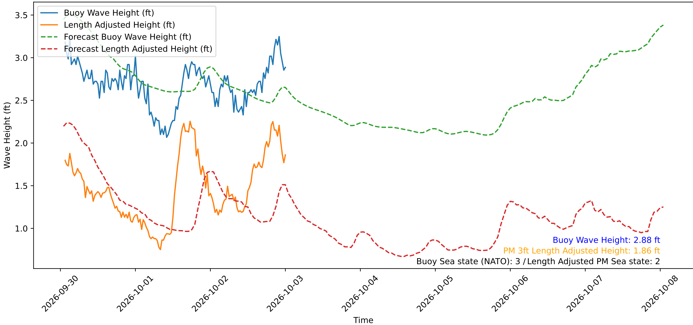
Wave Heights over Time for Red Beach at 2026-10-03 01:00:49
