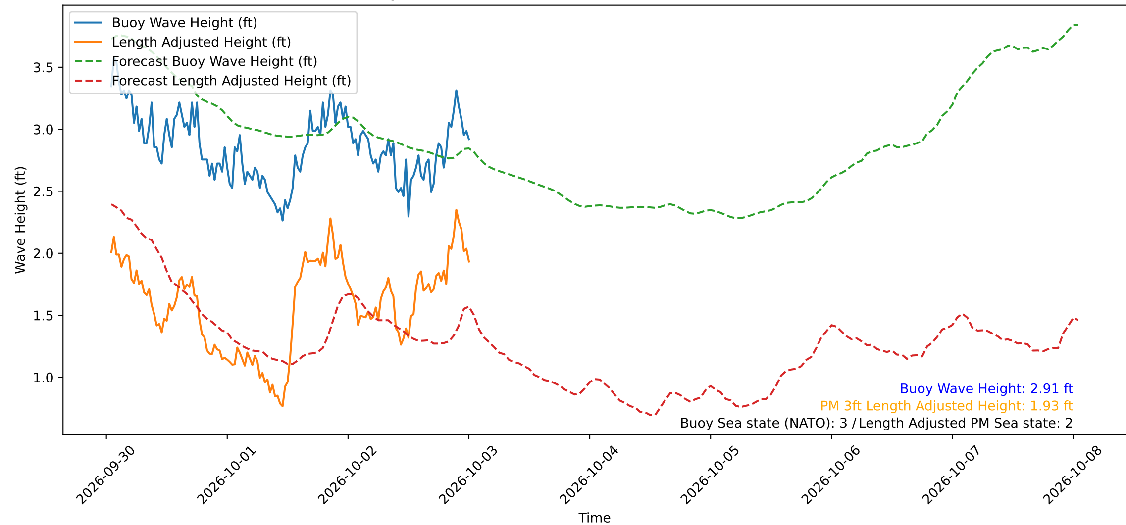
Wave Heights over Time for Oceanside Harbor at 2026-10-03 01:00:30
