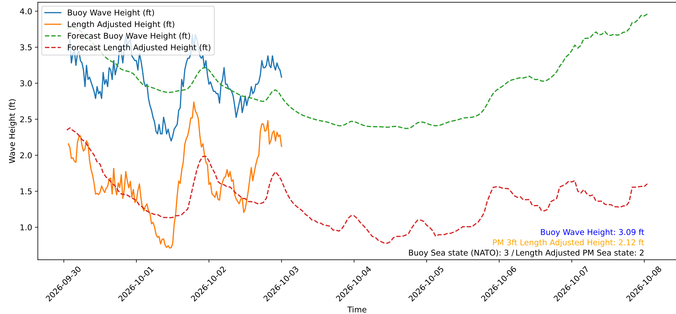
Wave Heights over Time for Green Beach at 2026-10-03 01:01:11
