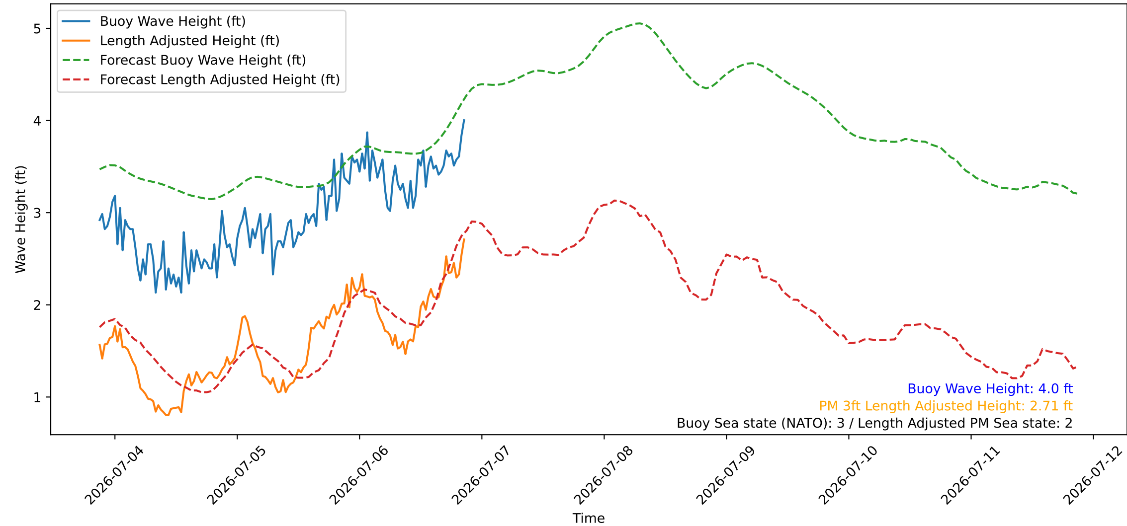
Wave Heights over Time for Oceanside Harbor at 2026-07-06 21:10:27
