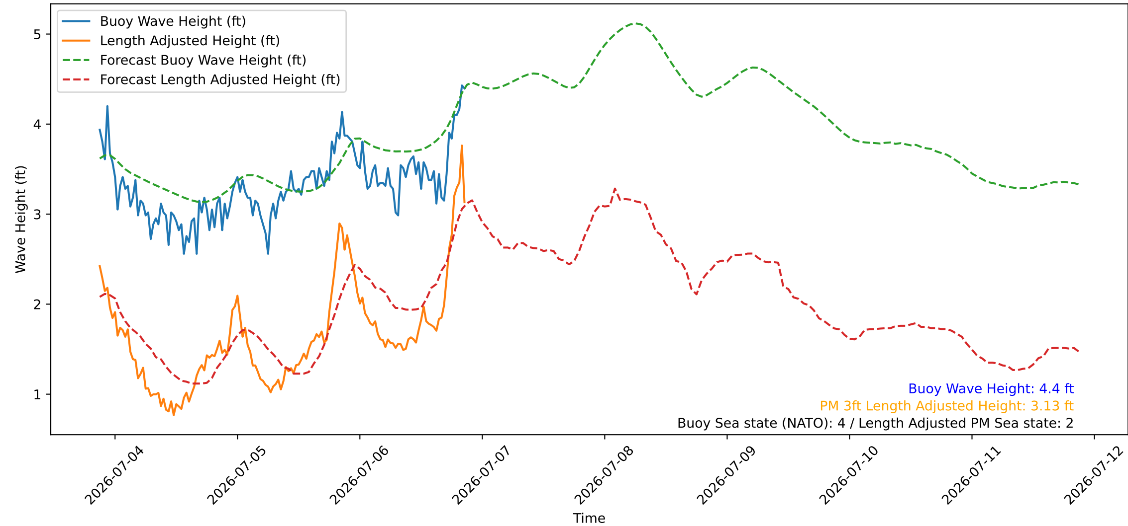
Wave Heights over Time for Green Beach at 2026-07-06 21:11:08
