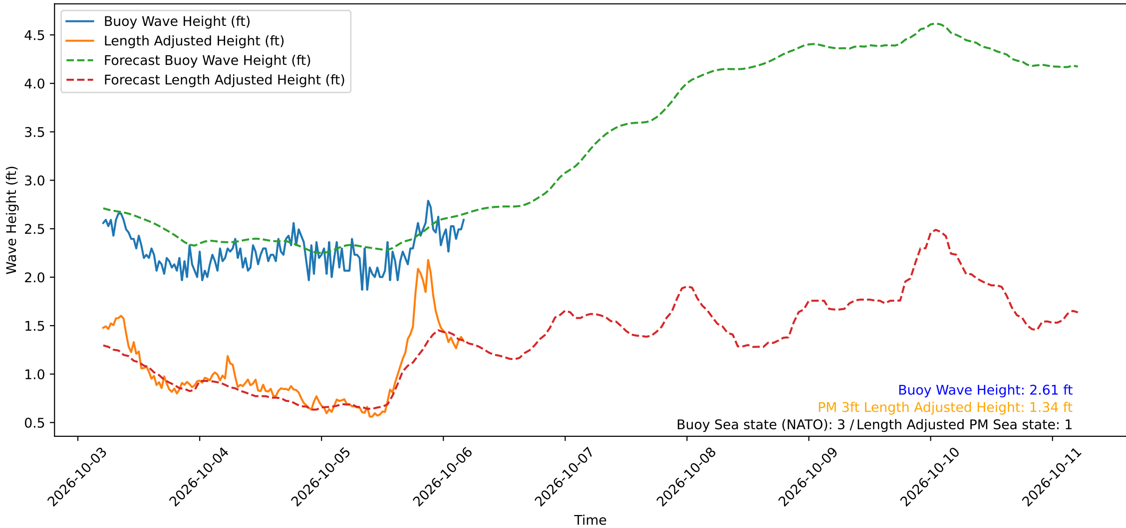
Wave Heights over Time for Oceanside Harbor at 2026-10-06 05:00:29
