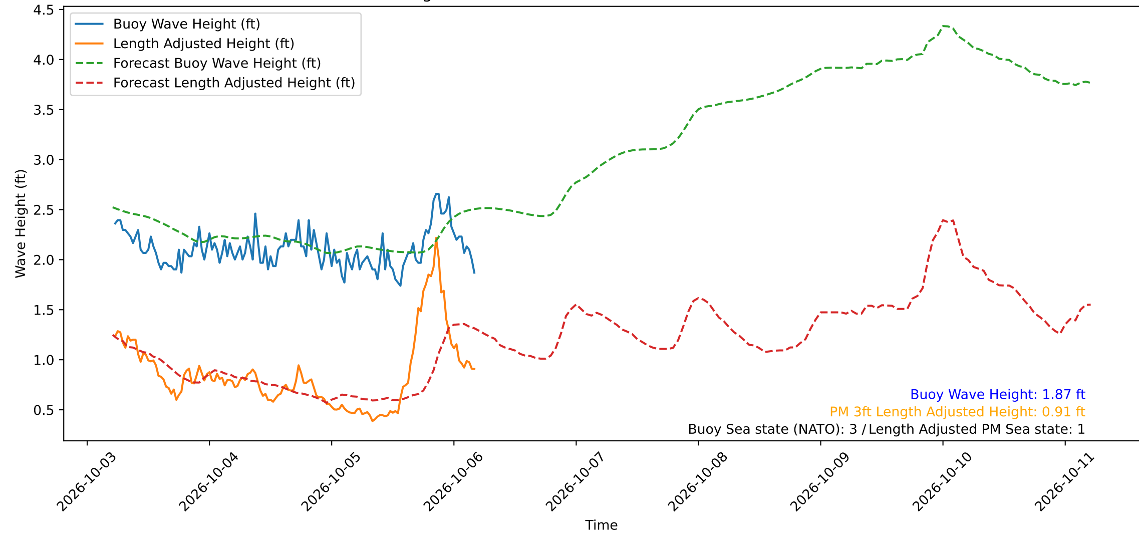
Wave Heights over Time for Red Beach at 2026-10-06 05:00:49
