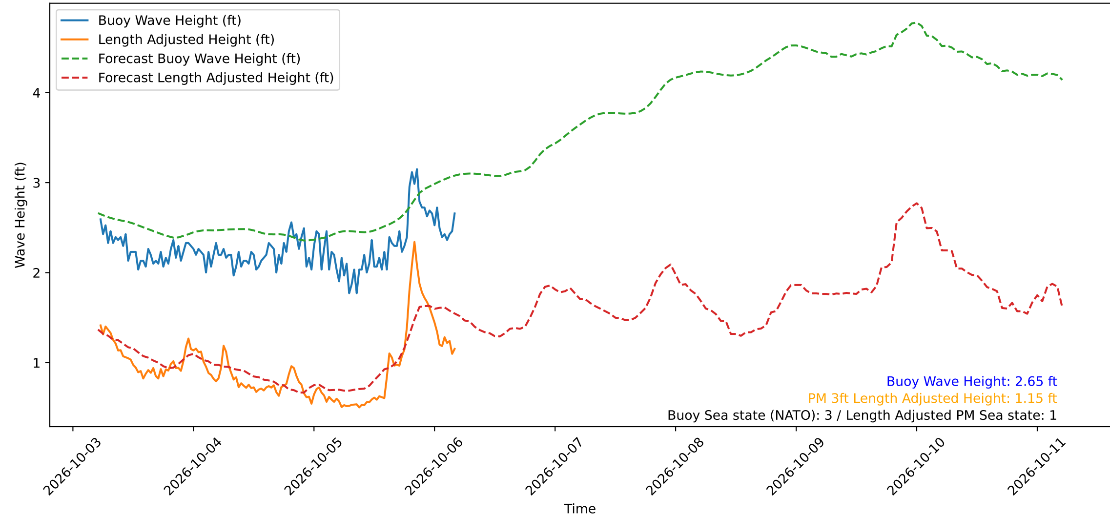
Wave Heights over Time for Green Beach at 2026-10-06 05:01:11
