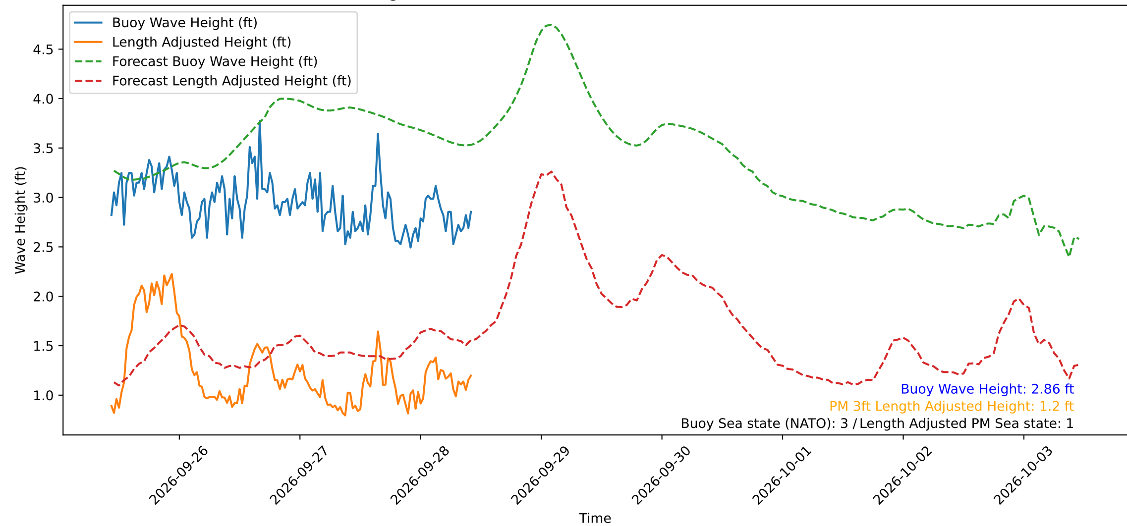
Wave Heights over Time for Oceanside Harbor at 2026-09-28 10:40:30
