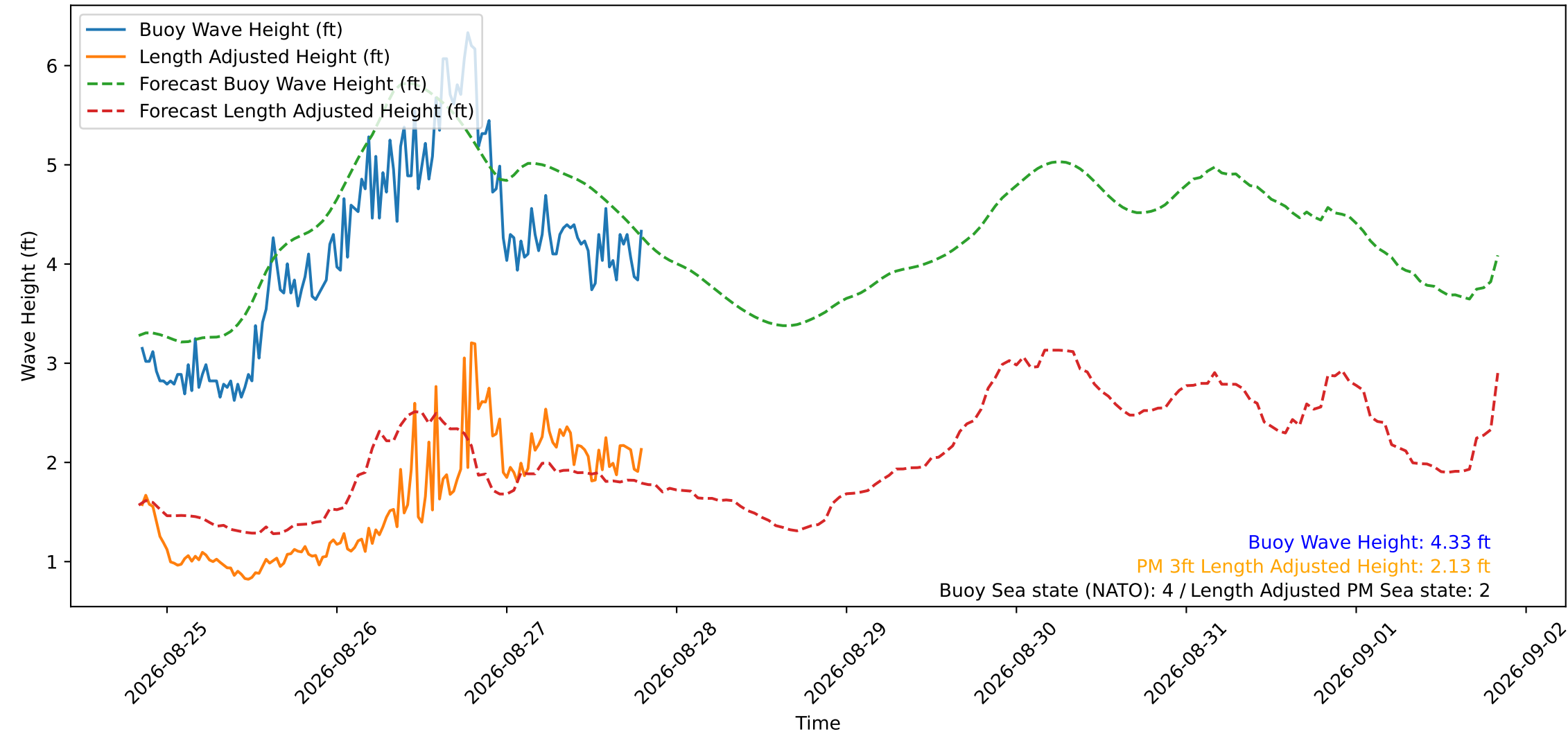
Wave Heights over Time for Green Beach at 2026-08-27 20:01:12
