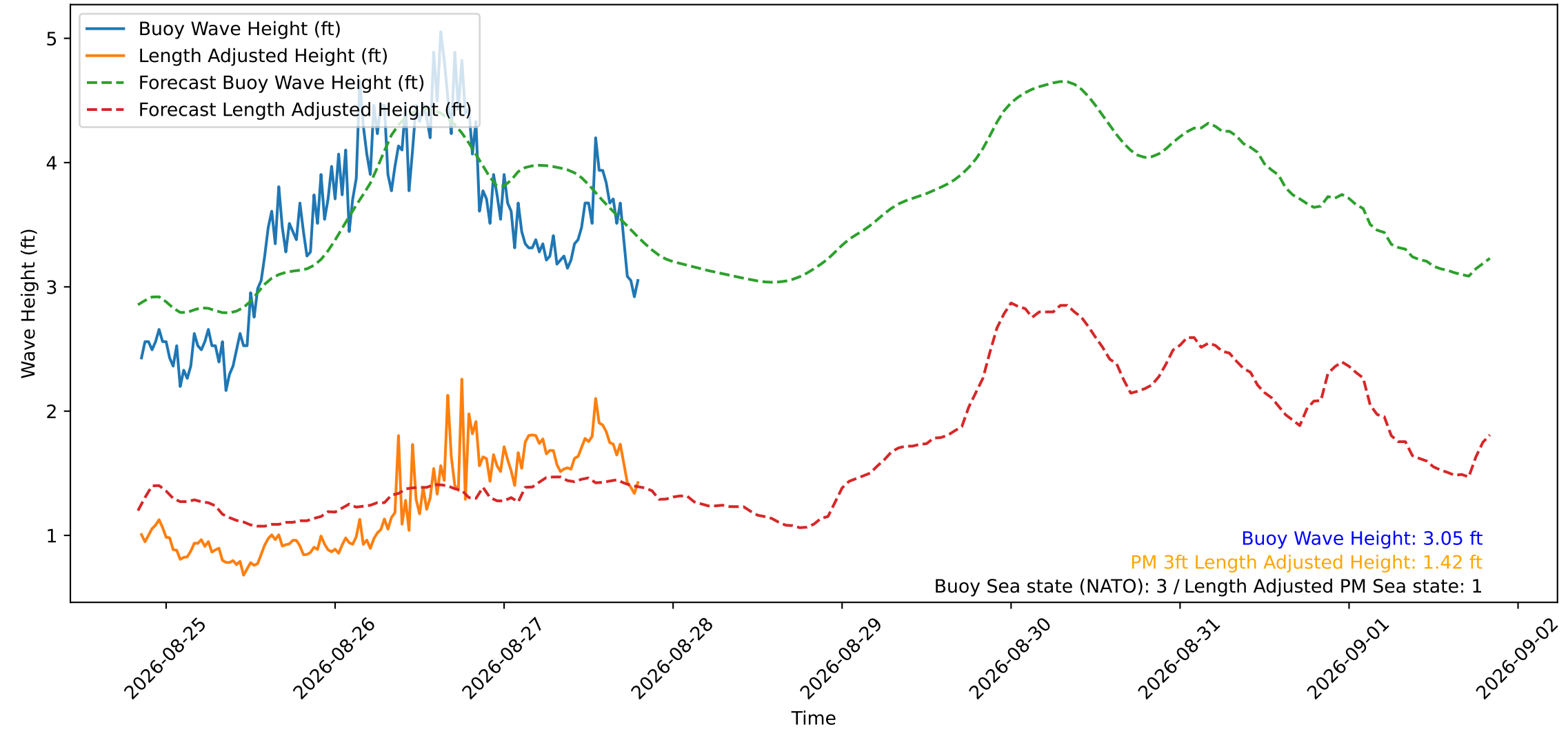
Wave Heights over Time for Red Beach at 2026-08-27 20:00:49
