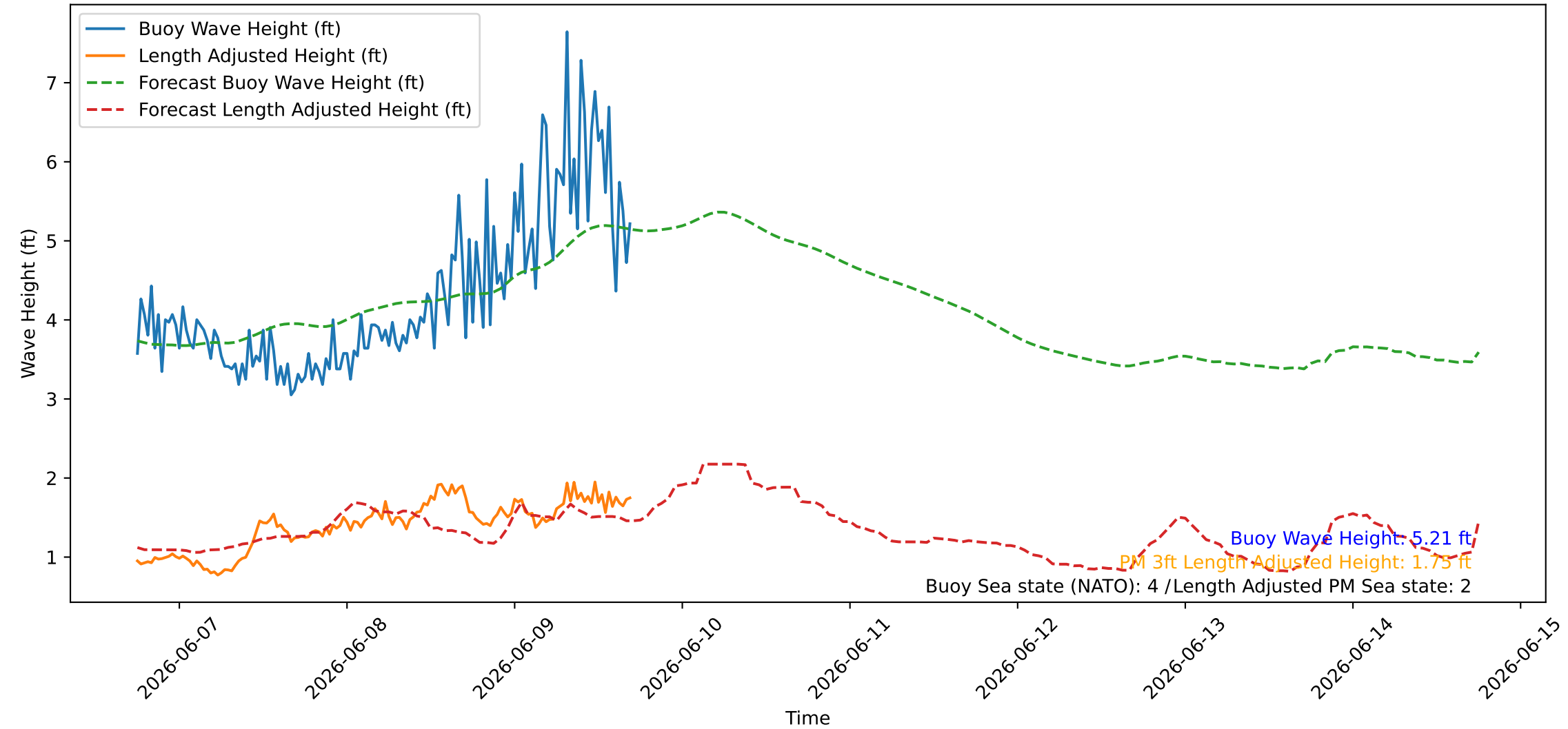
Wave Heights over Time for Red Beach at 2026-06-09 17:30:46
