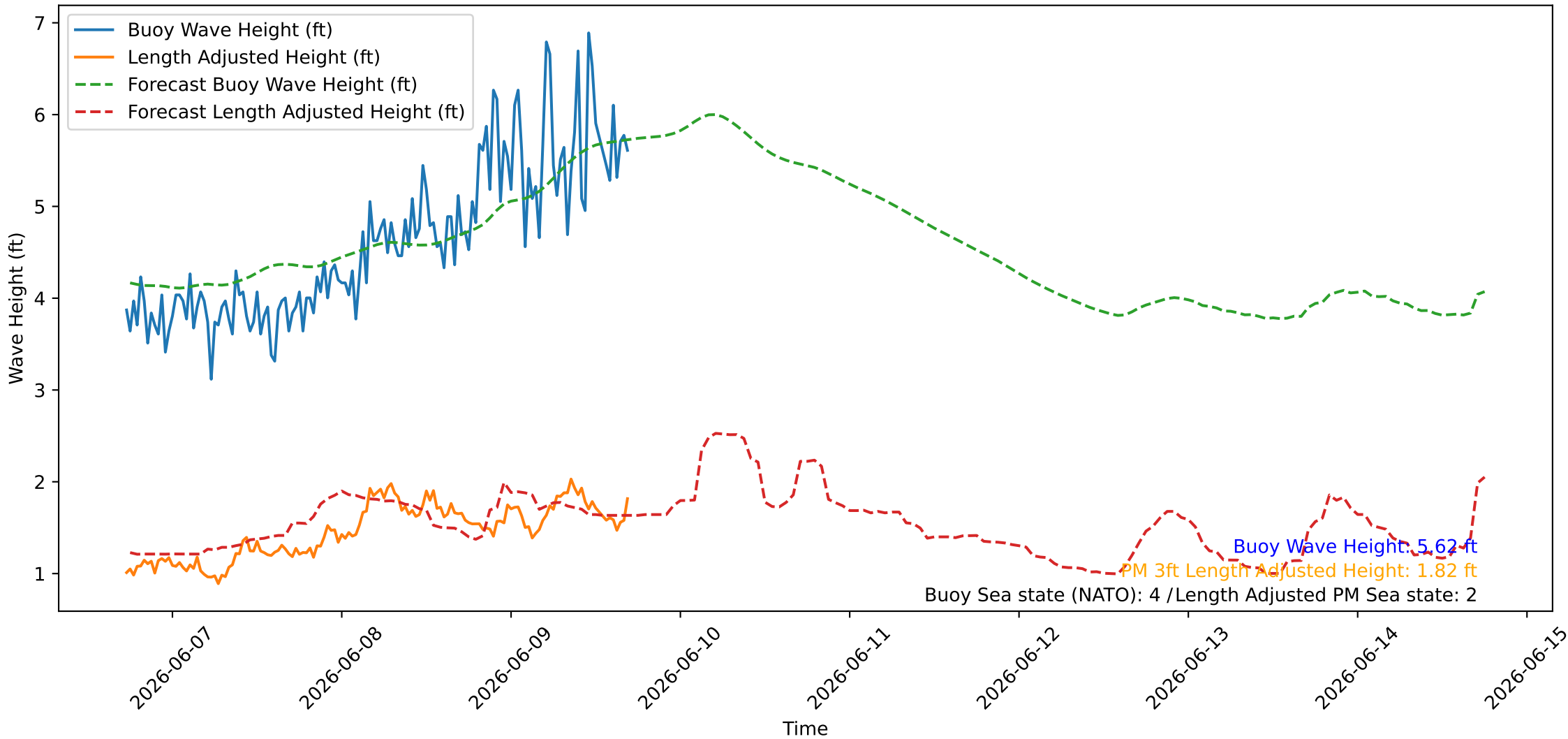
Wave Heights over Time for Green Beach at 2026-06-09 17:31:08
