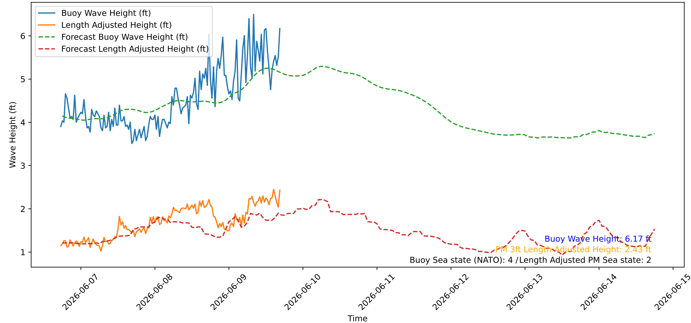
Wave Heights over Time for Oceanside Harbor at 2026-06-09 17:30:27
