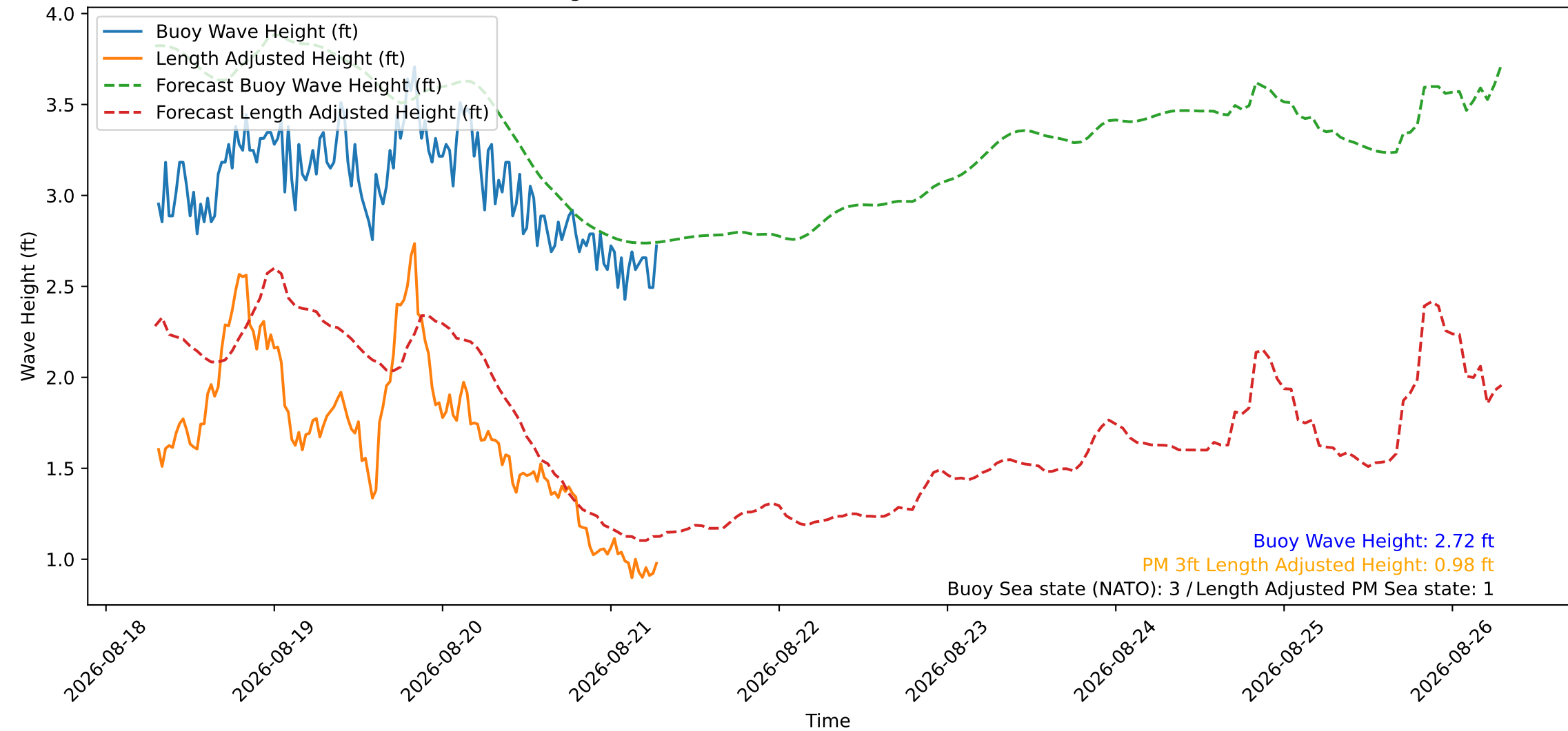
Wave Heights over Time for Green Beach at 2026-08-21 07:11:10
