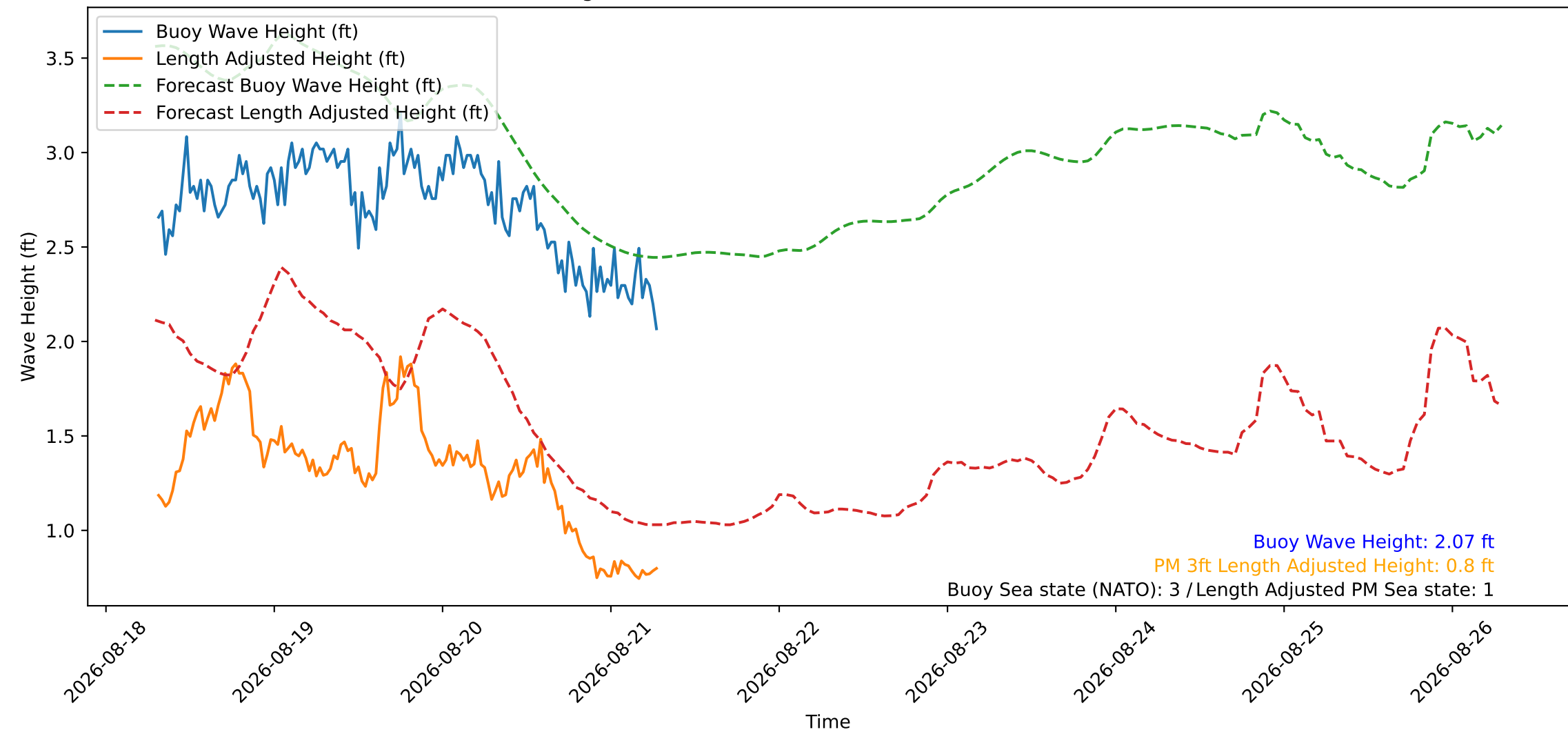
Wave Heights over Time for Red Beach at 2026-08-21 07:10:47
