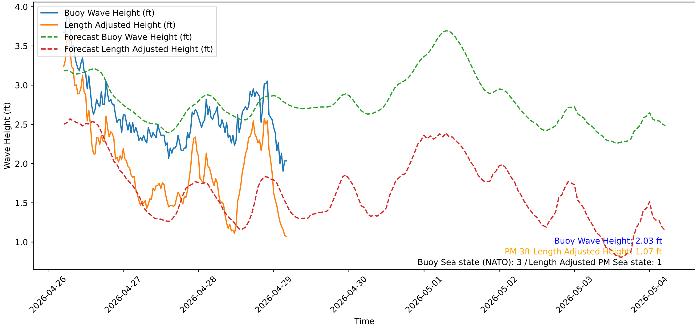
Wave Heights over Time for Oceanside Harbor at 2026-04-29 05:00:31
