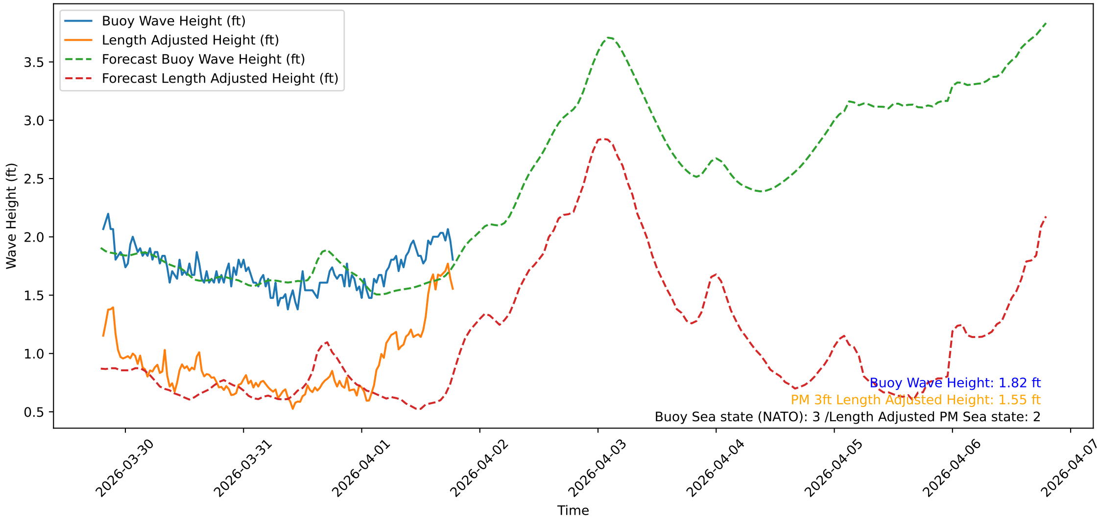
Wave Heights over Time for Red Beach at 2026-04-01 19:20:47
