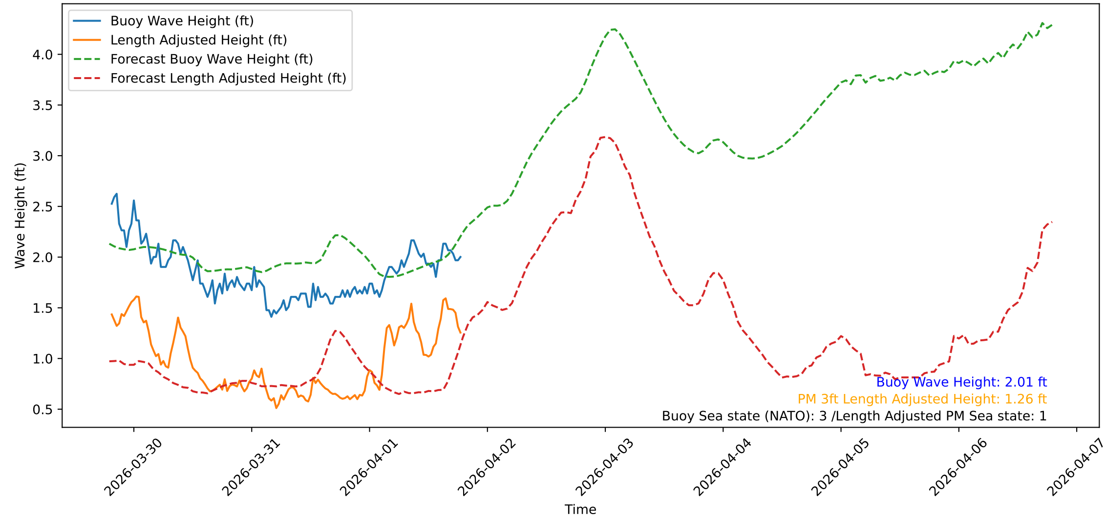
Wave Heights over Time for Green Beach at 2026-04-01 19:21:10
