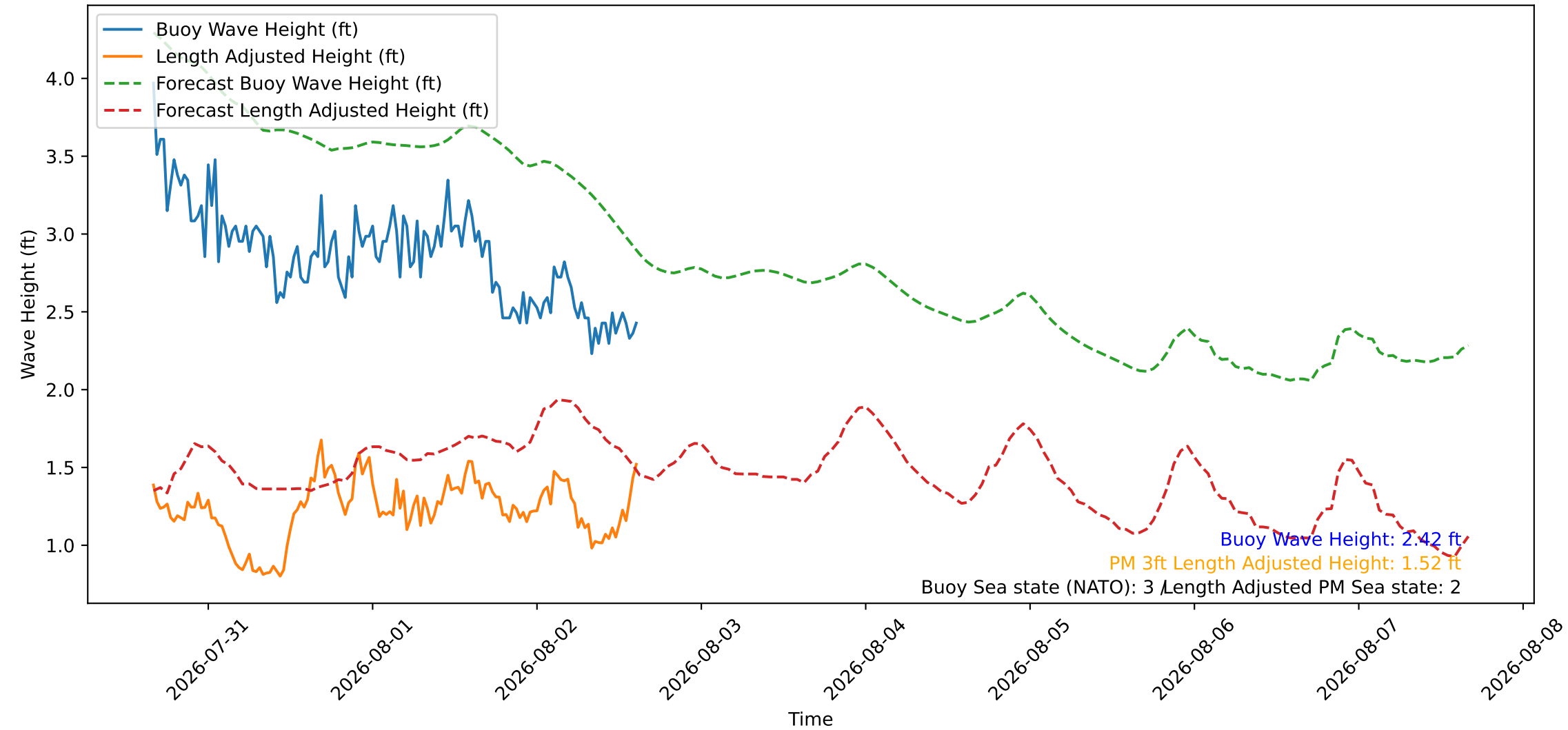
Wave Heights over Time for Red Beach at 2026-08-02 15:30:45
