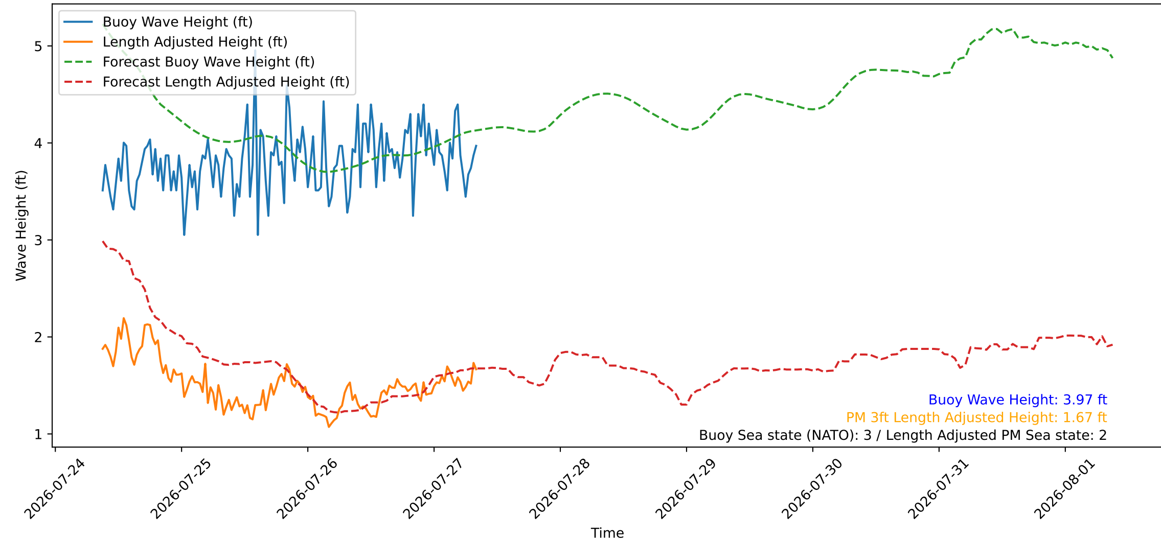
Wave Heights over Time for Oceanside Harbor at 2026-07-27 08:50:34
