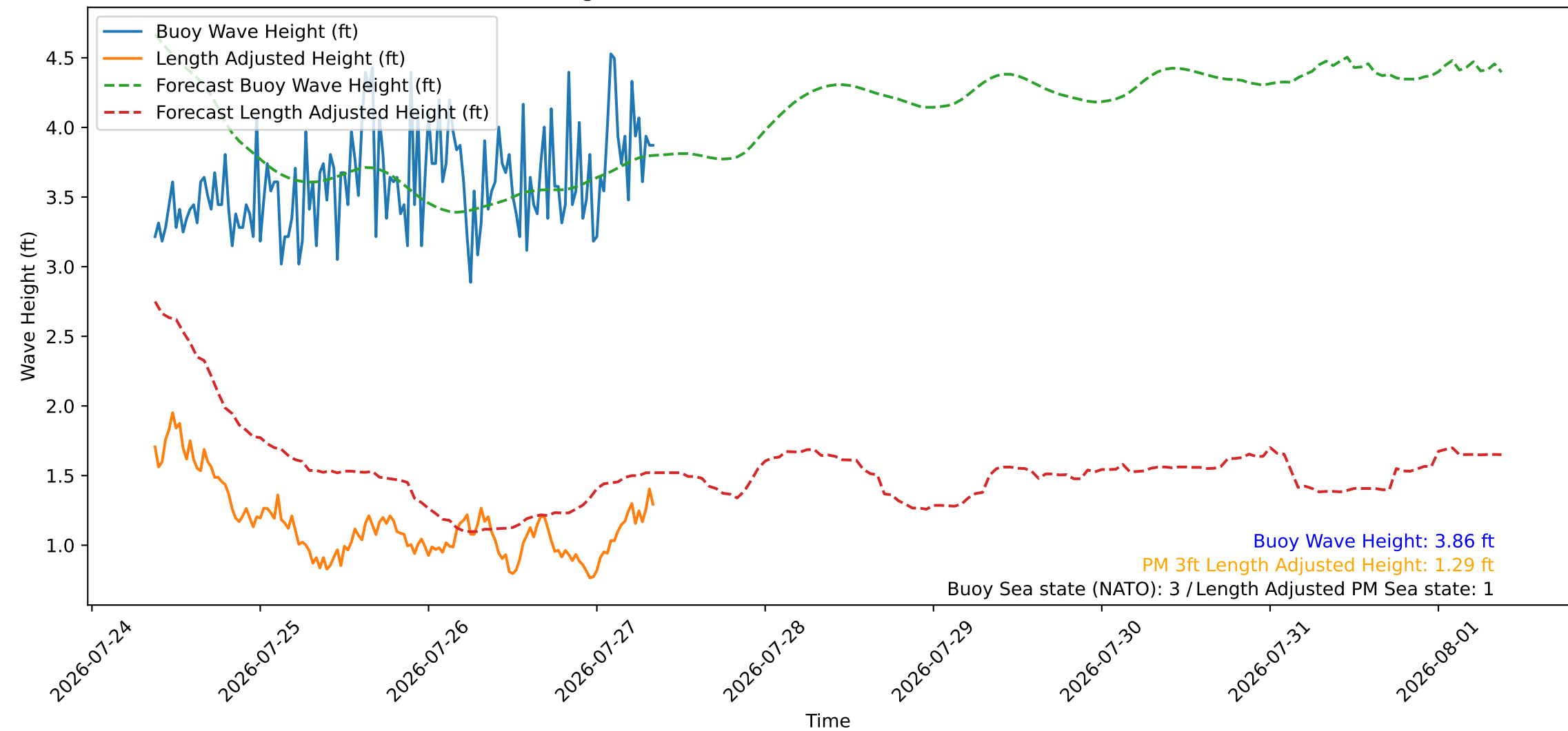
Wave Heights over Time for Red Beach at 2026-07-27 08:50:55
