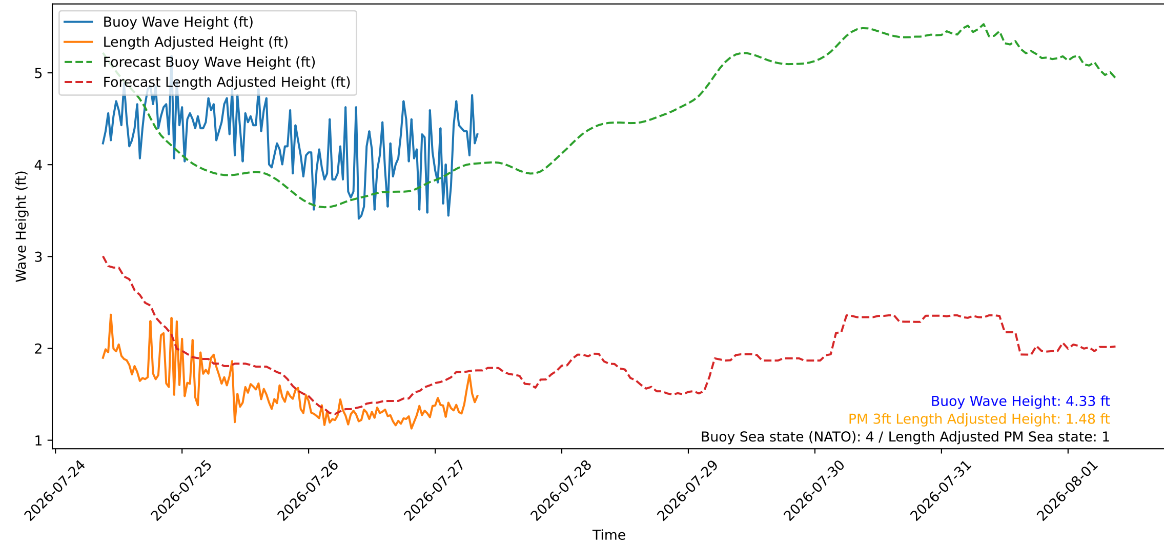
Wave Heights over Time for Green Beach at 2026-07-27 08:51:19
