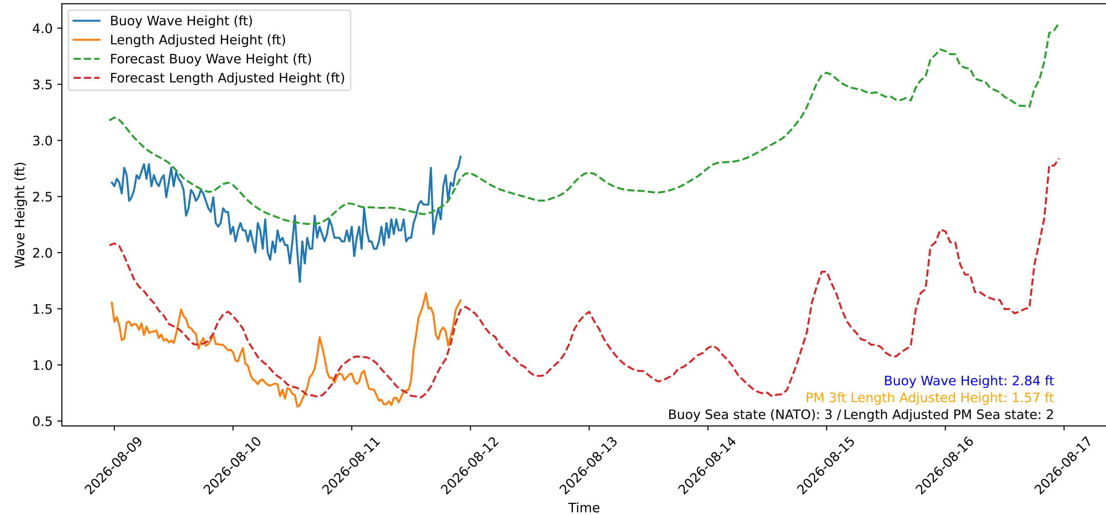
Wave Heights over Time for Red Beach at 2026-08-11 23:10:46
