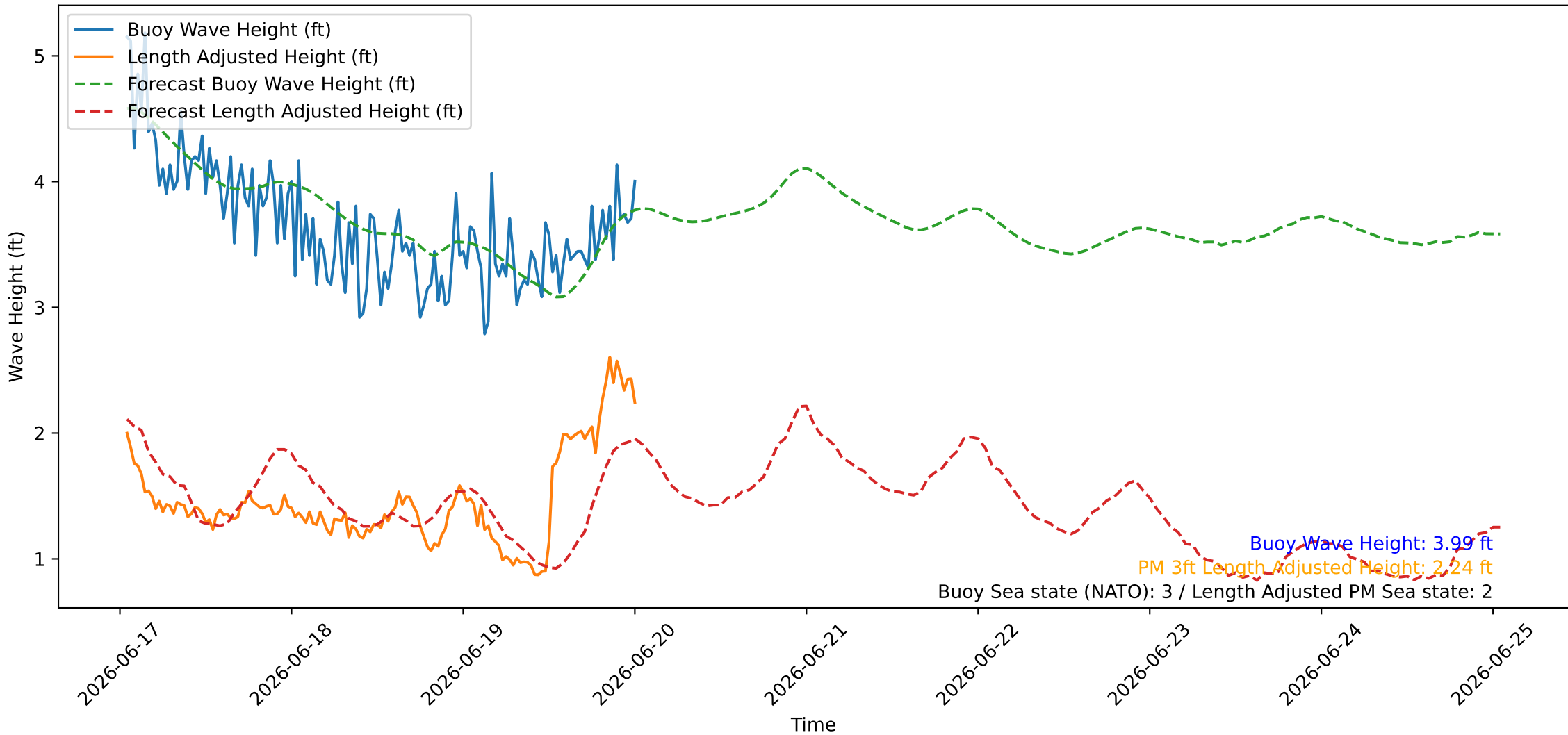
Wave Heights over Time for Oceanside Harbor at 2026-06-20 00:50:26
