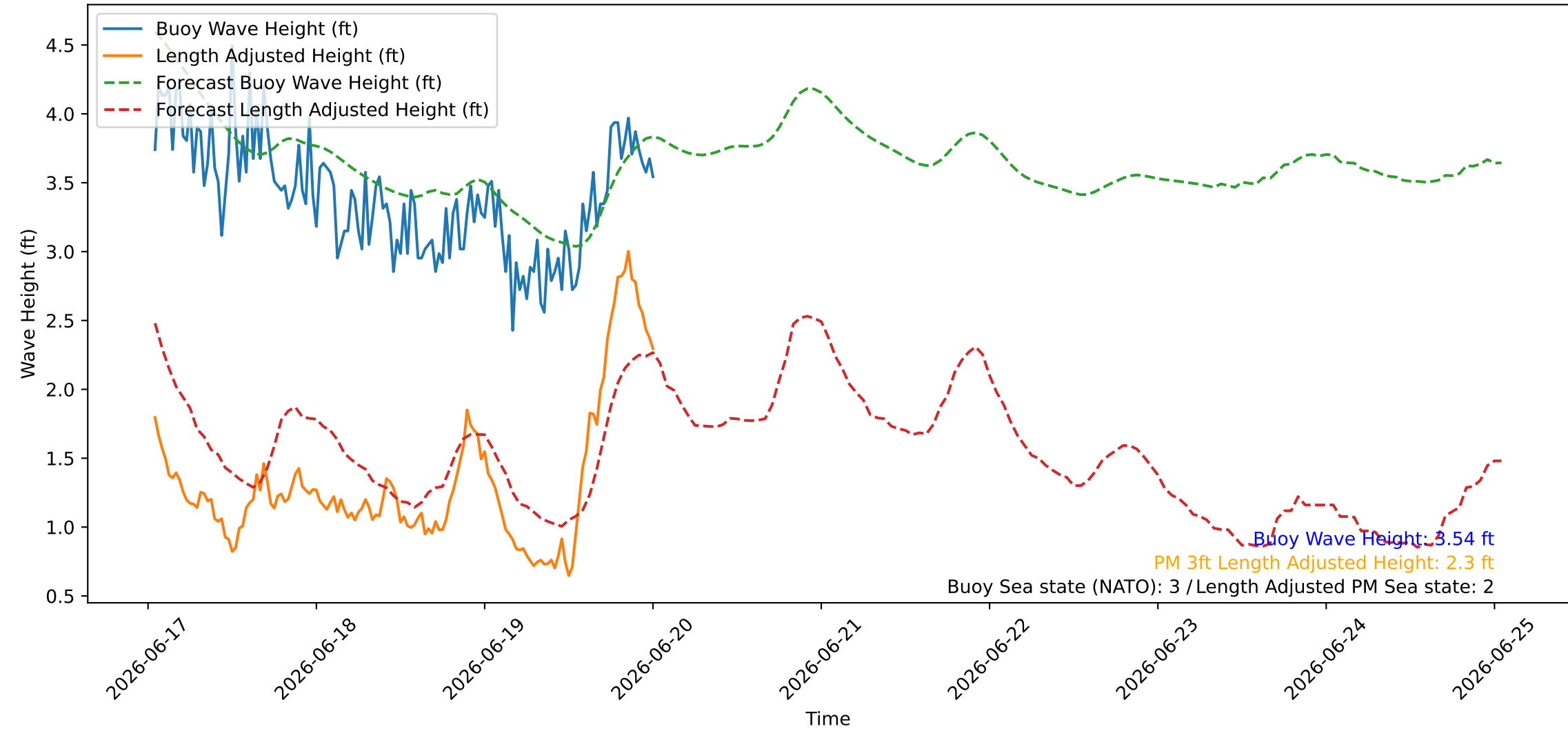
Wave Heights over Time for Green Beach at 2026-06-20 00:51:08
