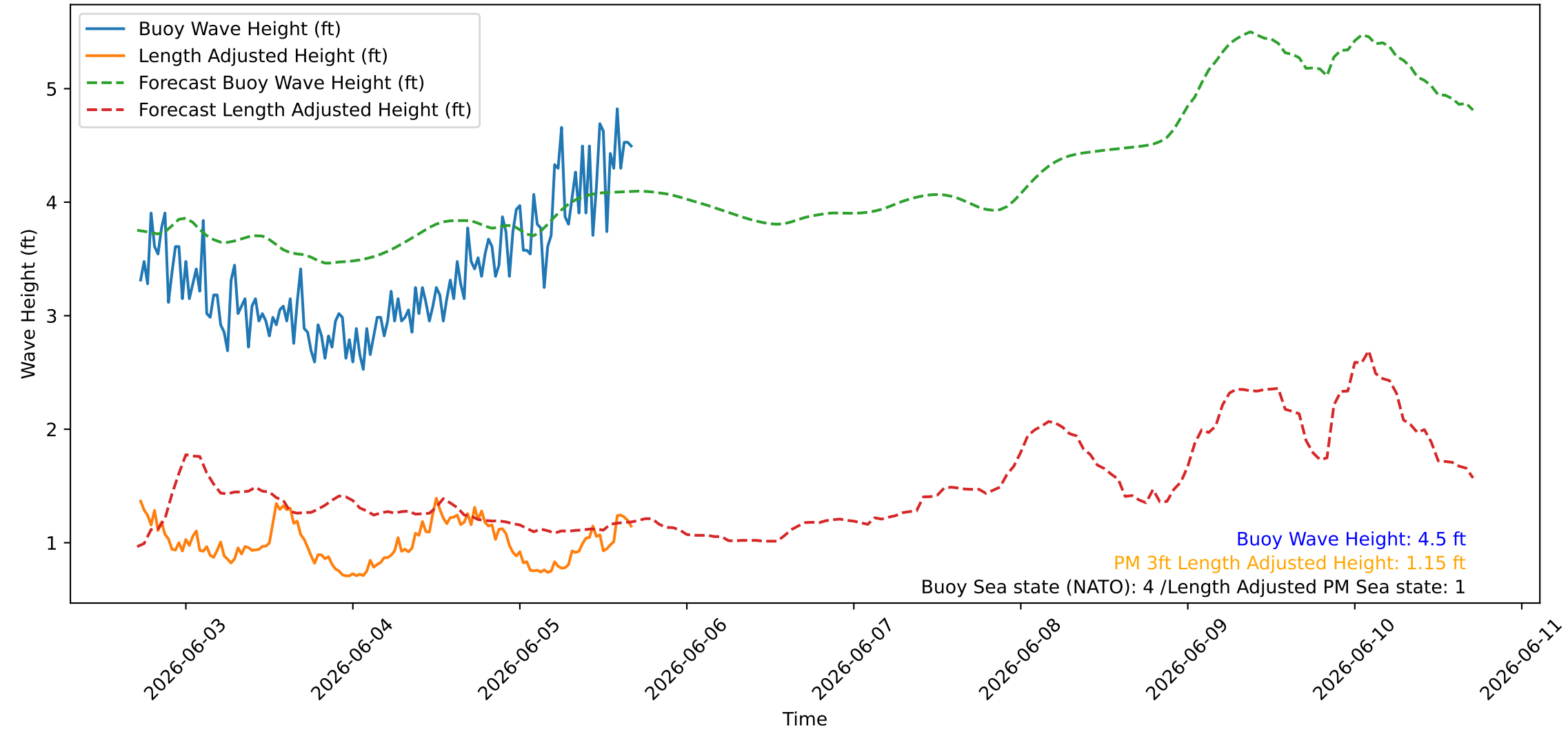
Wave Heights over Time for Red Beach at 2026-06-05 17:00:46
