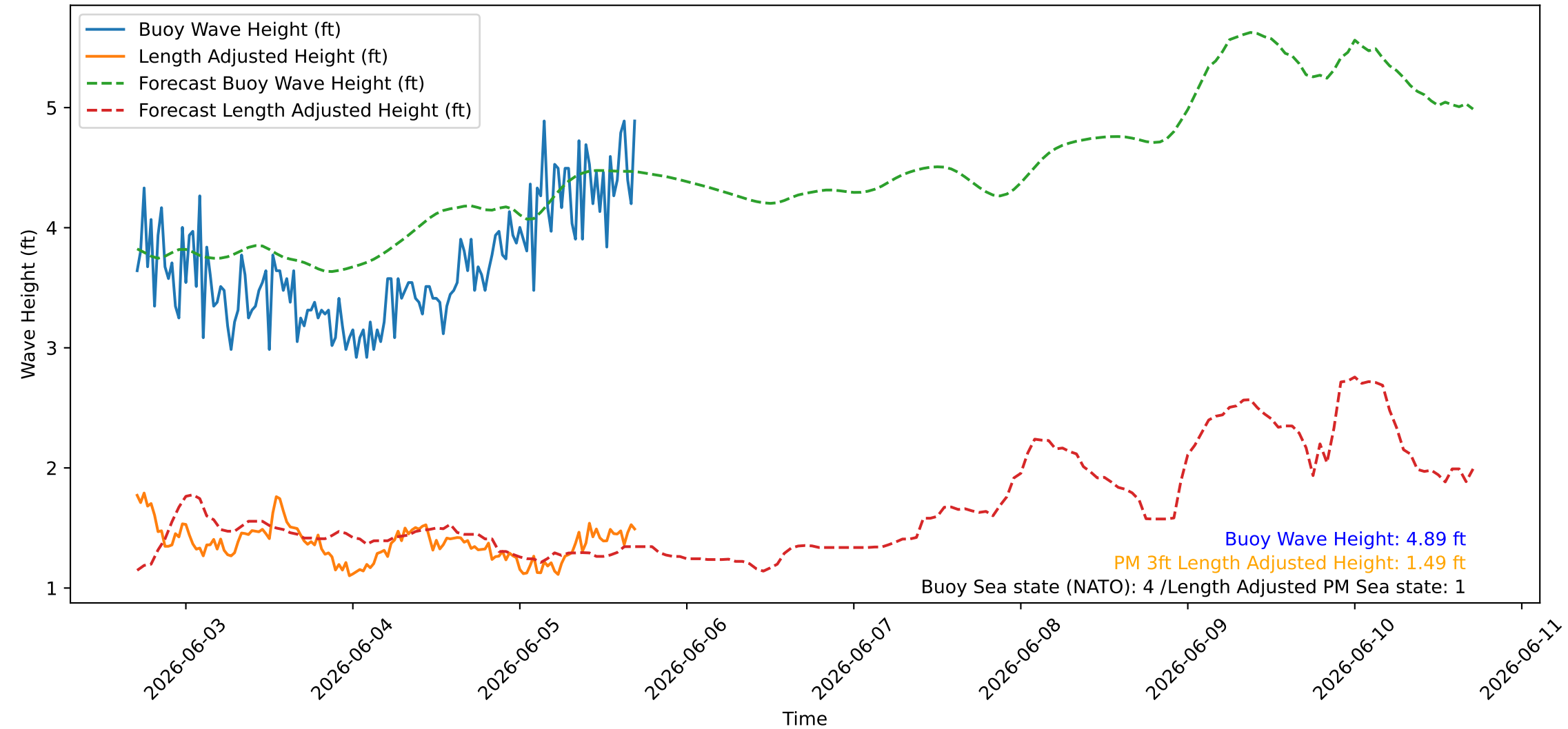
Wave Heights over Time for Oceanside Harbor at 2026-06-05 17:00:26
