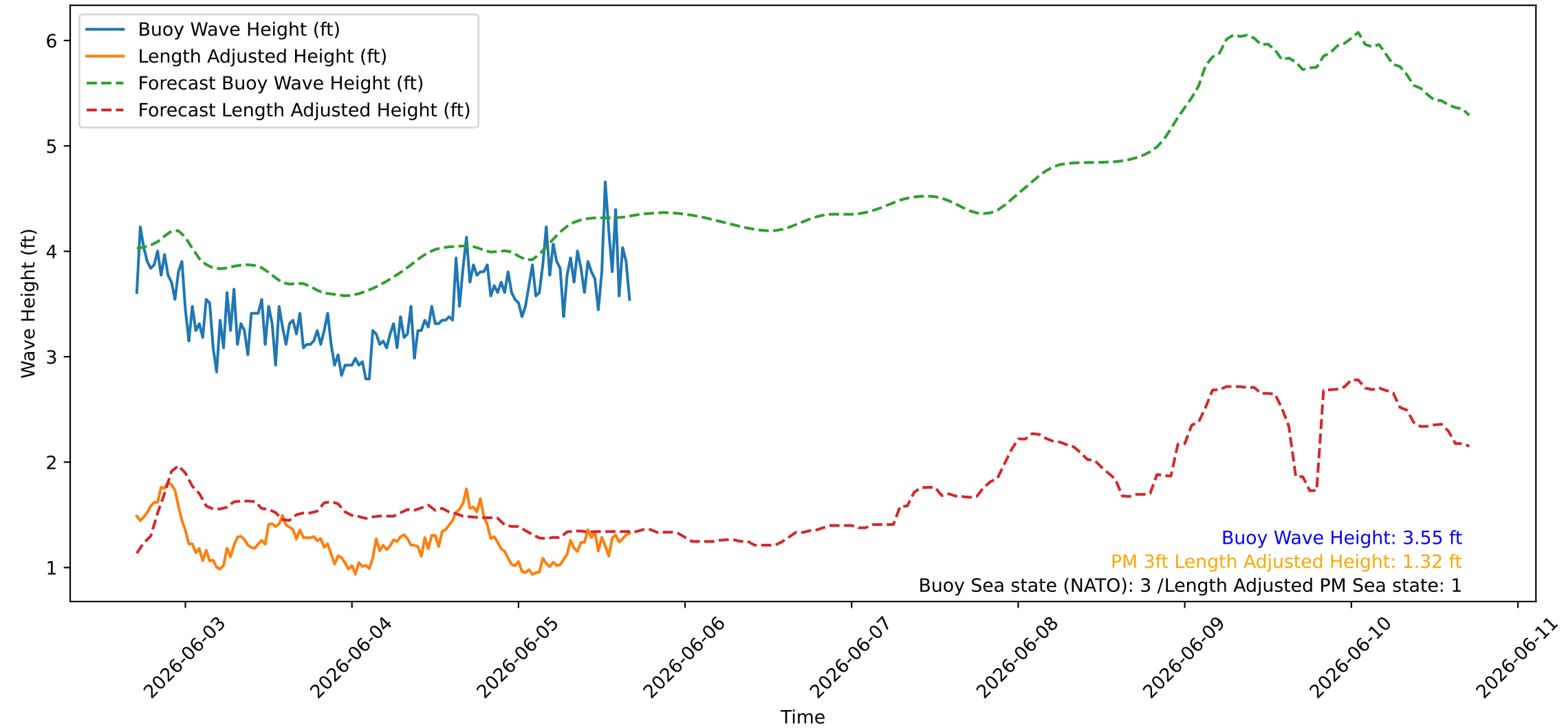
Wave Heights over Time for Green Beach at 2026-06-05 17:01:08
