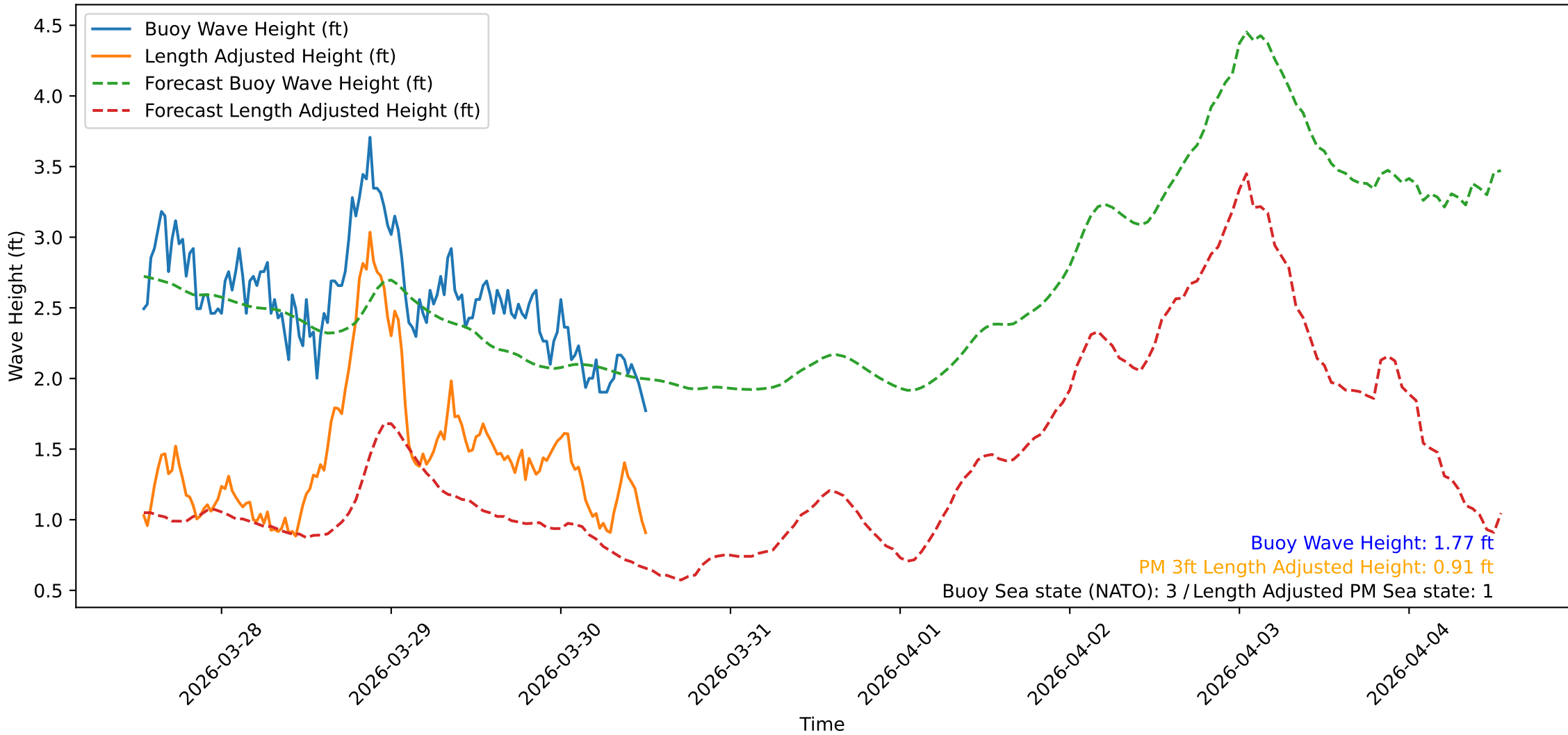
Wave Heights over Time for Green Beach at 2026-03-30 13:01:10
