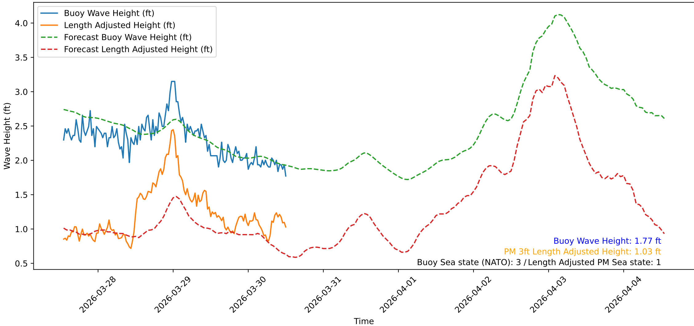
Wave Heights over Time for Oceanside Harbor at 2026-03-30 13:00:32
