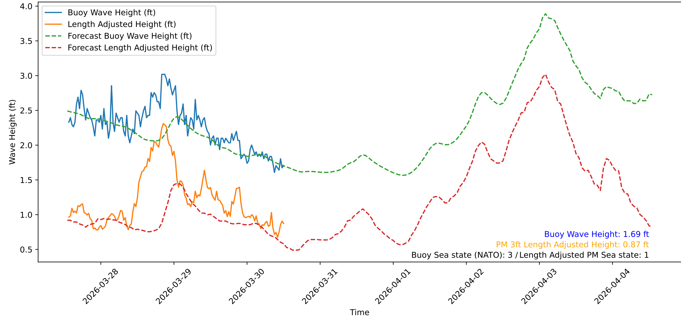
Wave Heights over Time for Red Beach at 2026-03-30 13:00:48
