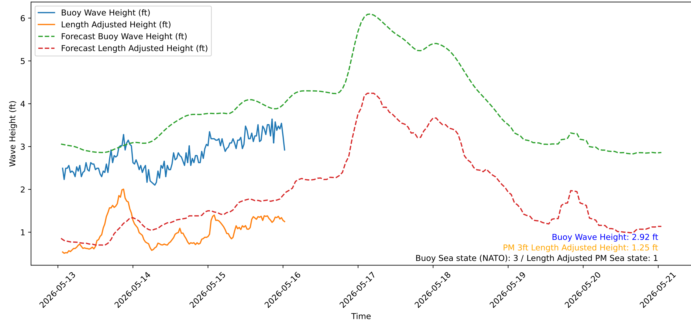
Wave Heights over Time for Green Beach at 2026-05-16 01:21:14
