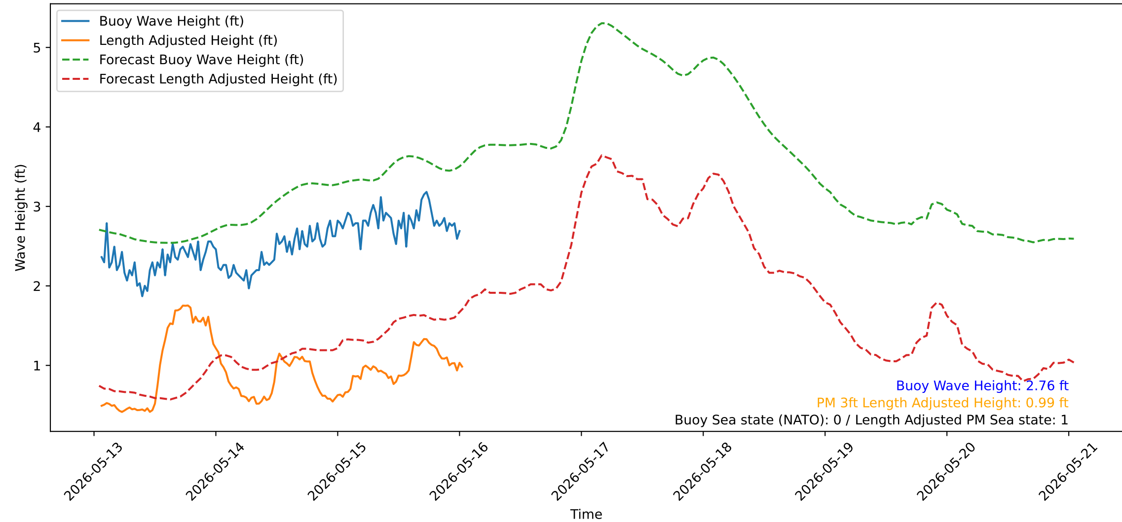
Wave Heights over Time for Red Beach at 2026-05-16 01:20:51
