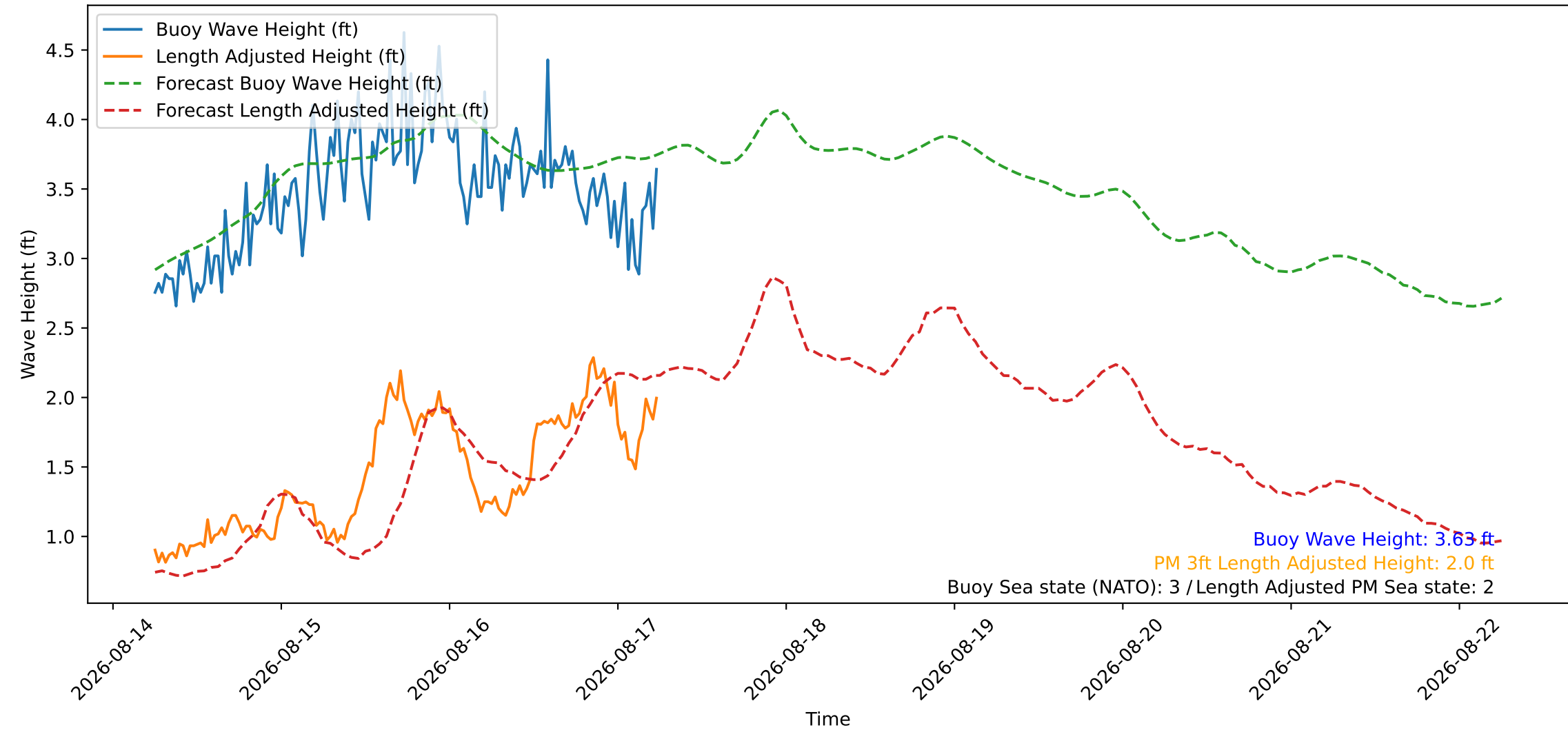
Wave Heights over Time for Oceanside Harbor at 2026-08-17 06:10:26
