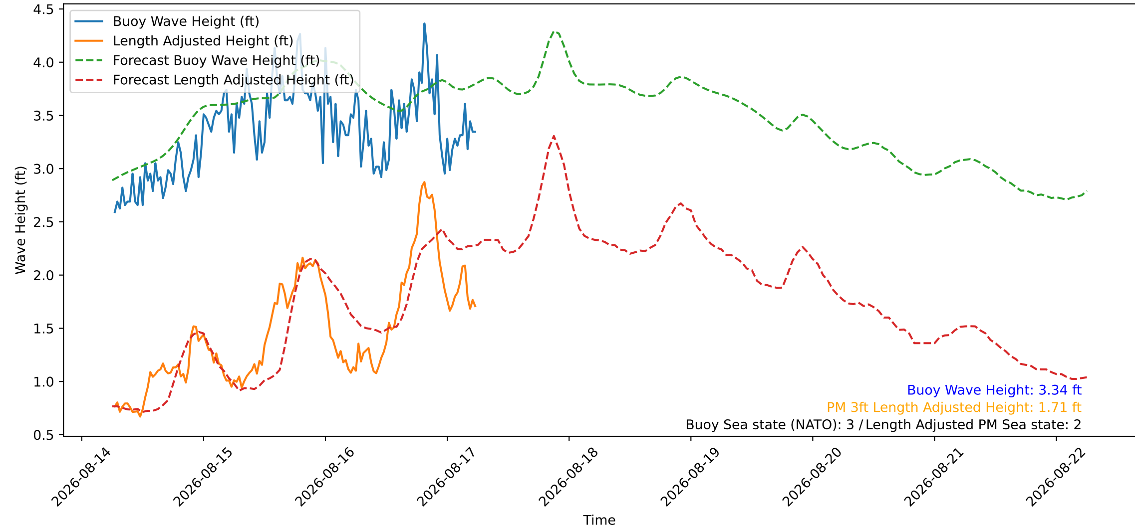
Wave Heights over Time for Green Beach at 2026-08-17 06:11:08
