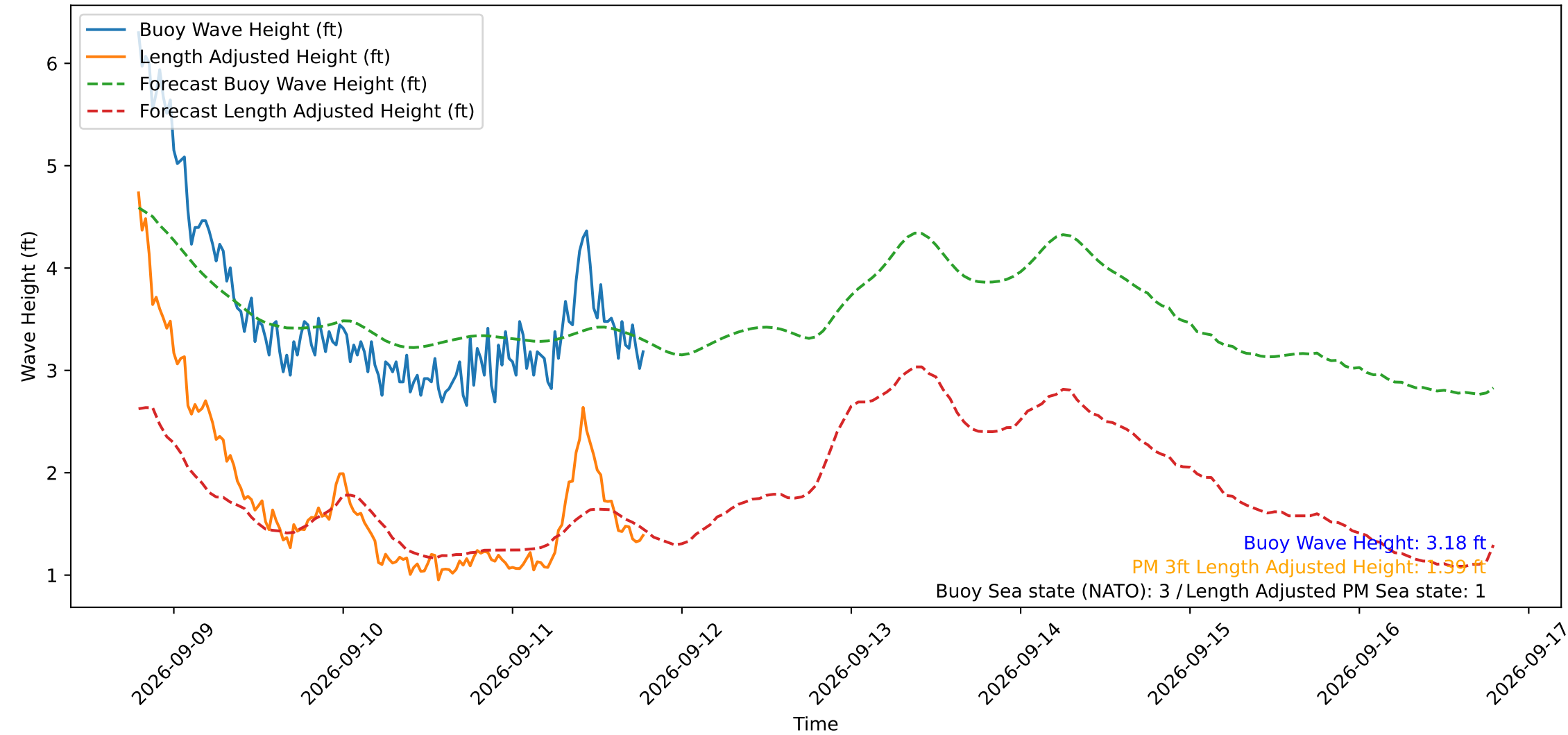
Wave Heights over Time for Oceanside Harbor at 2026-09-11 19:00:30
