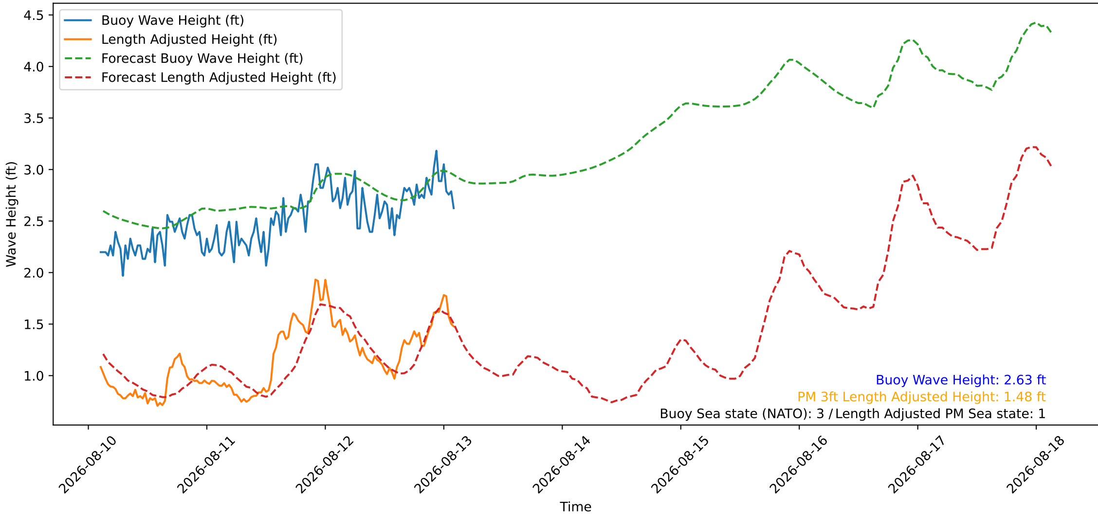
Wave Heights over Time for Oceanside Harbor at 2026-08-13 02:40:26
