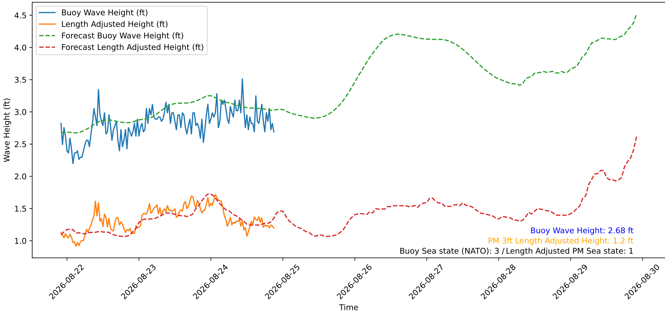
Wave Heights over Time for Oceanside Harbor at 2026-08-24 21:50:29
