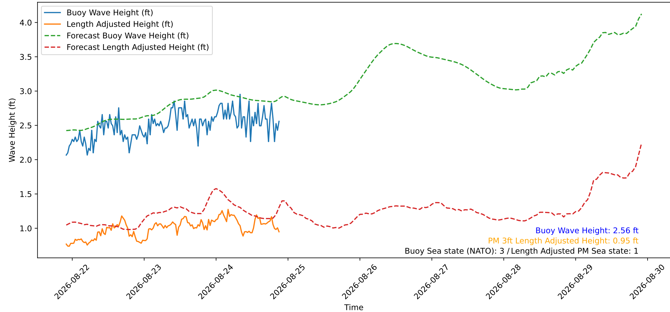
Wave Heights over Time for Red Beach at 2026-08-24 21:50:50
