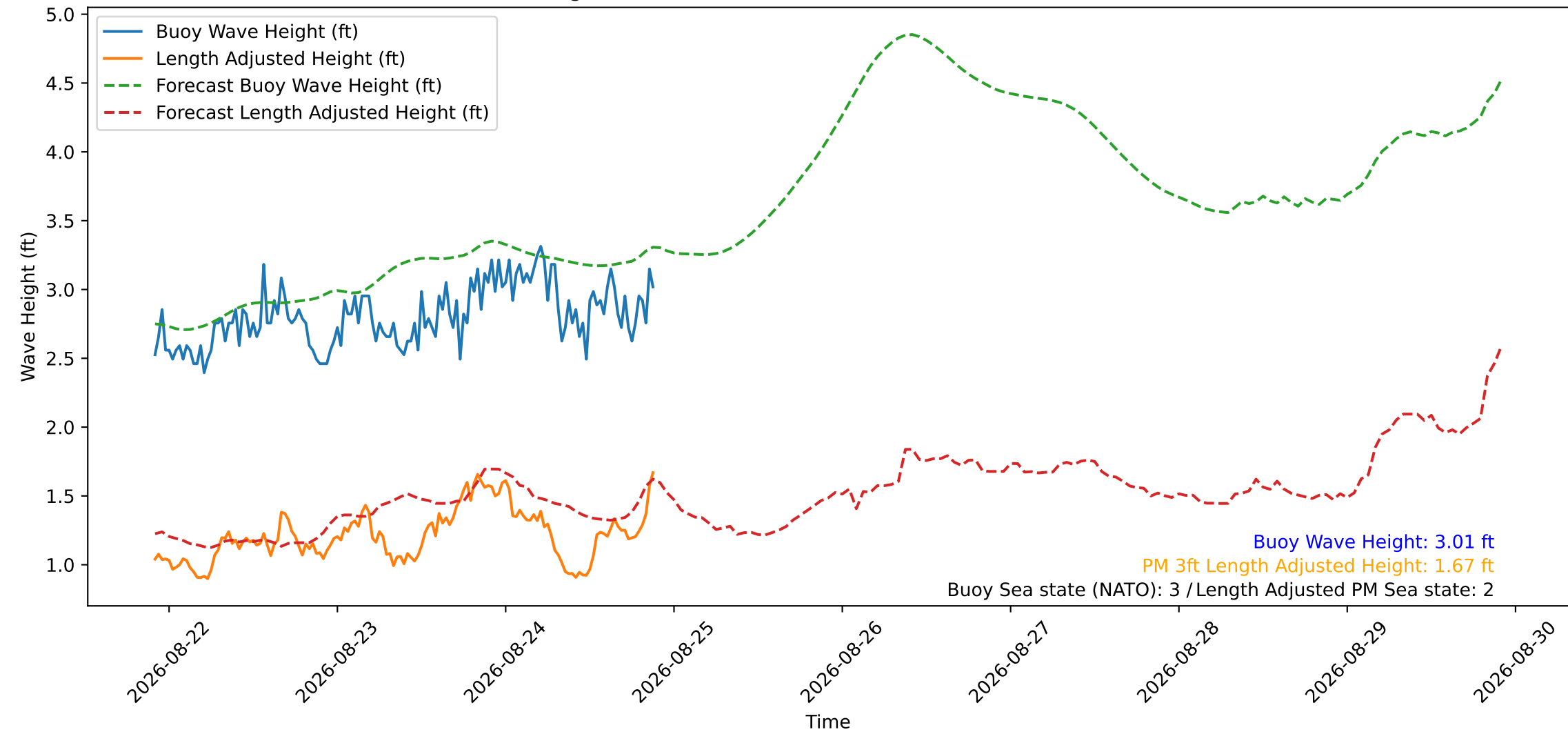
Wave Heights over Time for Green Beach at 2026-08-24 21:51:14
