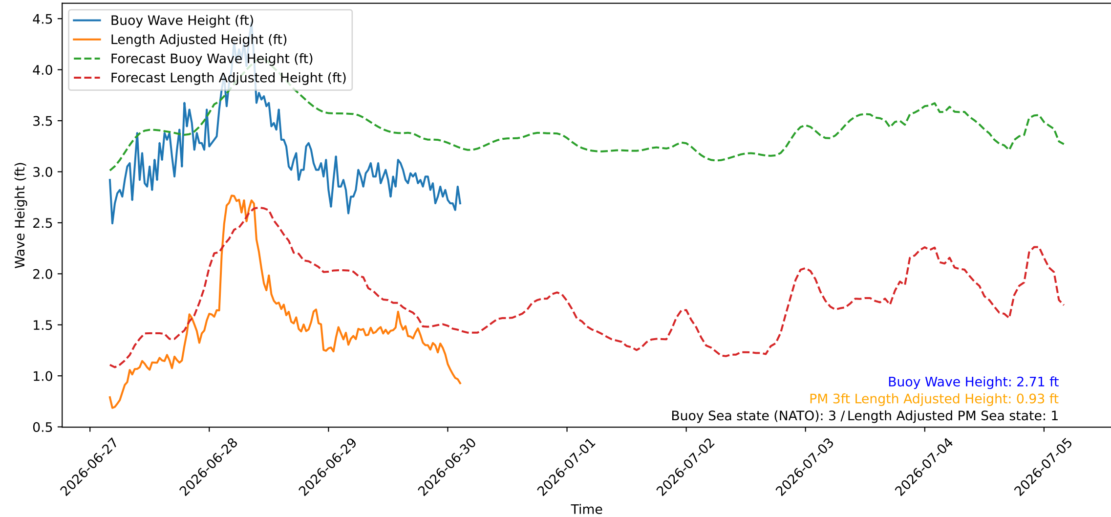
Wave Heights over Time for Red Beach at 2026-06-30 03:30:45
