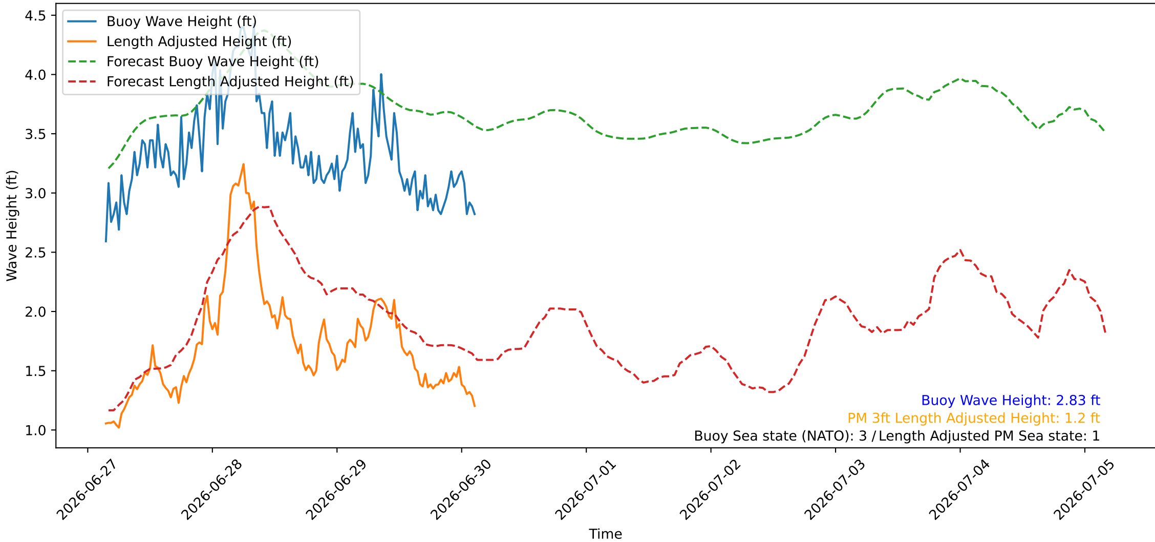
Wave Heights over Time for Oceanside Harbor at 2026-06-30 03:30:26
