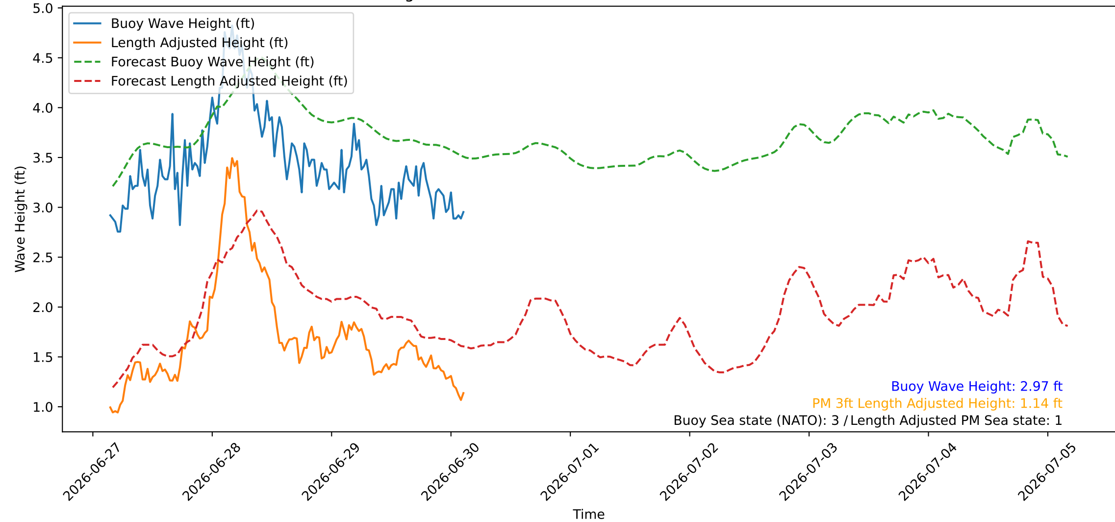
Wave Heights over Time for Green Beach at 2026-06-30 03:31:08
