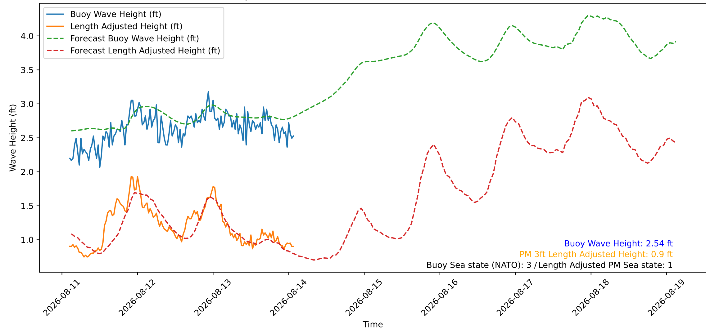
Wave Heights over Time for Oceanside Harbor at 2026-08-14 02:30:26
