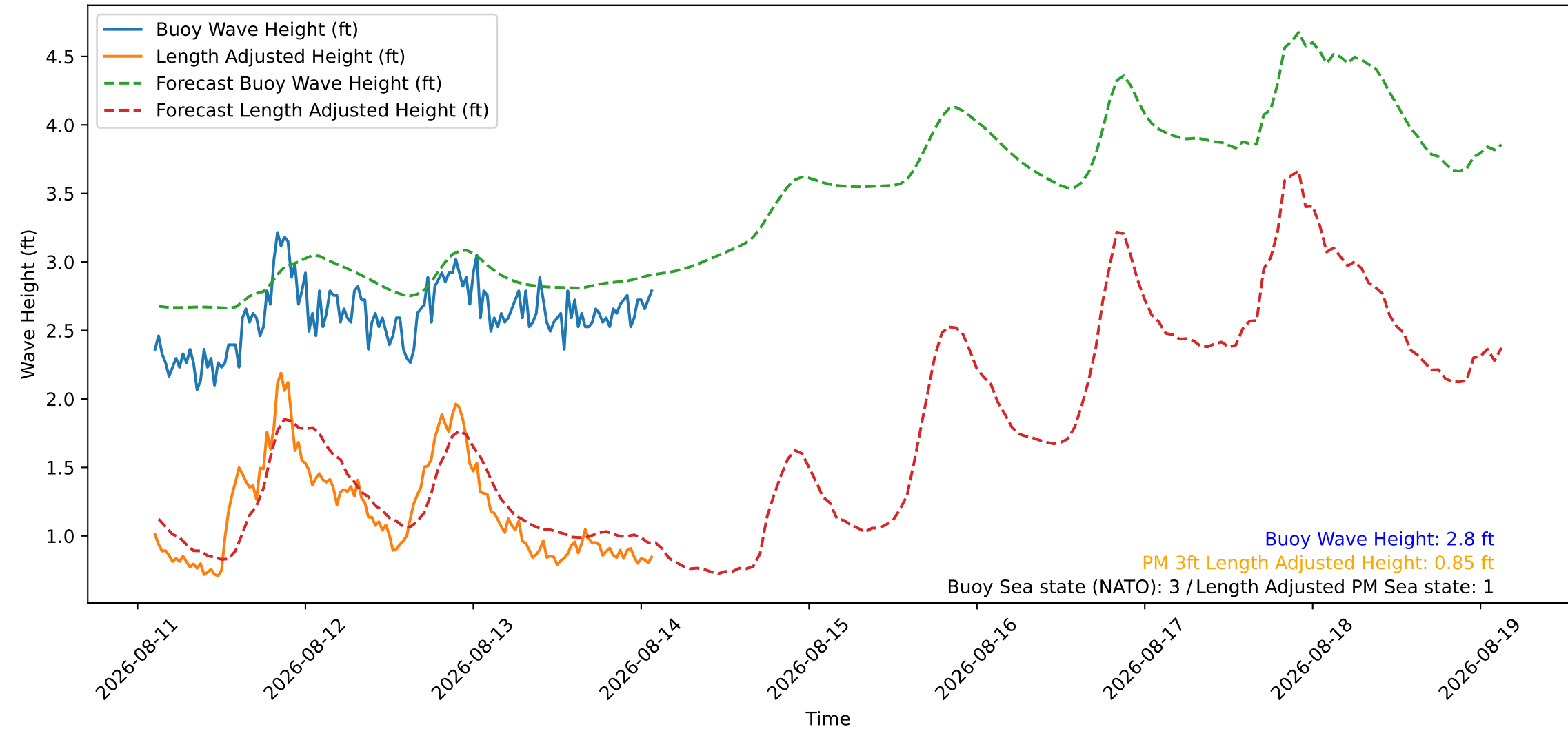
Wave Heights over Time for Green Beach at 2026-08-14 02:31:08
