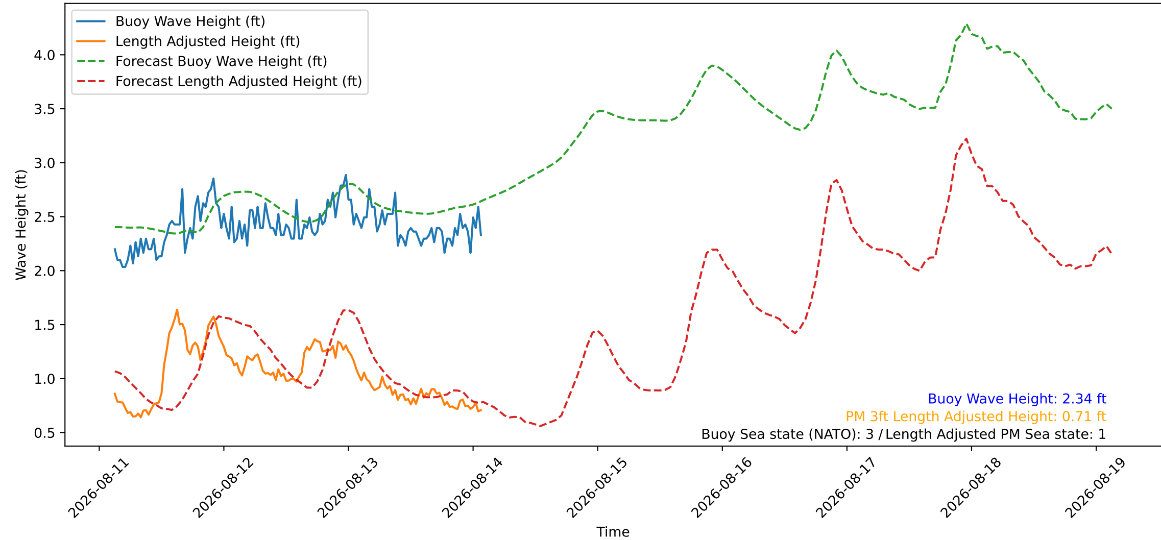
Wave Heights over Time for Red Beach at 2026-08-14 02:30:46
