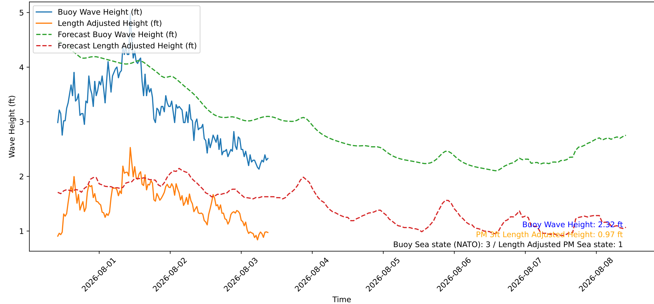
Wave Heights over Time for Green Beach at 2026-08-03 10:11:07
