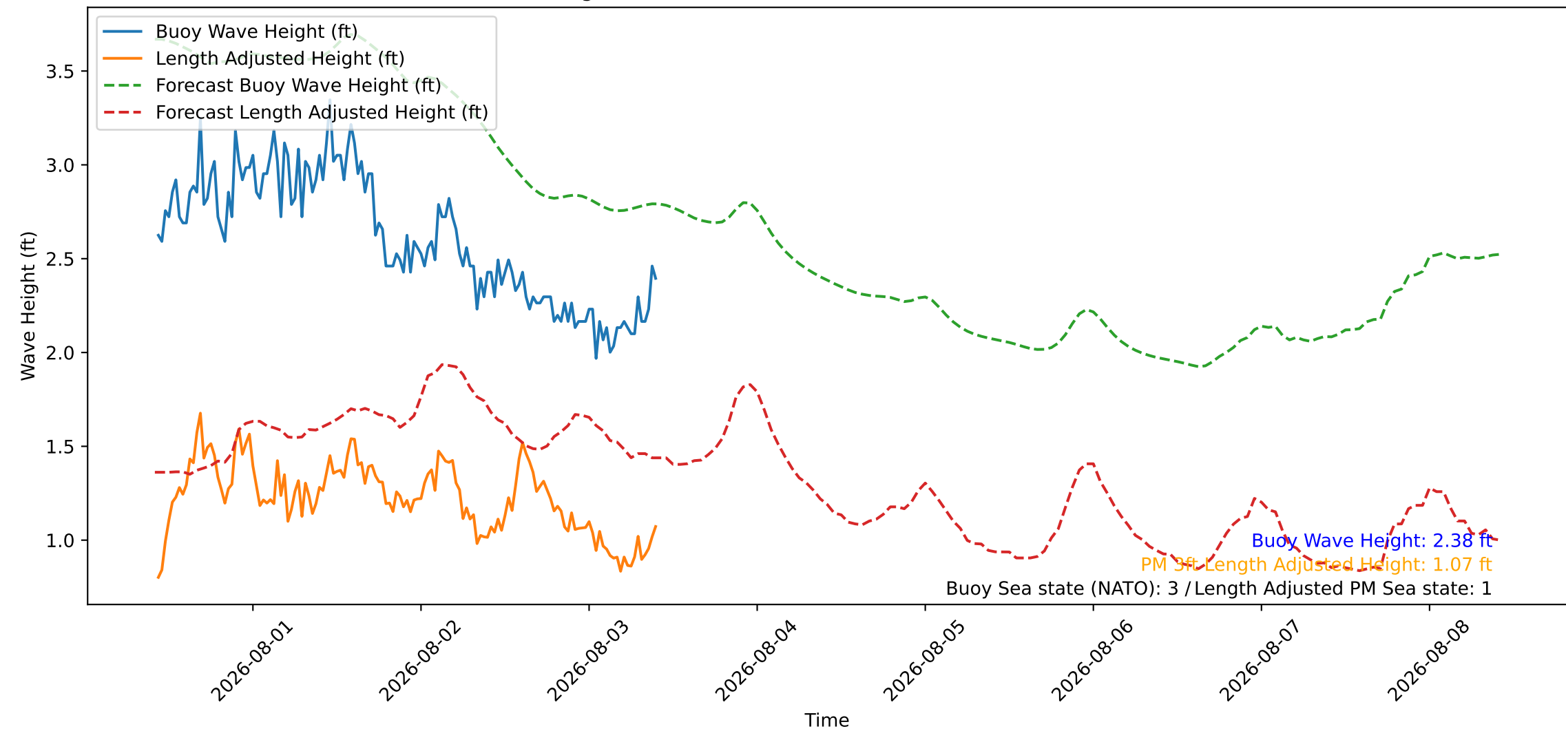
Wave Heights over Time for Red Beach at 2026-08-03 10:10:45
