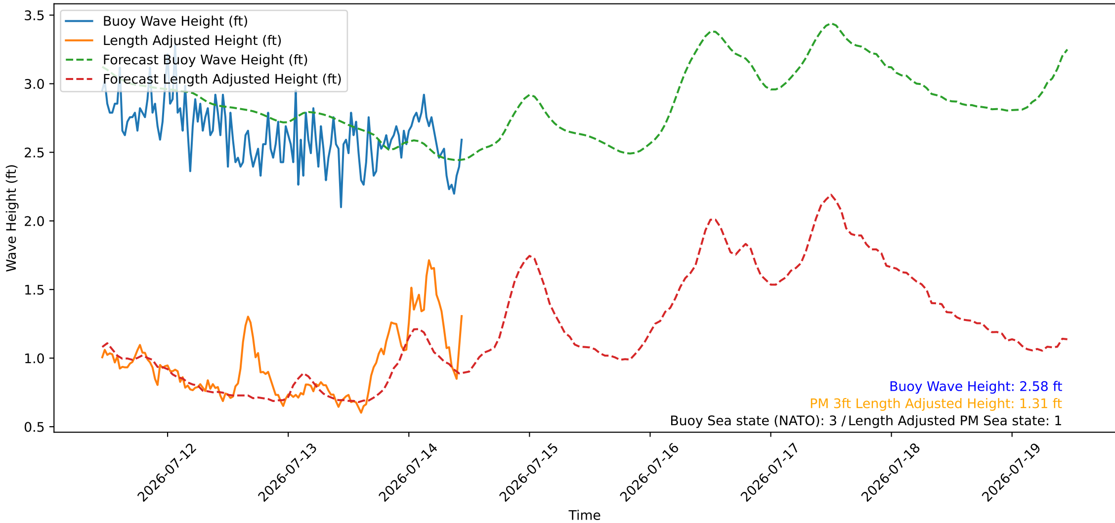
Wave Heights over Time for Oceanside Harbor at 2026-07-14 11:00:27
