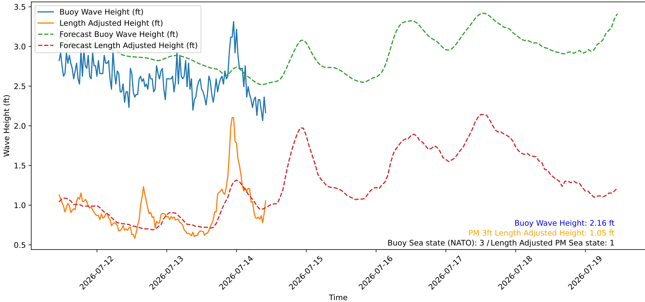
Wave Heights over Time for Green Beach at 2026-07-14 11:01:09
