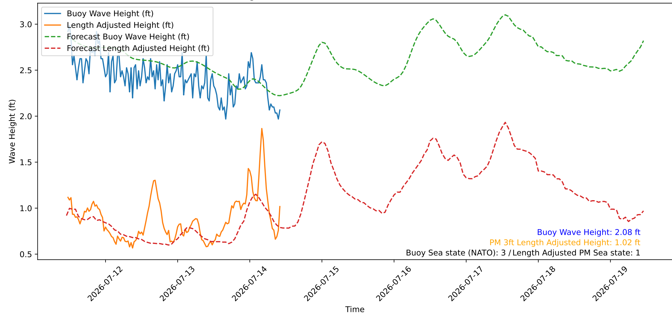
Wave Heights over Time for Red Beach at 2026-07-14 11:00:46
