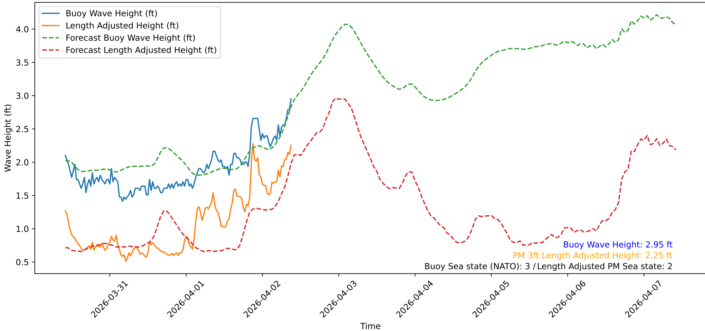
Wave Heights over Time for Green Beach at 2026-04-02 09:51:10
