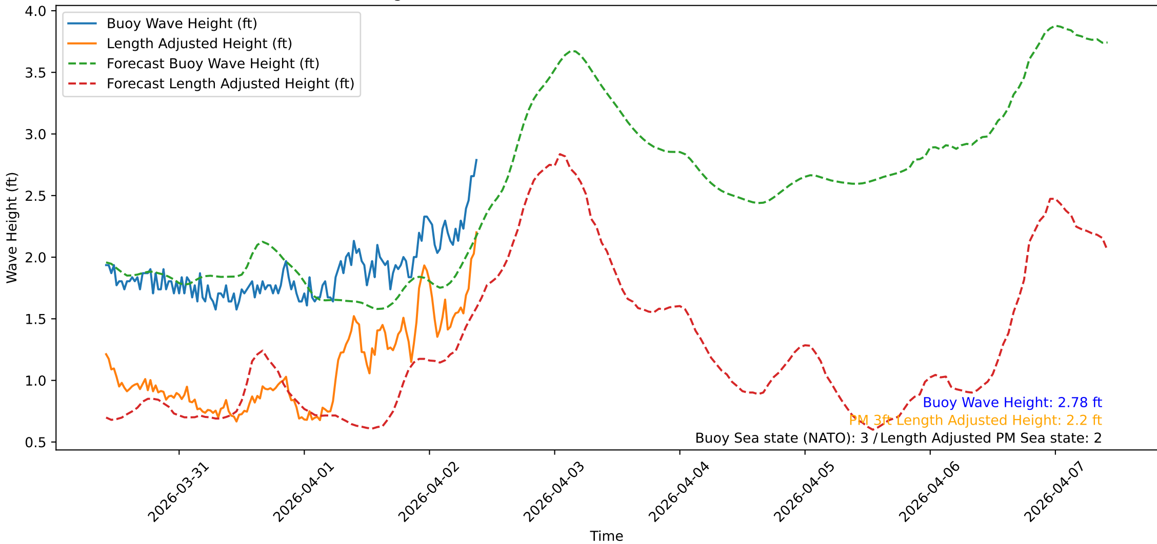
Wave Heights over Time for Oceanside Harbor at 2026-04-02 09:50:31
