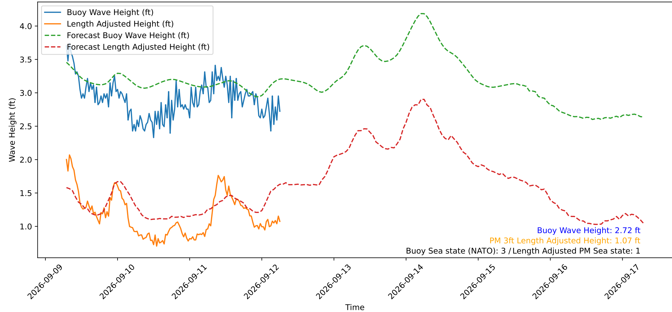
Wave Heights over Time for Red Beach at 2026-09-12 06:40:49
