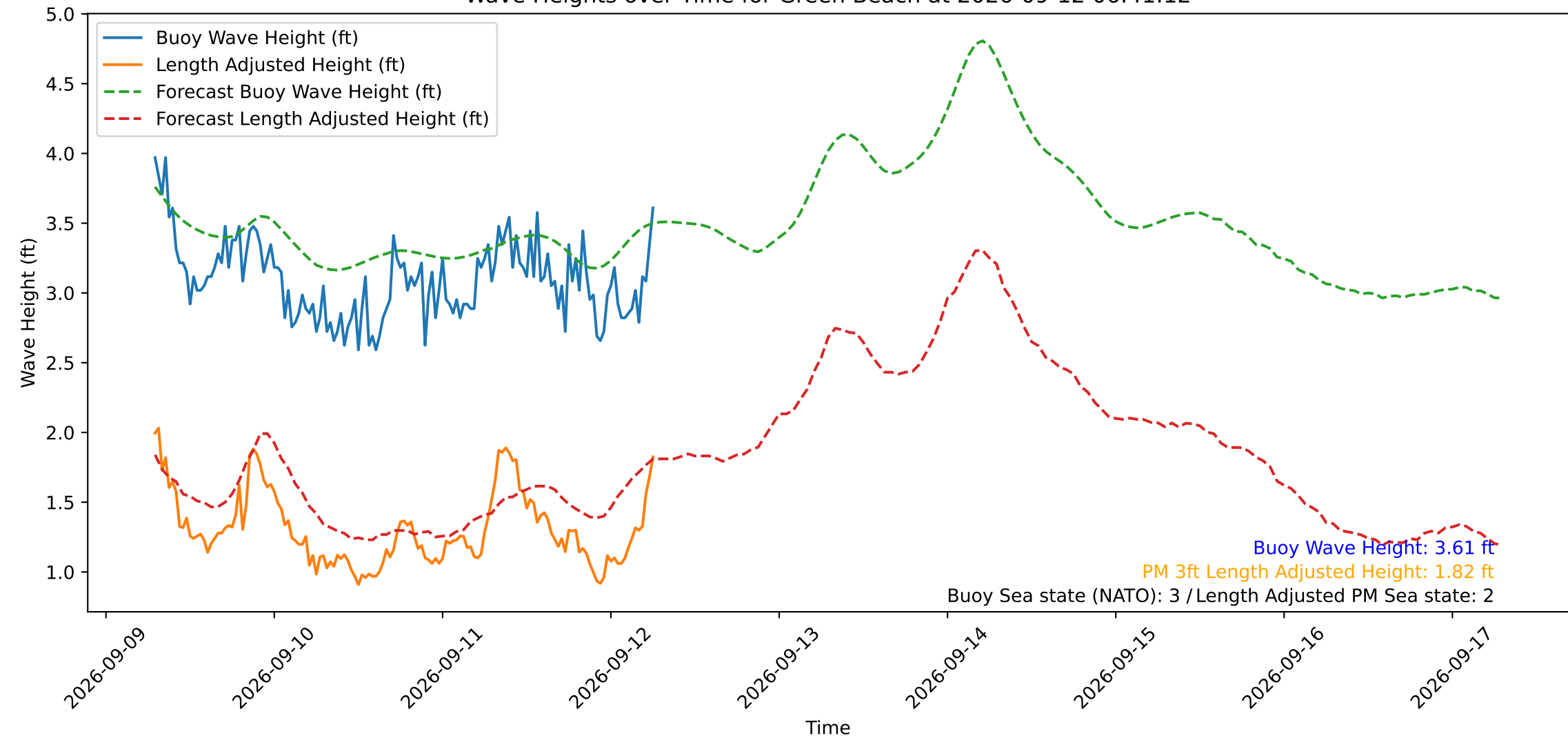
Wave Heights over Time for Green Beach at 2026-09-12 06:41:12
