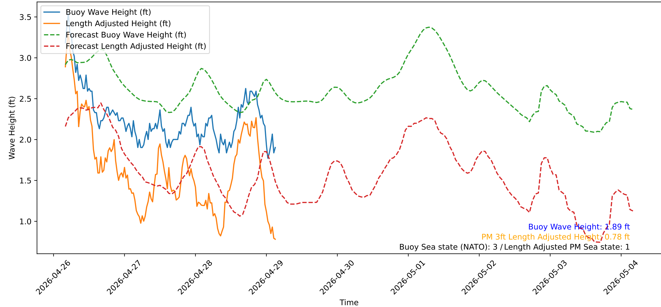
Wave Heights over Time for Red Beach at 2026-04-29 03:50:52
