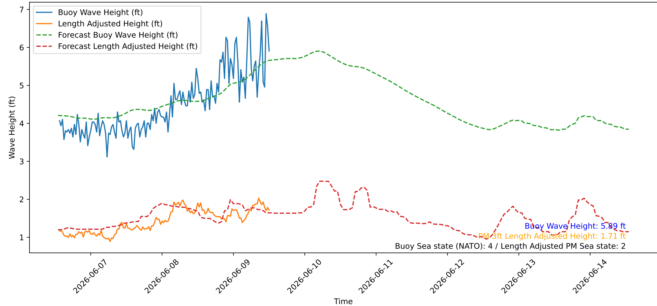
Wave Heights over Time for Green Beach at 2026-06-09 13:21:09
