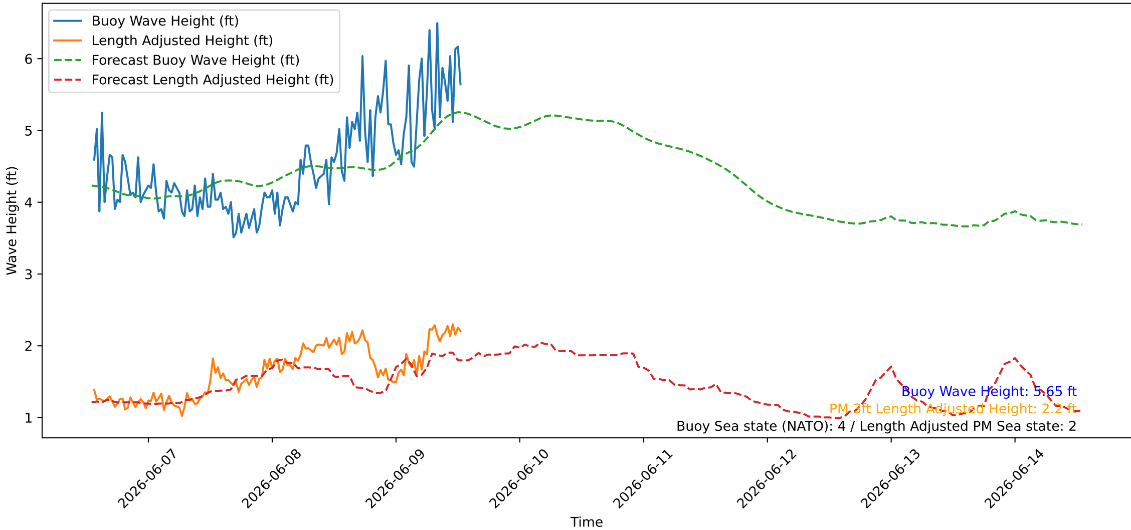
Wave Heights over Time for Oceanside Harbor at 2026-06-09 13:20:26
