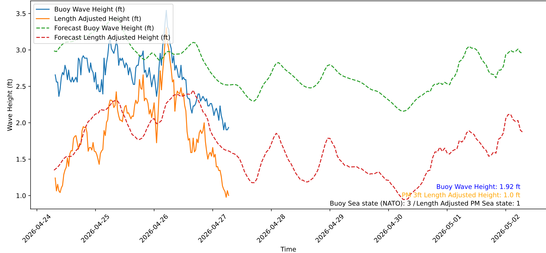
Wave Heights over Time for Red Beach at 2026-04-27 07:20:51
