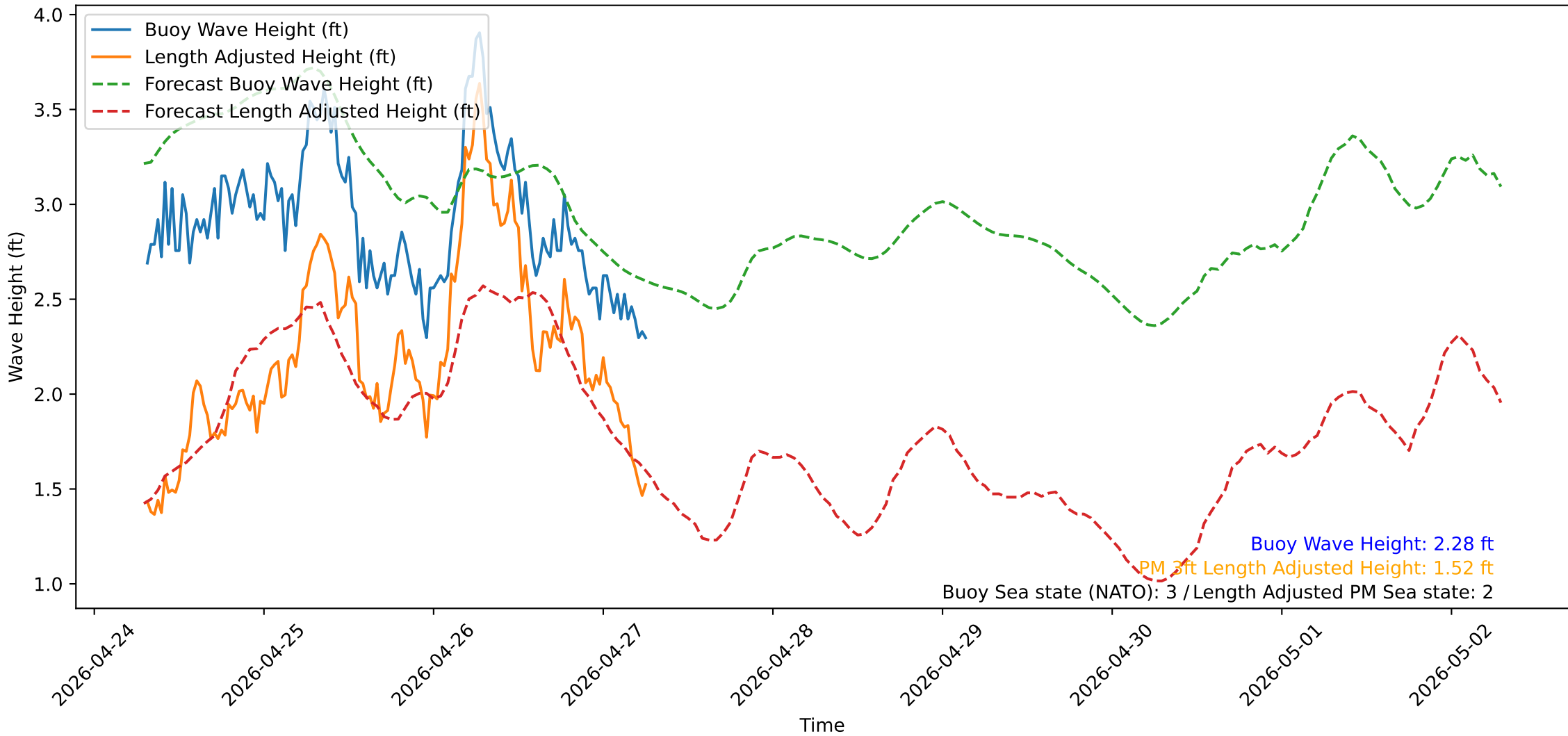
Wave Heights over Time for Oceanside Harbor at 2026-04-27 07:20:30
