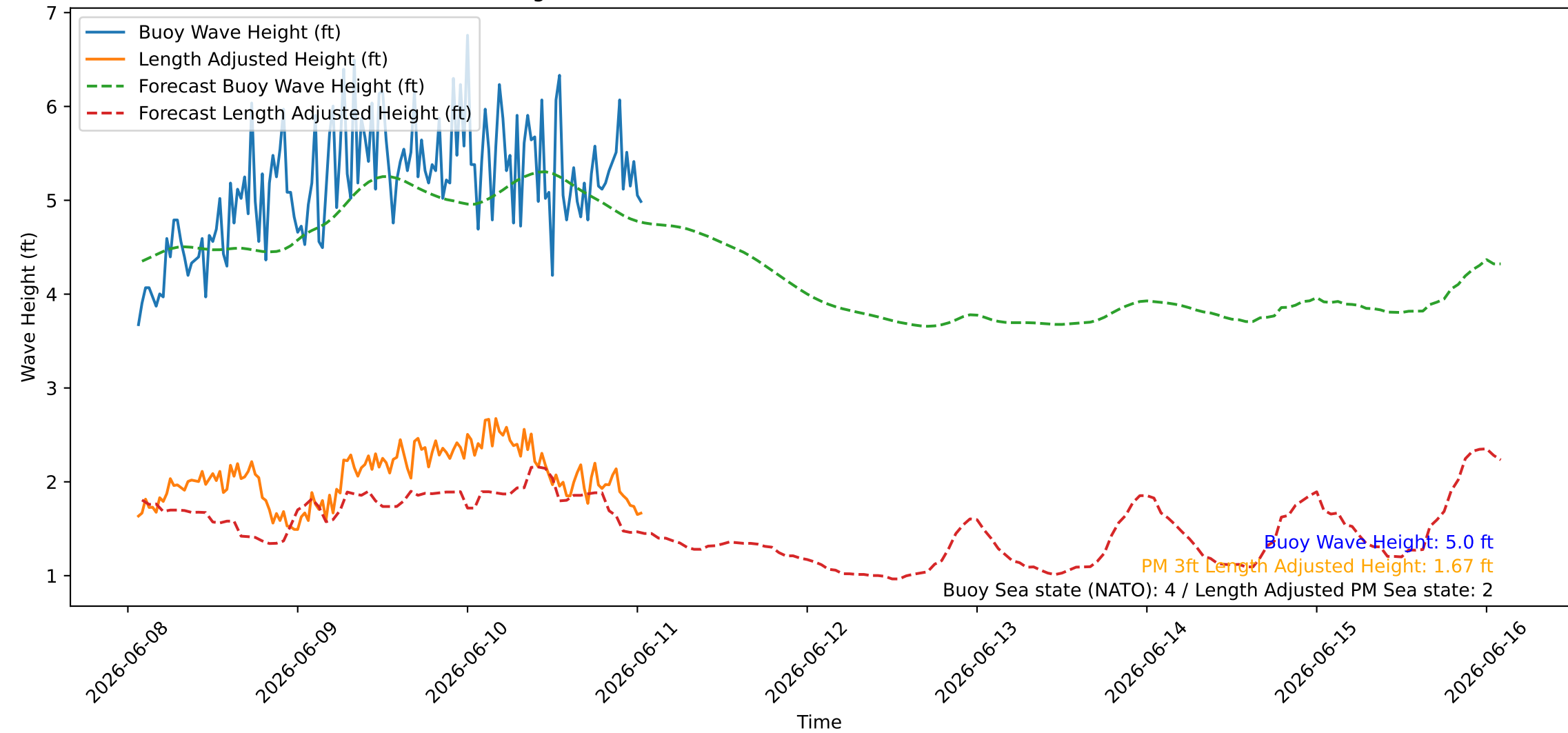
Wave Heights over Time for Oceanside Harbor at 2026-06-11 01:30:27
