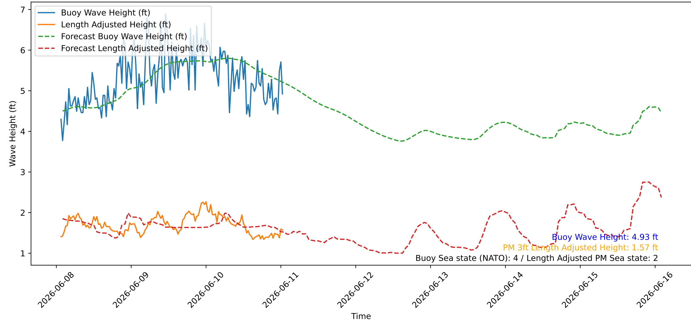
Wave Heights over Time for Green Beach at 2026-06-11 01:31:10
