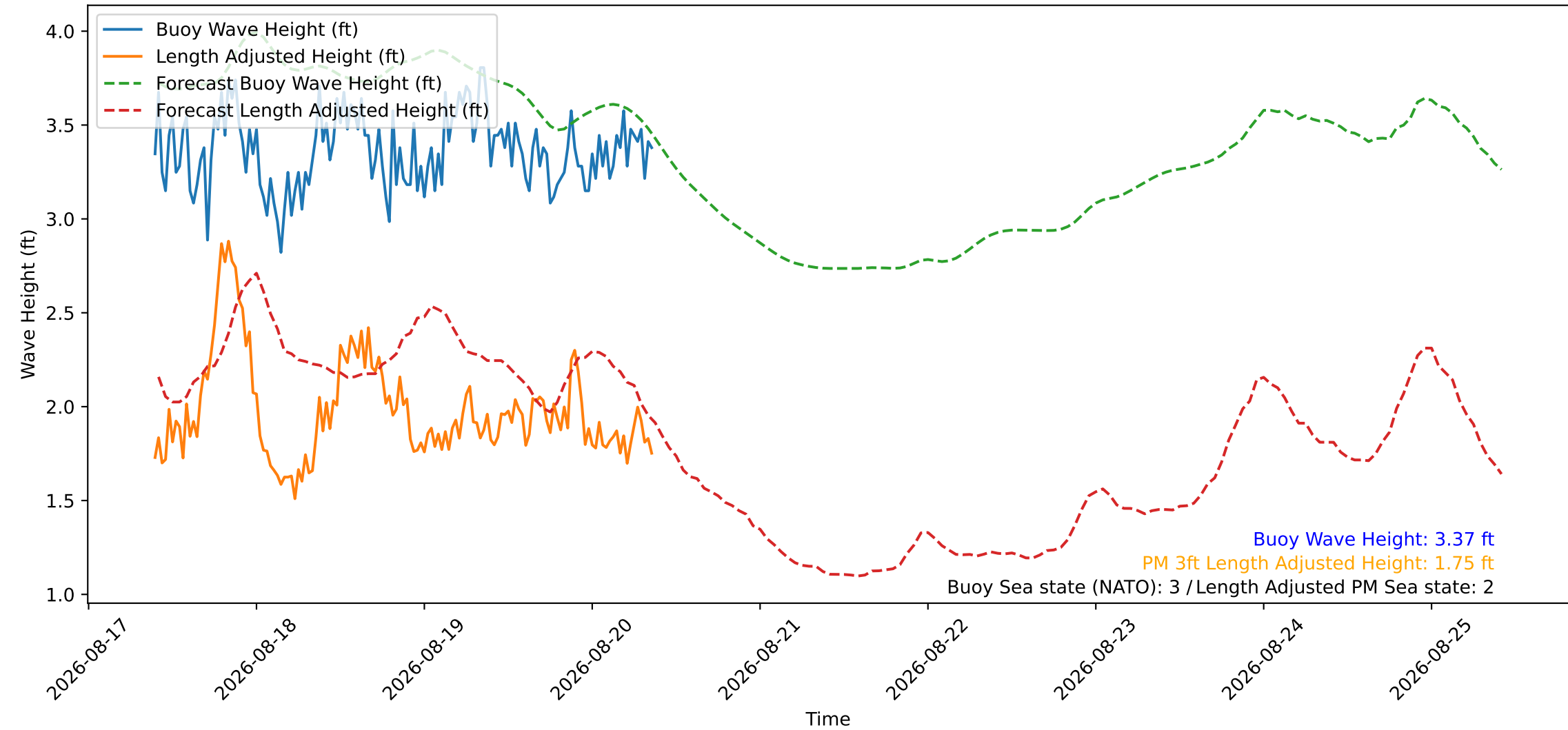
Wave Heights over Time for Oceanside Harbor at 2026-08-20 09:30:27
