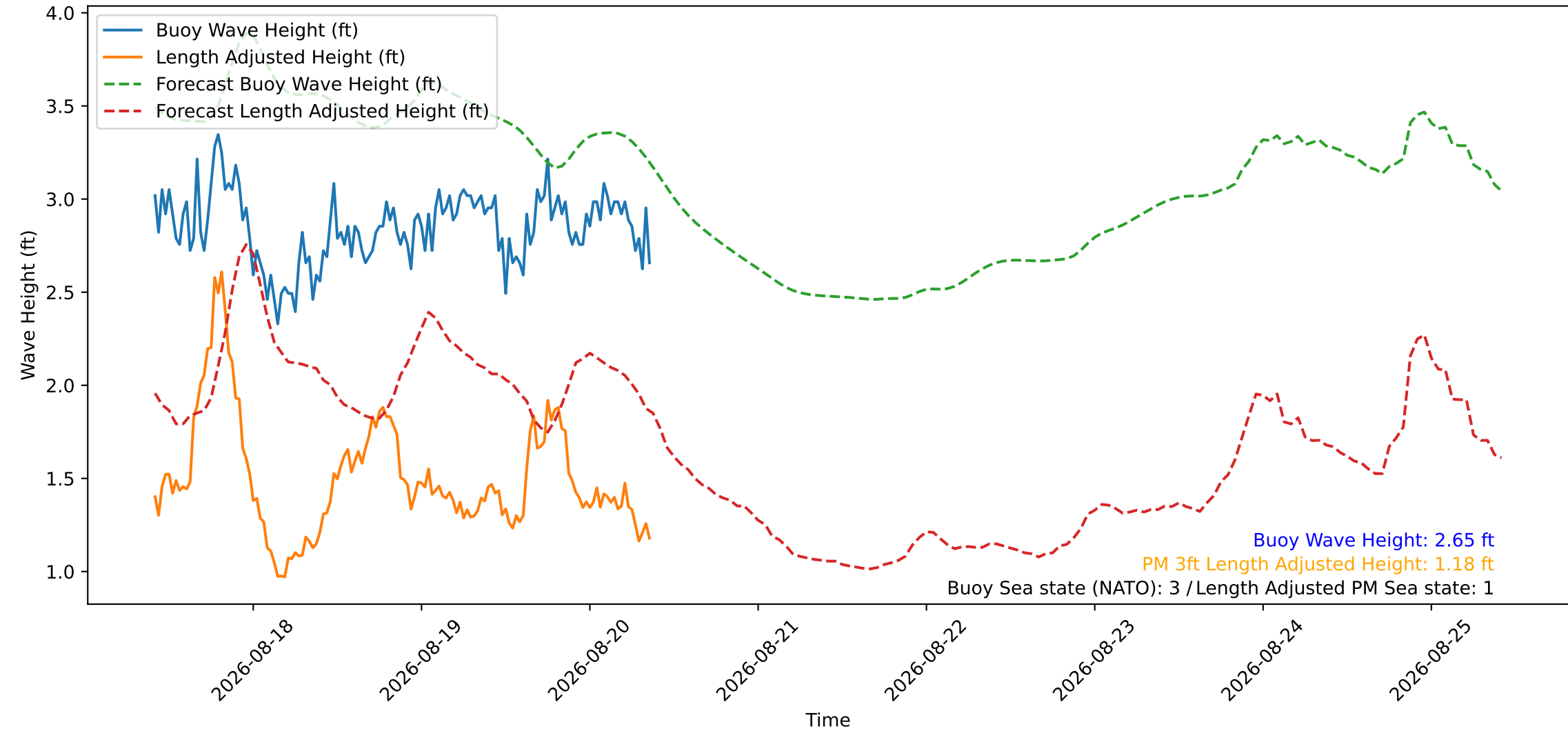
Wave Heights over Time for Red Beach at 2026-08-20 09:30:46
