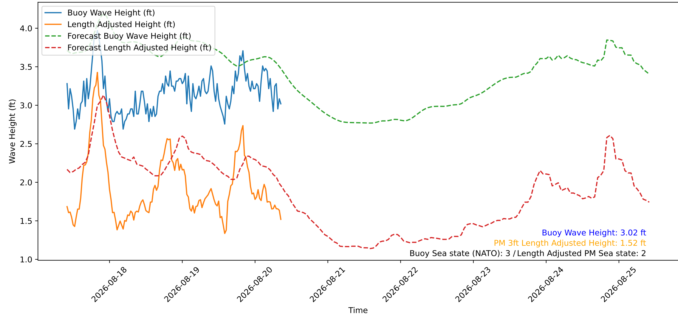
Wave Heights over Time for Green Beach at 2026-08-20 09:31:09
