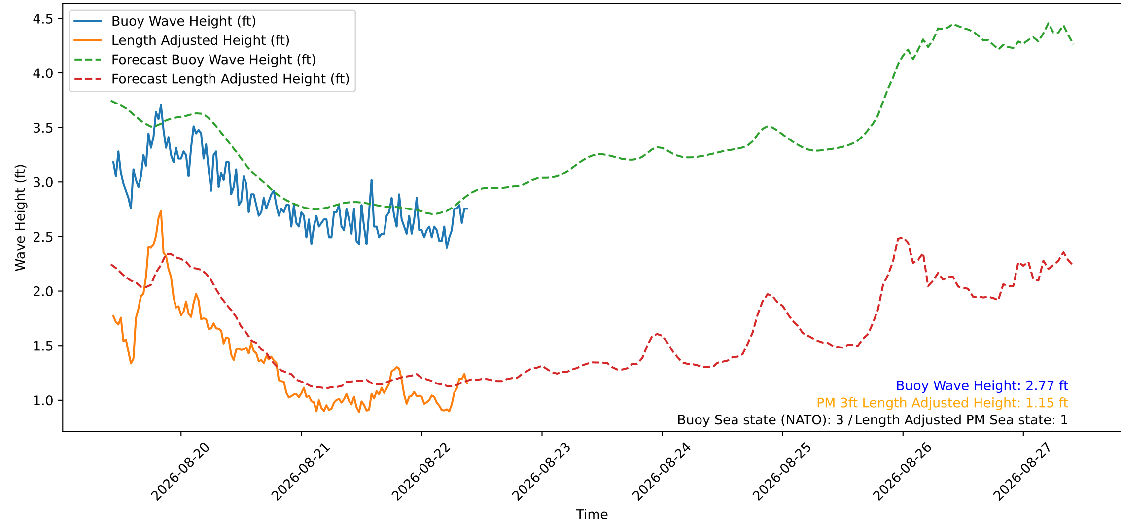
Wave Heights over Time for Green Beach at 2026-08-22 10:01:12
