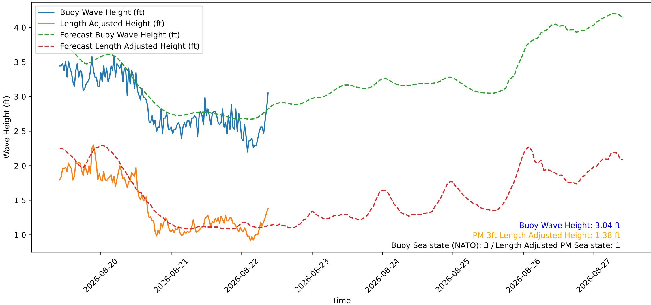
Wave Heights over Time for Oceanside Harbor at 2026-08-22 10:00:29
