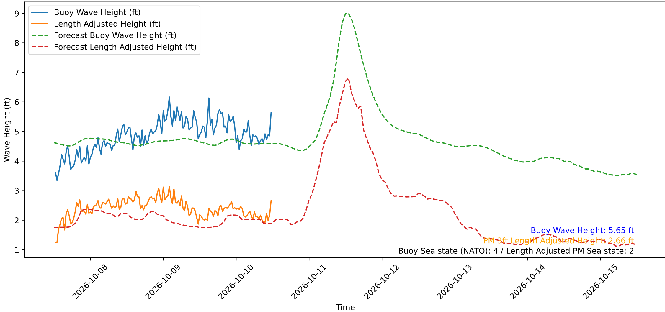
Wave Heights over Time for Green Beach at 2026-10-10 12:11:12
