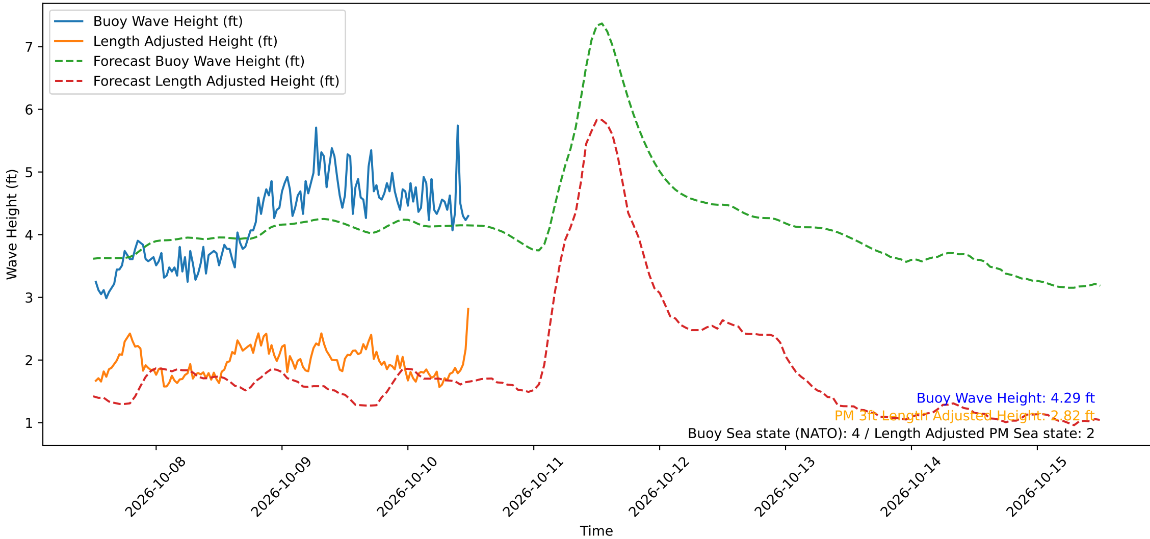
Wave Heights over Time for Red Beach at 2026-10-10 12:10:49
