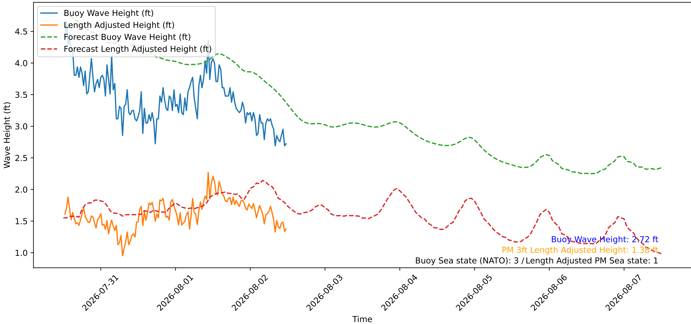
Wave Heights over Time for Oceanside Harbor at 2026-08-02 12:20:27
