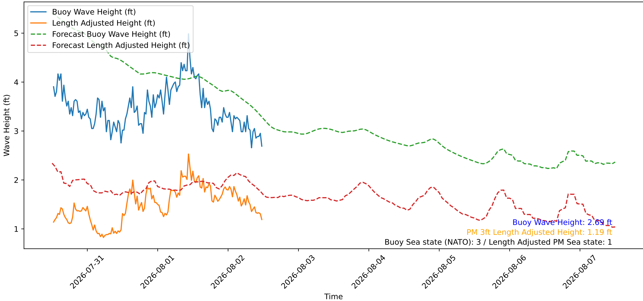
Wave Heights over Time for Green Beach at 2026-08-02 12:21:09
