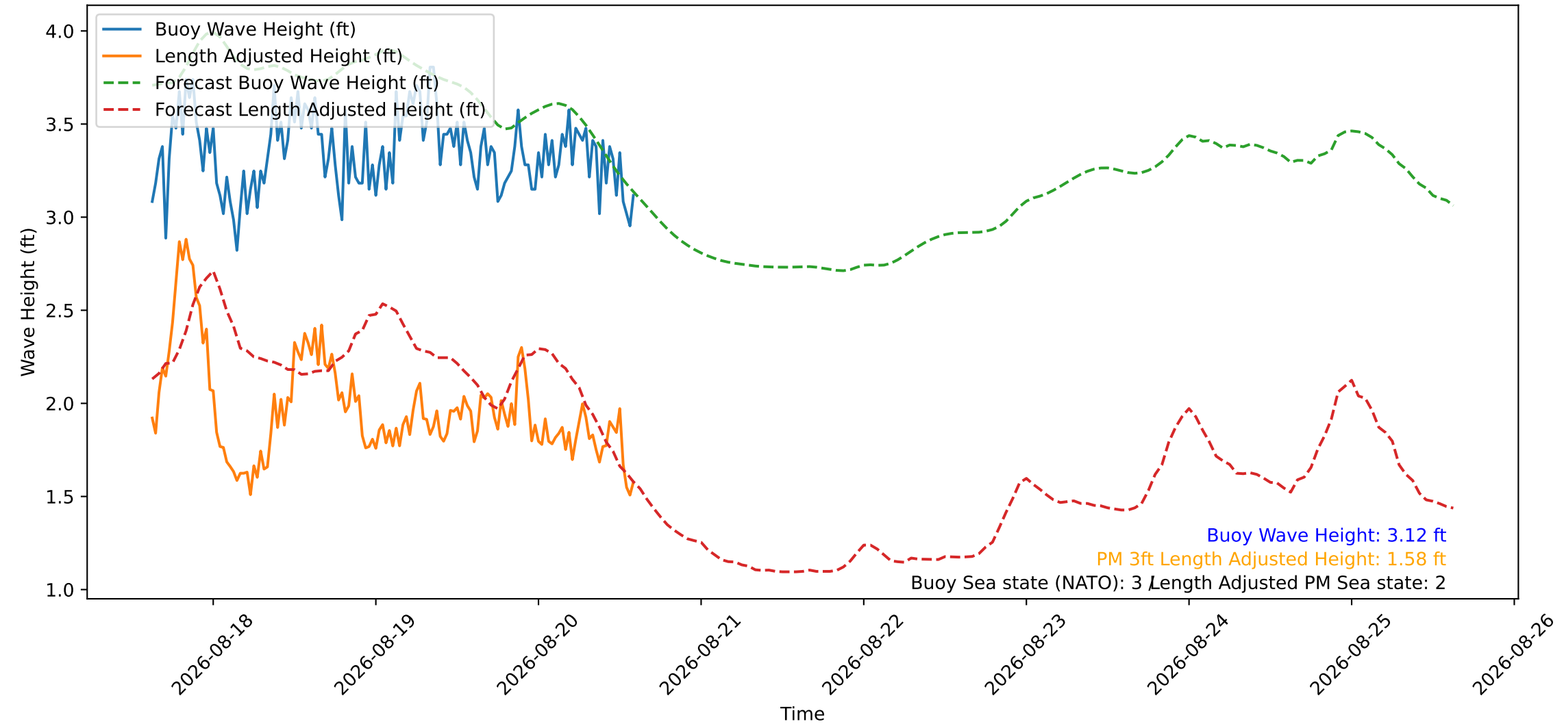
Wave Heights over Time for Oceanside Harbor at 2026-08-20 14:50:26
