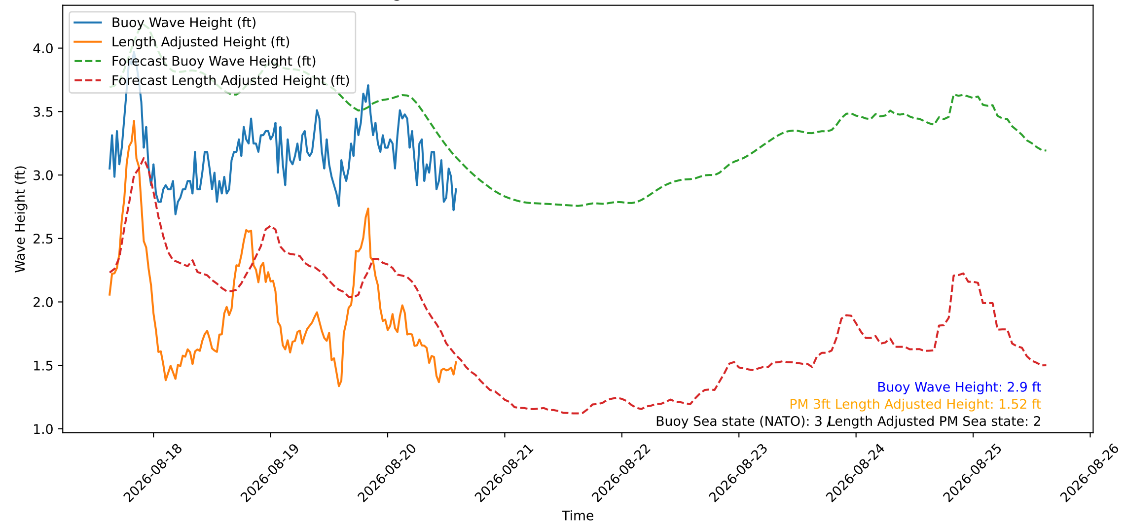
Wave Heights over Time for Green Beach at 2026-08-20 14:51:11
