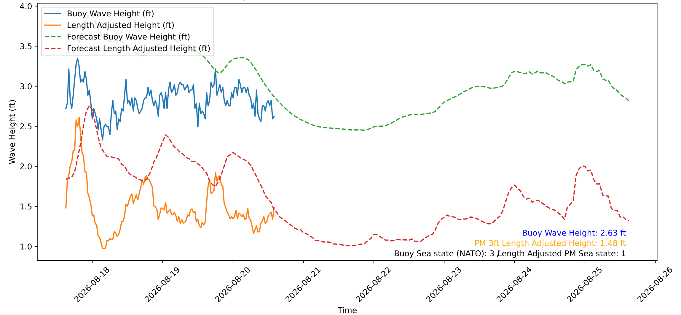
Wave Heights over Time for Red Beach at 2026-08-20 14:50:47
