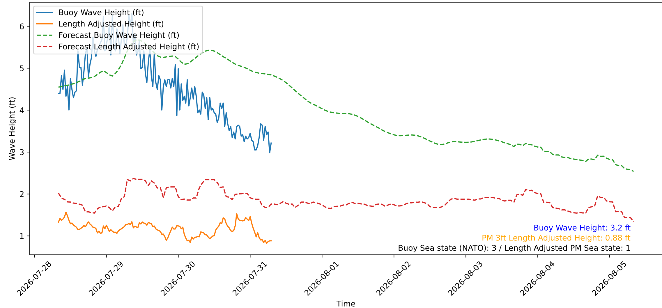
Wave Heights over Time for Green Beach at 2026-07-31 08:01:07
