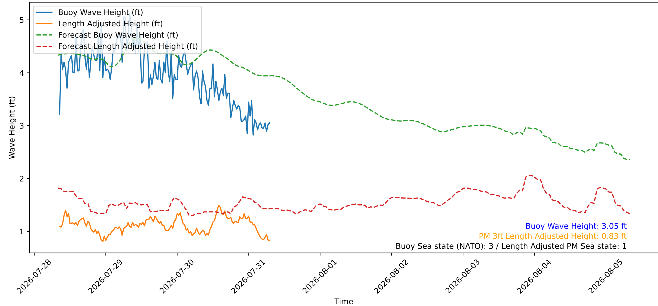
Wave Heights over Time for Red Beach at 2026-07-31 08:00:45
