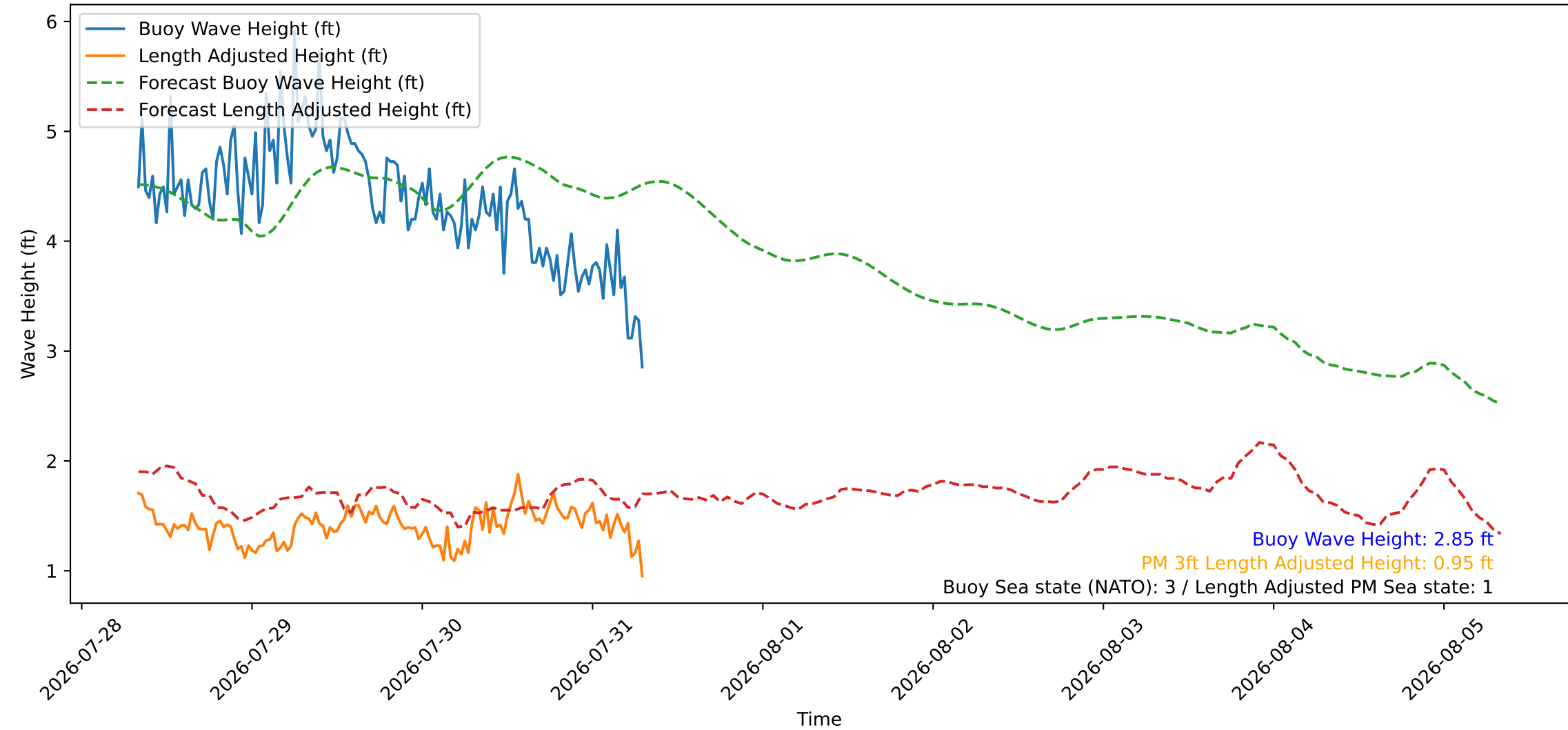
Wave Heights over Time for Oceanside Harbor at 2026-07-31 08:00:26
