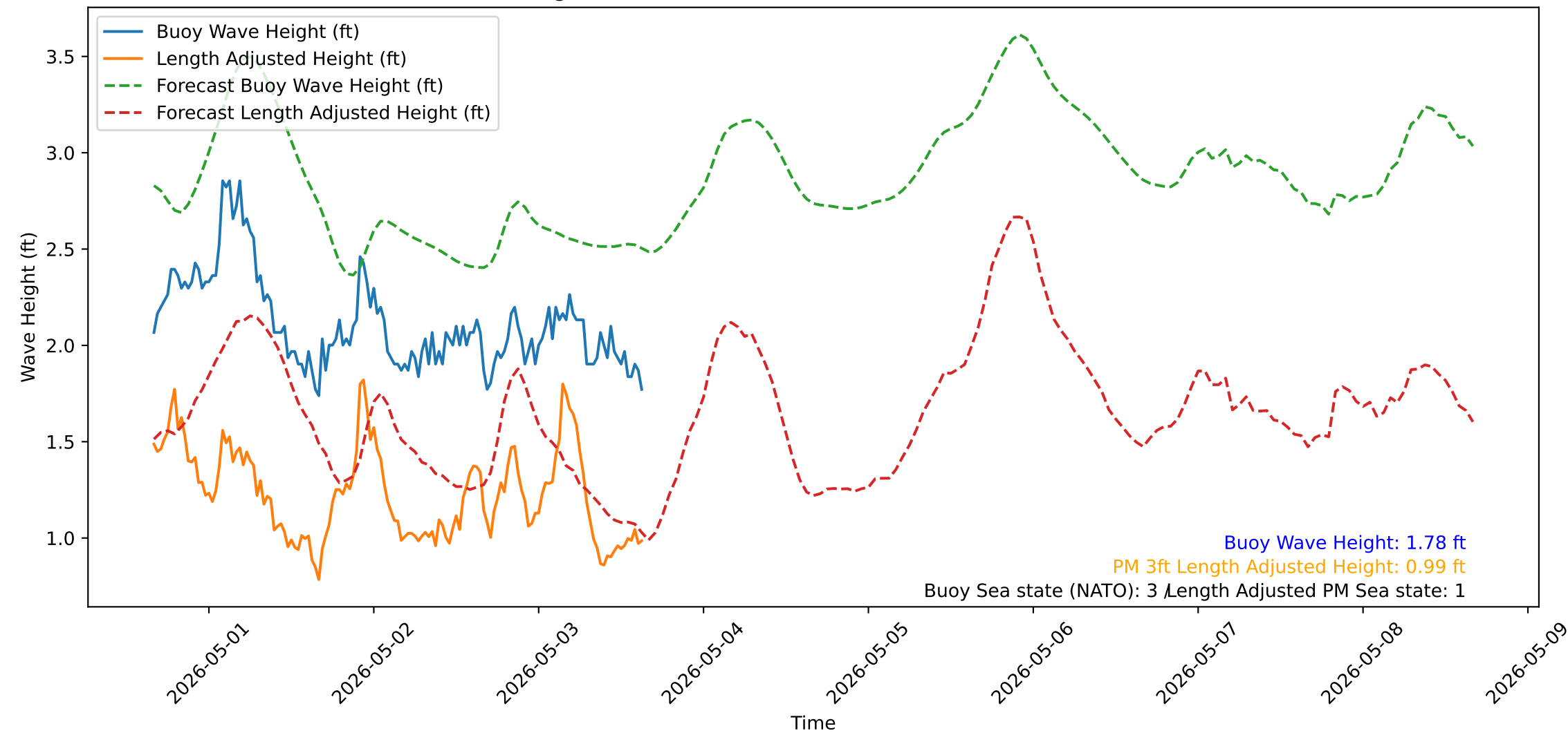
Wave Heights over Time for Green Beach at 2026-05-03 16:01:13
