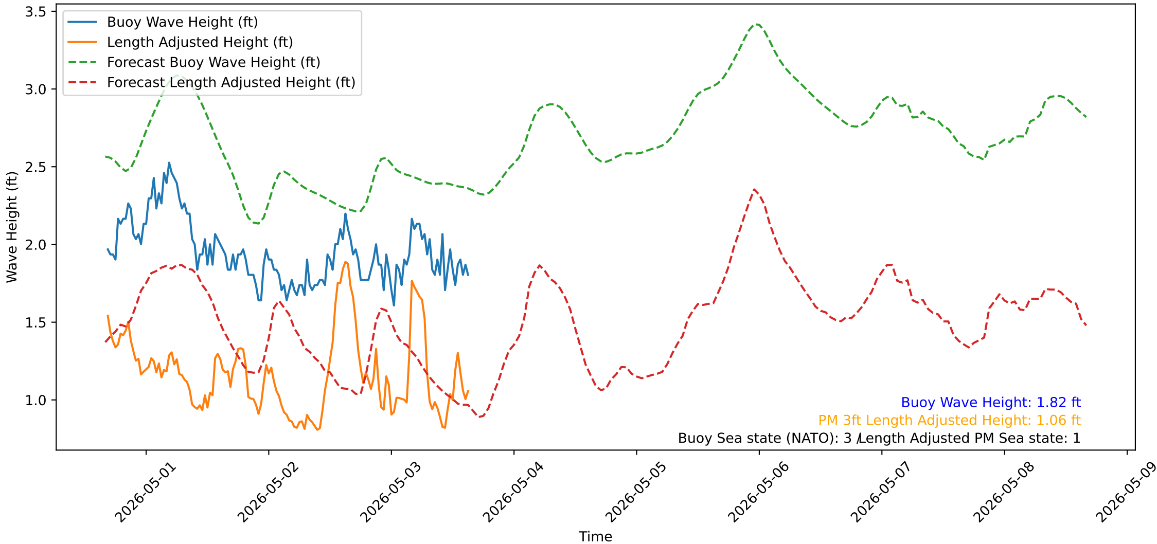
Wave Heights over Time for Red Beach at 2026-05-03 16:00:50
