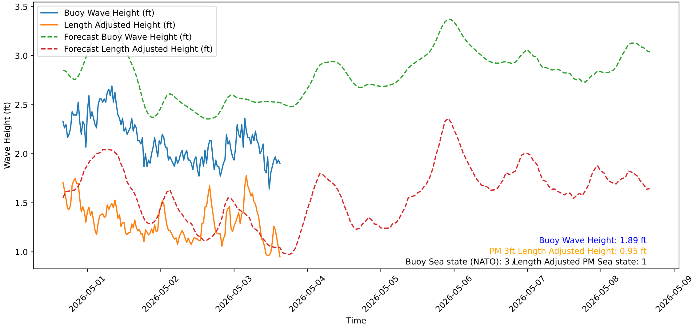
Wave Heights over Time for Oceanside Harbor at 2026-05-03 16:00:31
