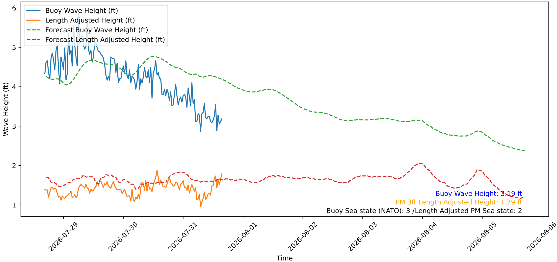
Wave Heights over Time for Oceanside Harbor at 2026-07-31 16:30:26
