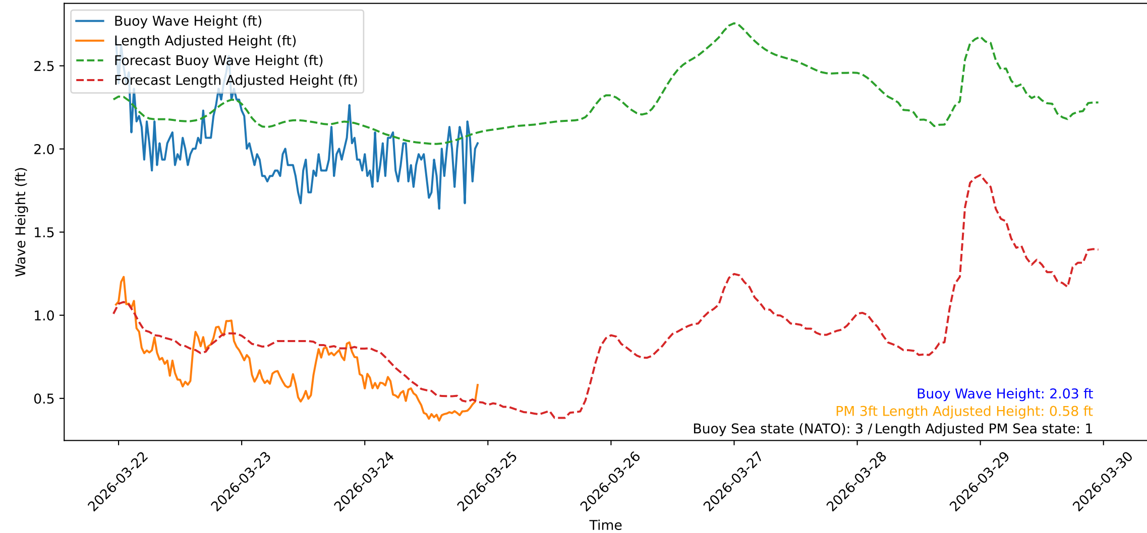
Wave Heights over Time for Red Beach at 2026-03-24 23:00:48
