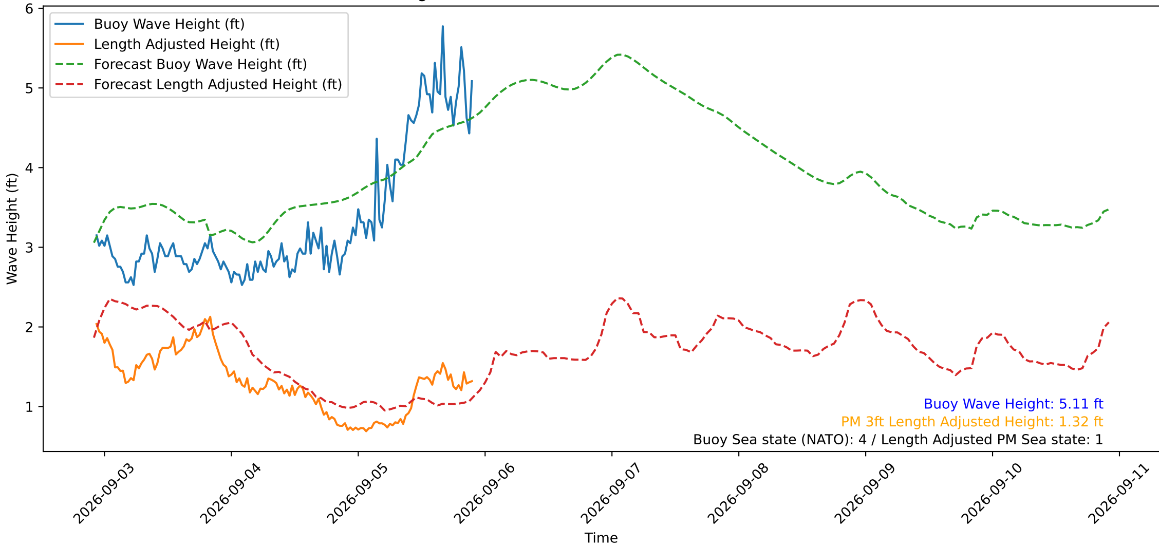
Wave Heights over Time for Red Beach at 2026-09-05 22:10:50
