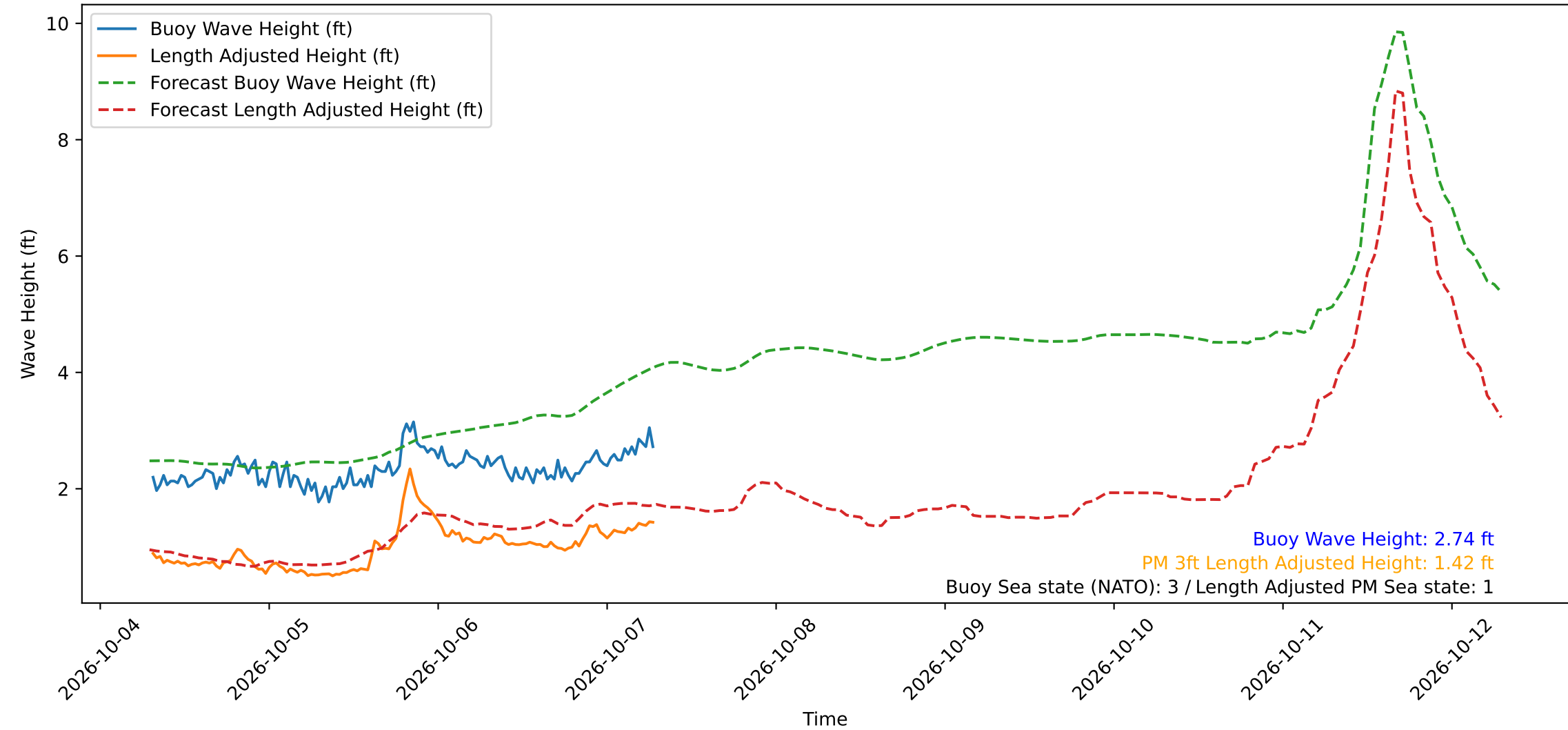
Wave Heights over Time for Green Beach at 2026-10-07 07:21:14
