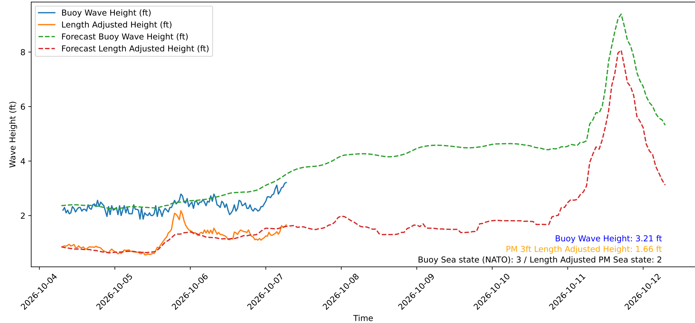
Wave Heights over Time for Oceanside Harbor at 2026-10-07 07:20:30
