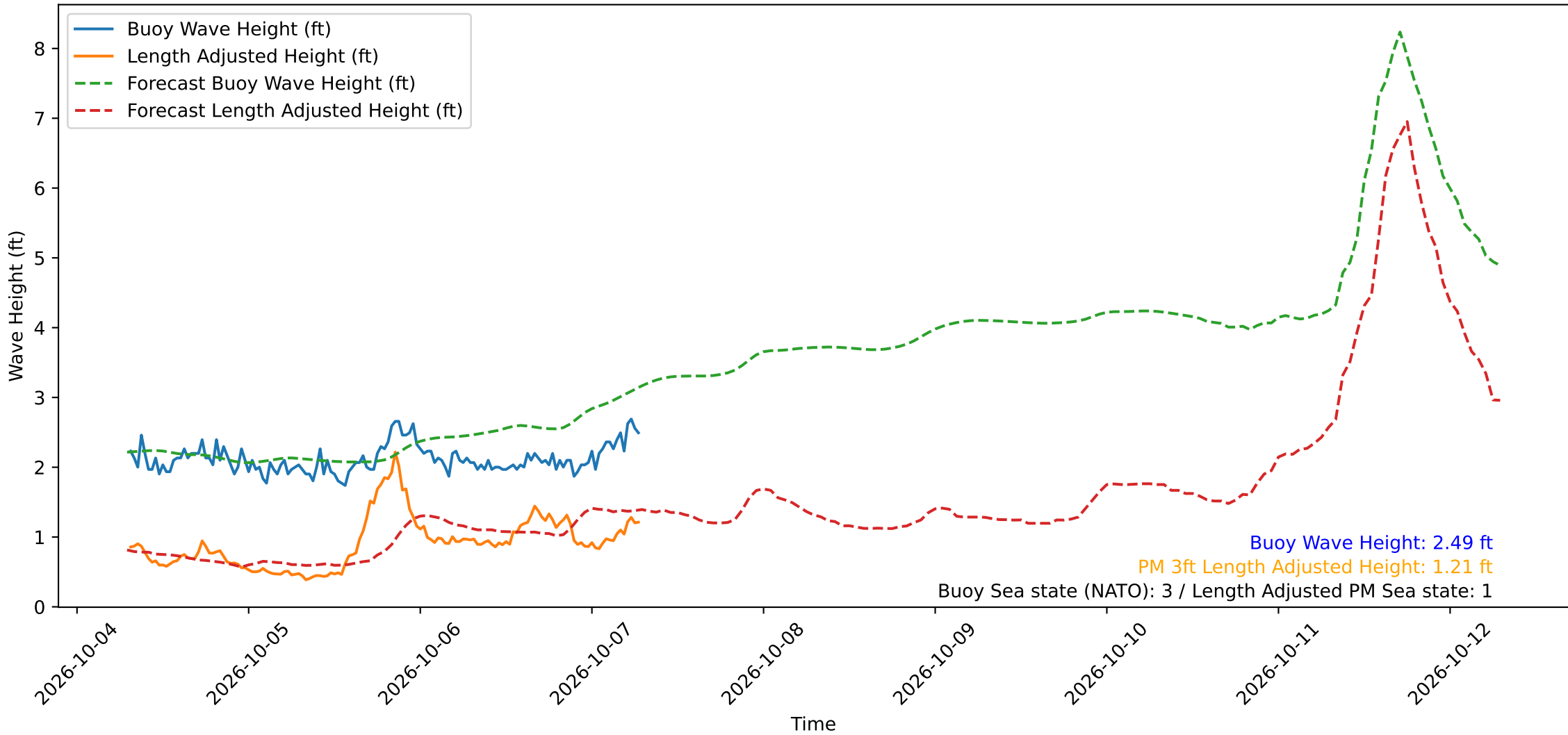
Wave Heights over Time for Red Beach at 2026-10-07 07:20:50
