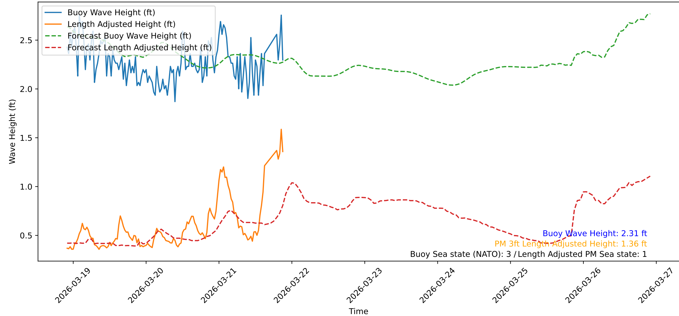
Wave Heights over Time for Red Beach at 2026-03-21 21:40:47
