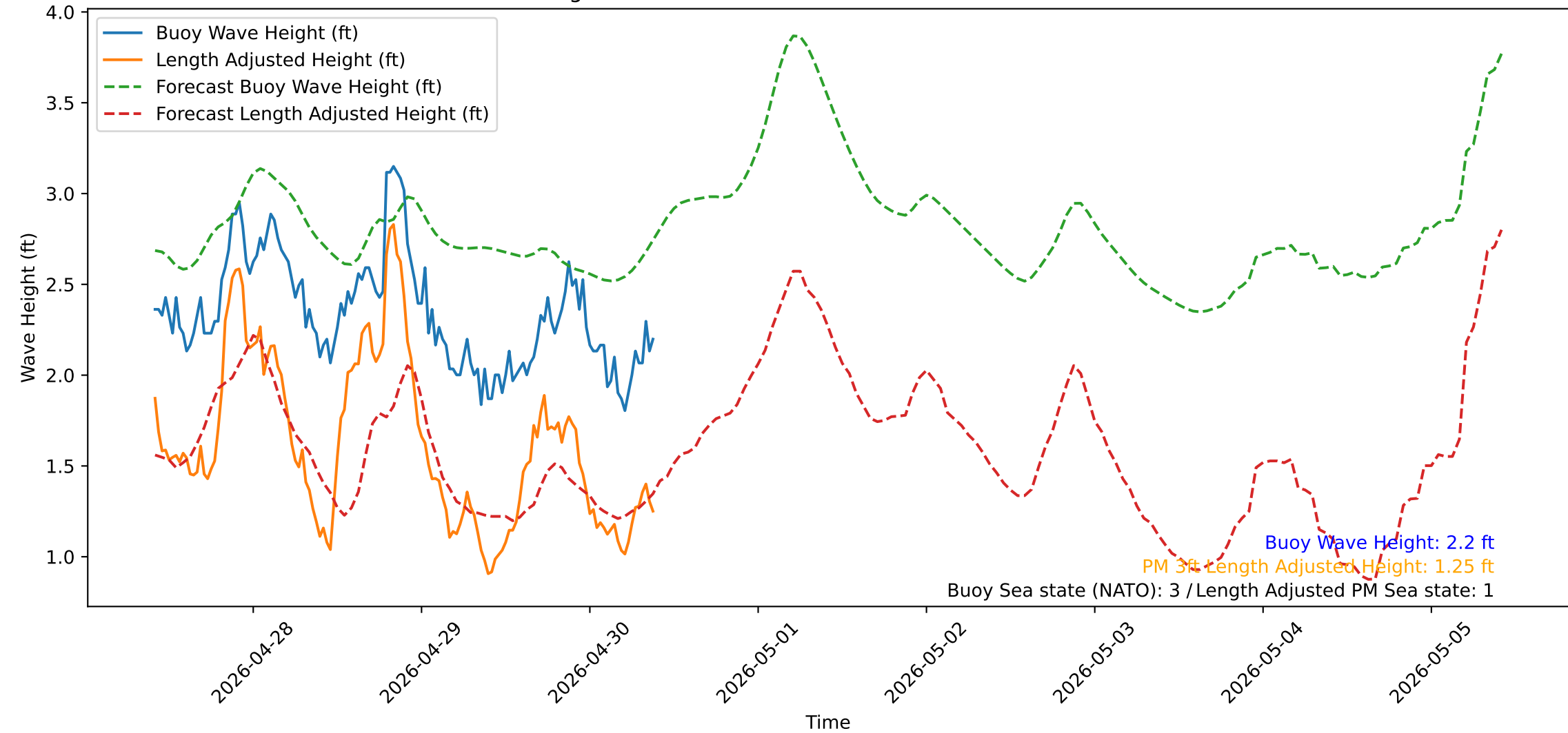
Wave Heights over Time for Green Beach at 2026-04-30 09:51:14
