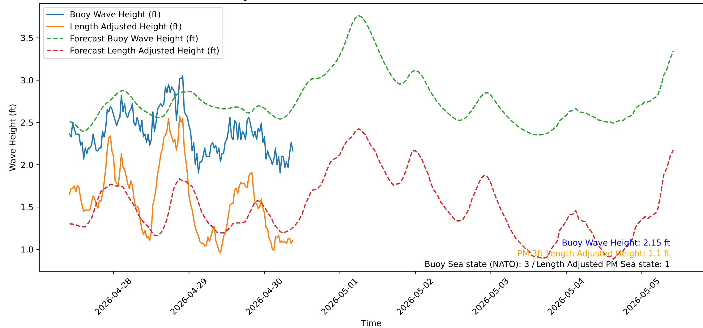
Wave Heights over Time for Oceanside Harbor at 2026-04-30 09:50:31
