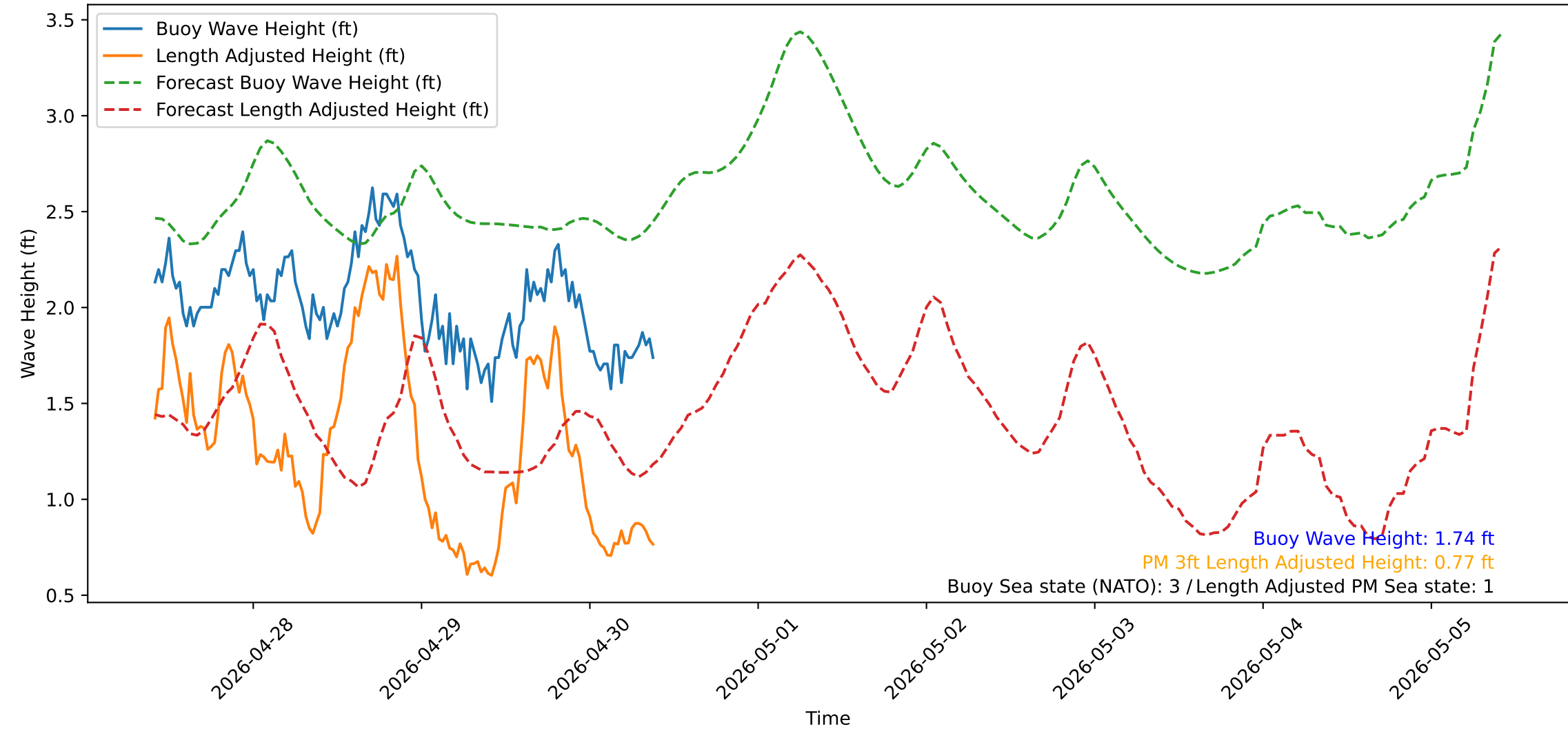
Wave Heights over Time for Red Beach at 2026-04-30 09:50:51
