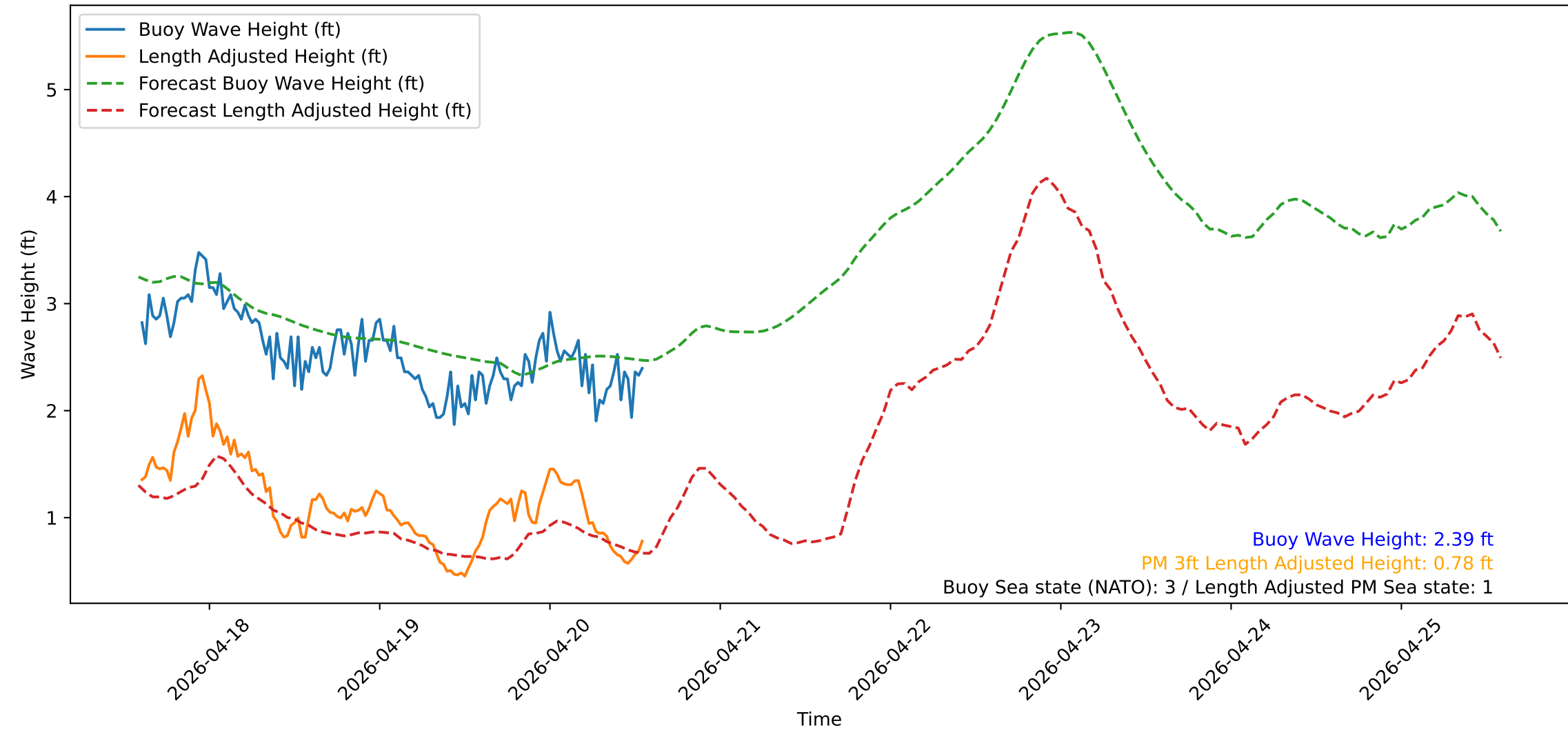
Wave Heights over Time for Green Beach at 2026-04-20 14:21:15
