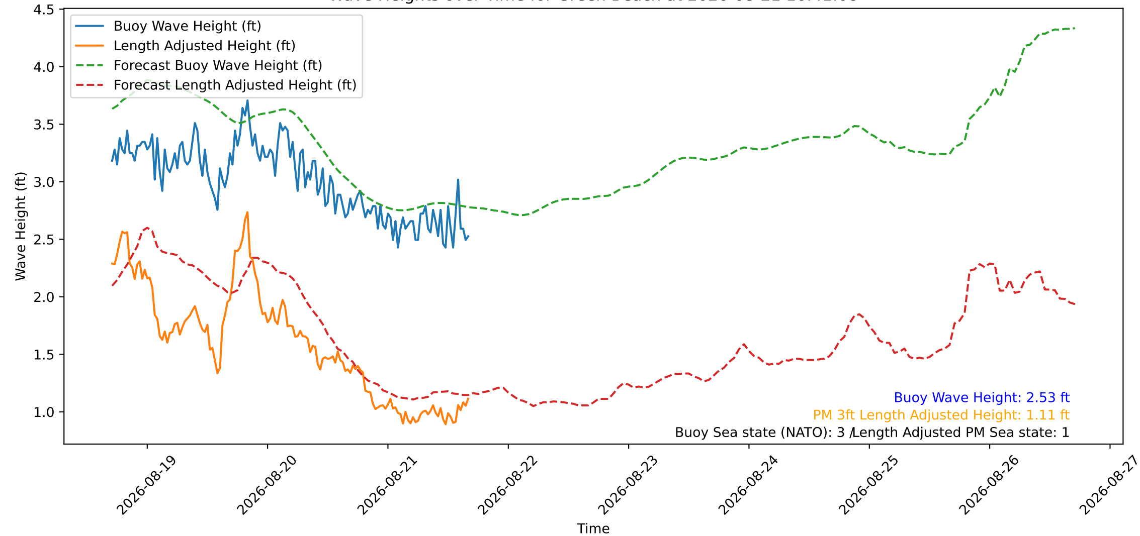
Wave Heights over Time for Green Beach at 2026-08-21 16:41:08
