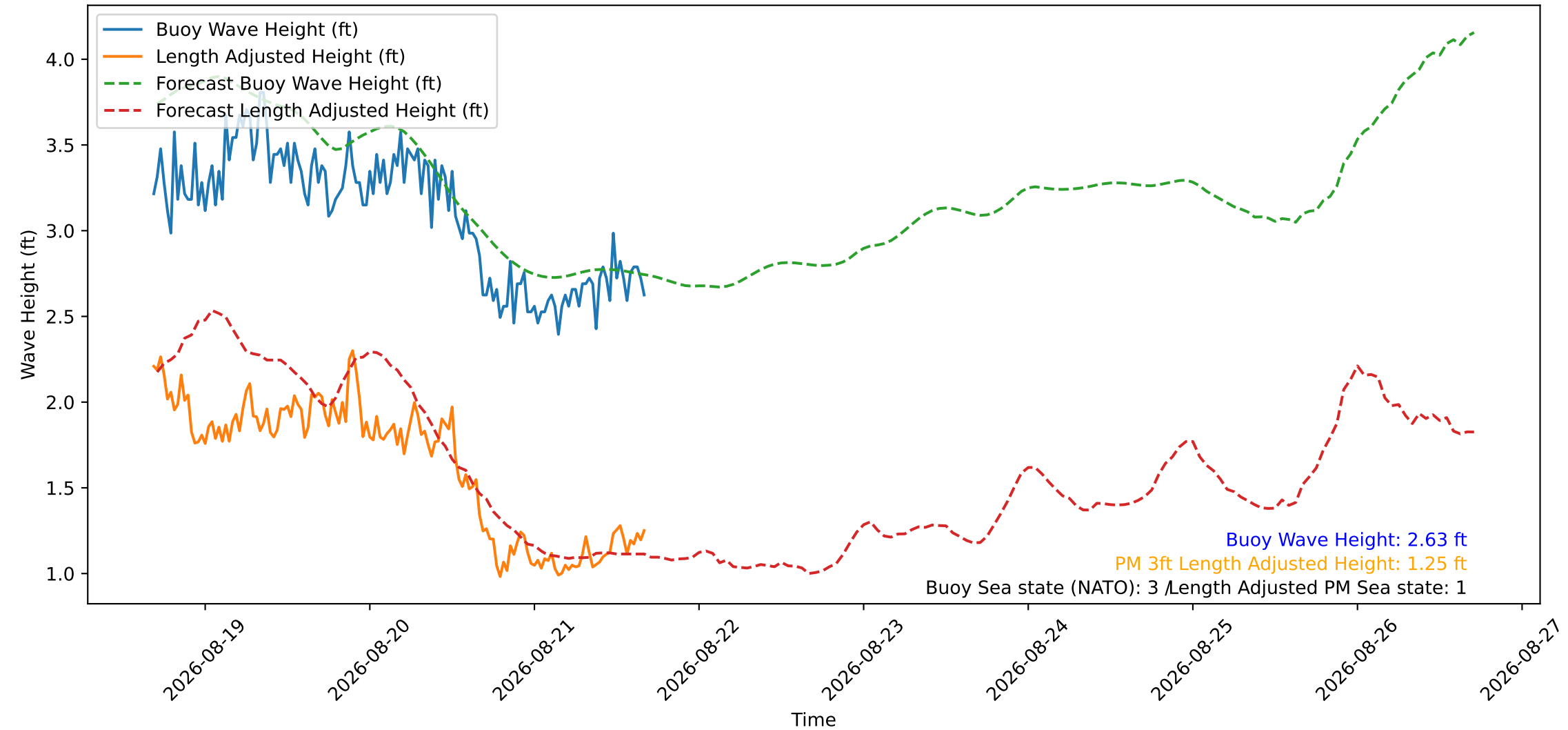
Wave Heights over Time for Oceanside Harbor at 2026-08-21 16:40:27
