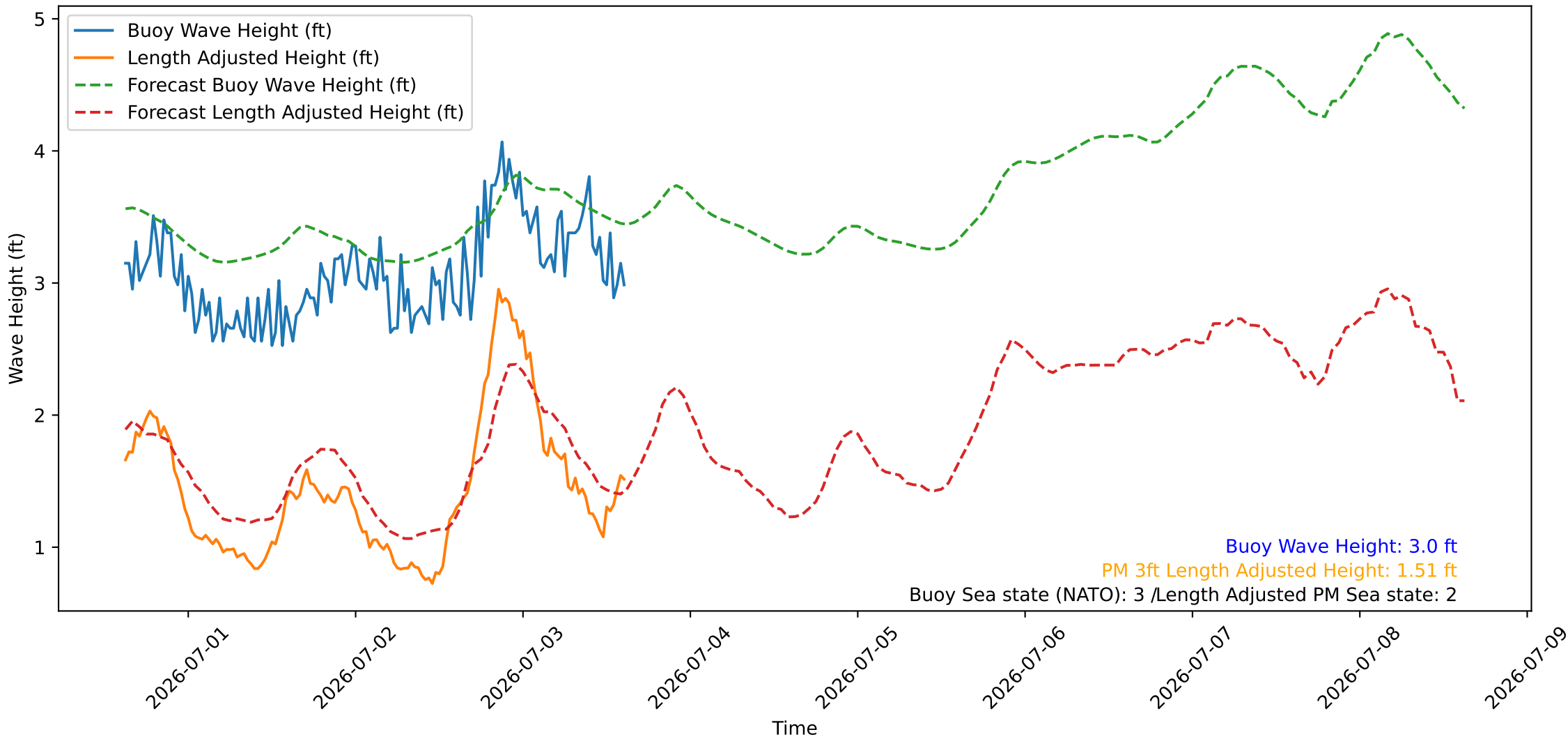
Wave Heights over Time for Green Beach at 2026-07-03 15:11:09
