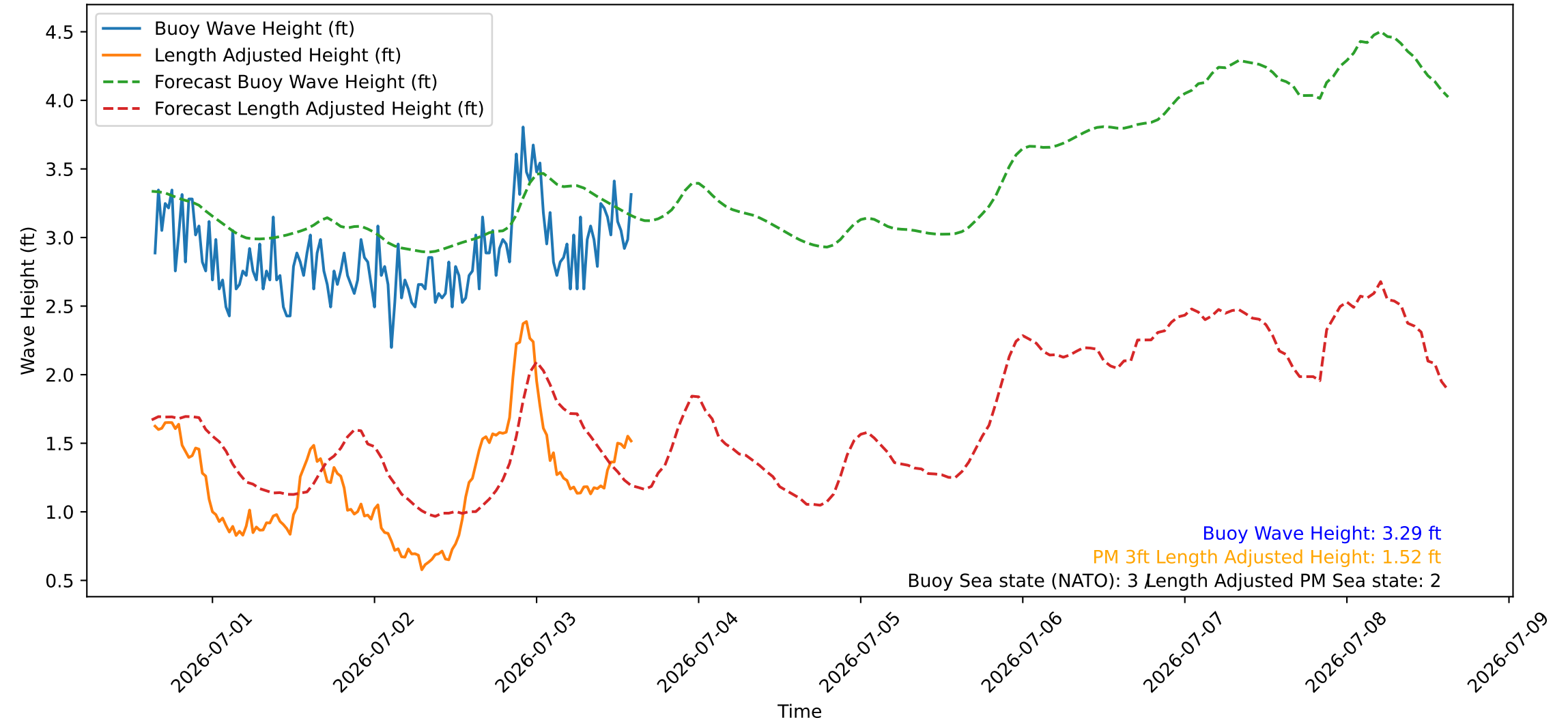
Wave Heights over Time for Red Beach at 2026-07-03 15:10:46
