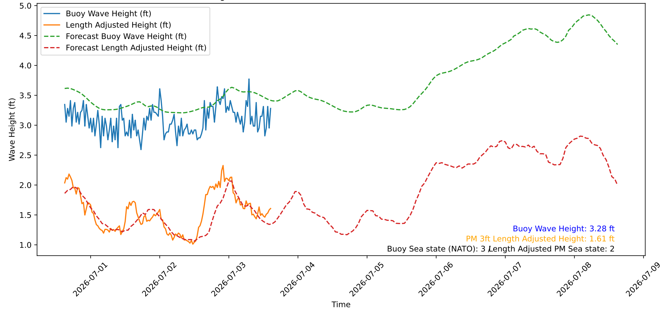
Wave Heights over Time for Oceanside Harbor at 2026-07-03 15:10:26
