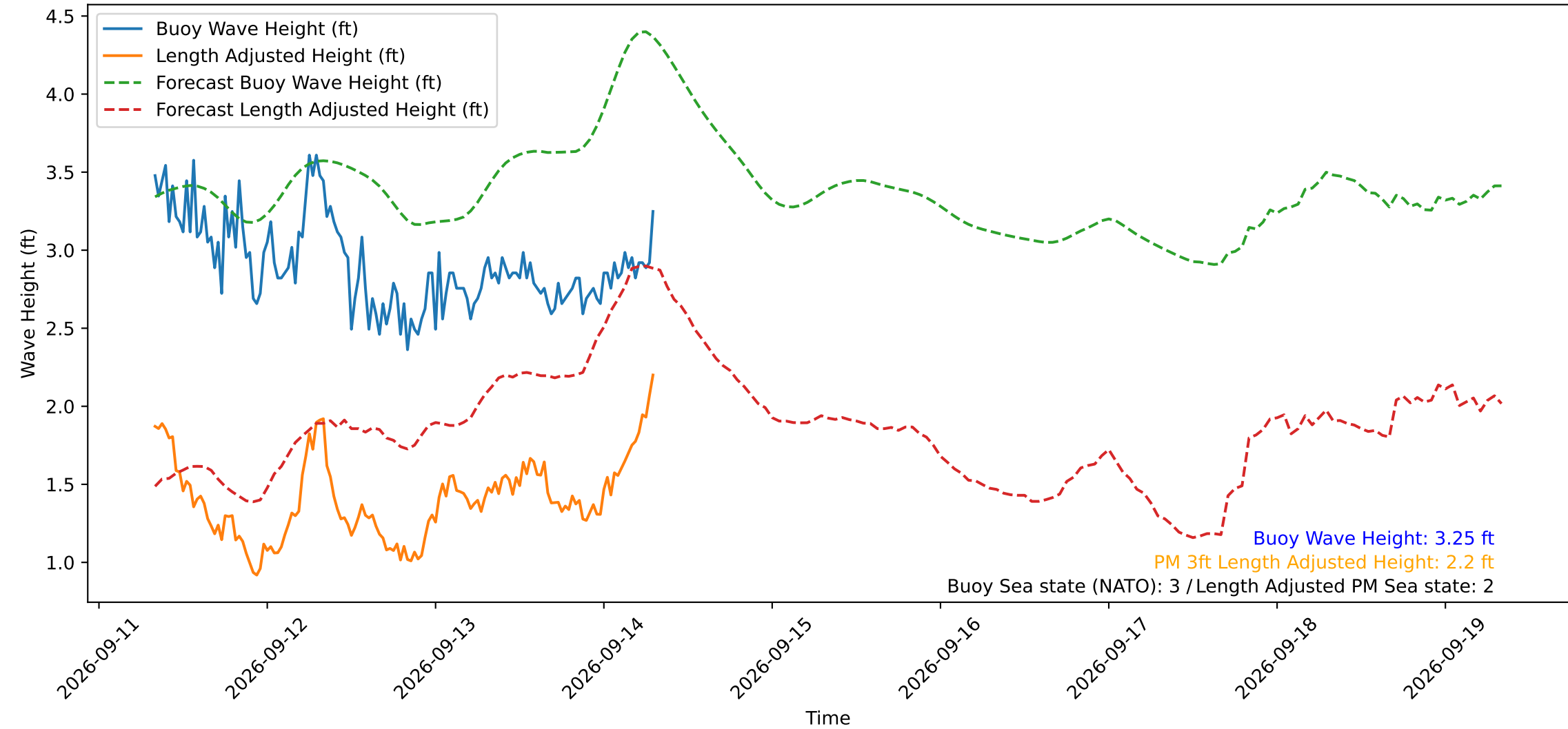
Wave Heights over Time for Green Beach at 2026-09-14 07:51:14
